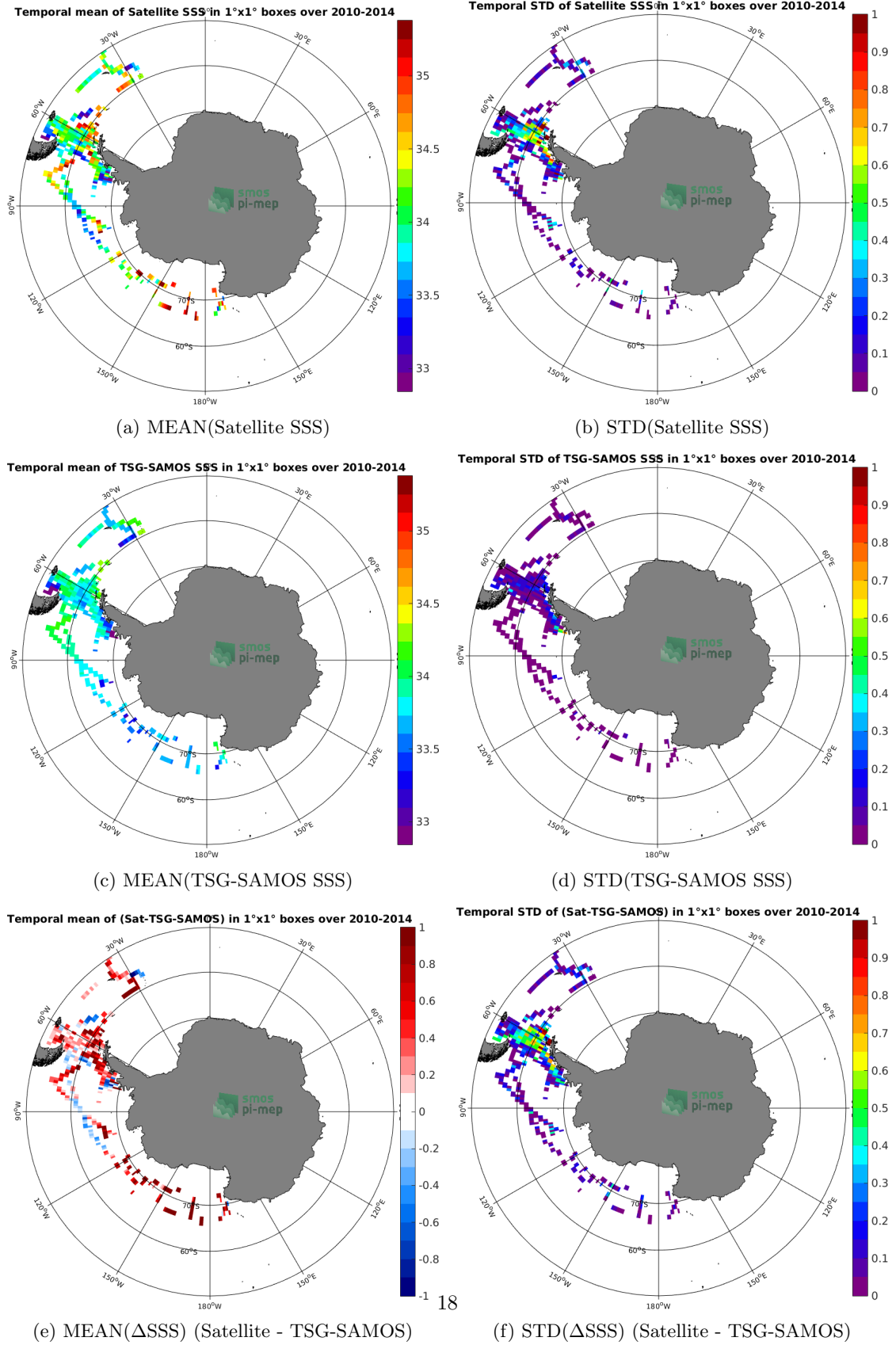
Figure 6: Temporal mean (left) and STD (right) of SSS from SMOS-L3-CATDS-CECOS-LOCEAN-V3-9DAYS-25KM (top), TSG-SAMOS (middle), and of \Delta SSS (Satellite - TSG-SAMOS). Only match-up pairs are used to generate these maps.
