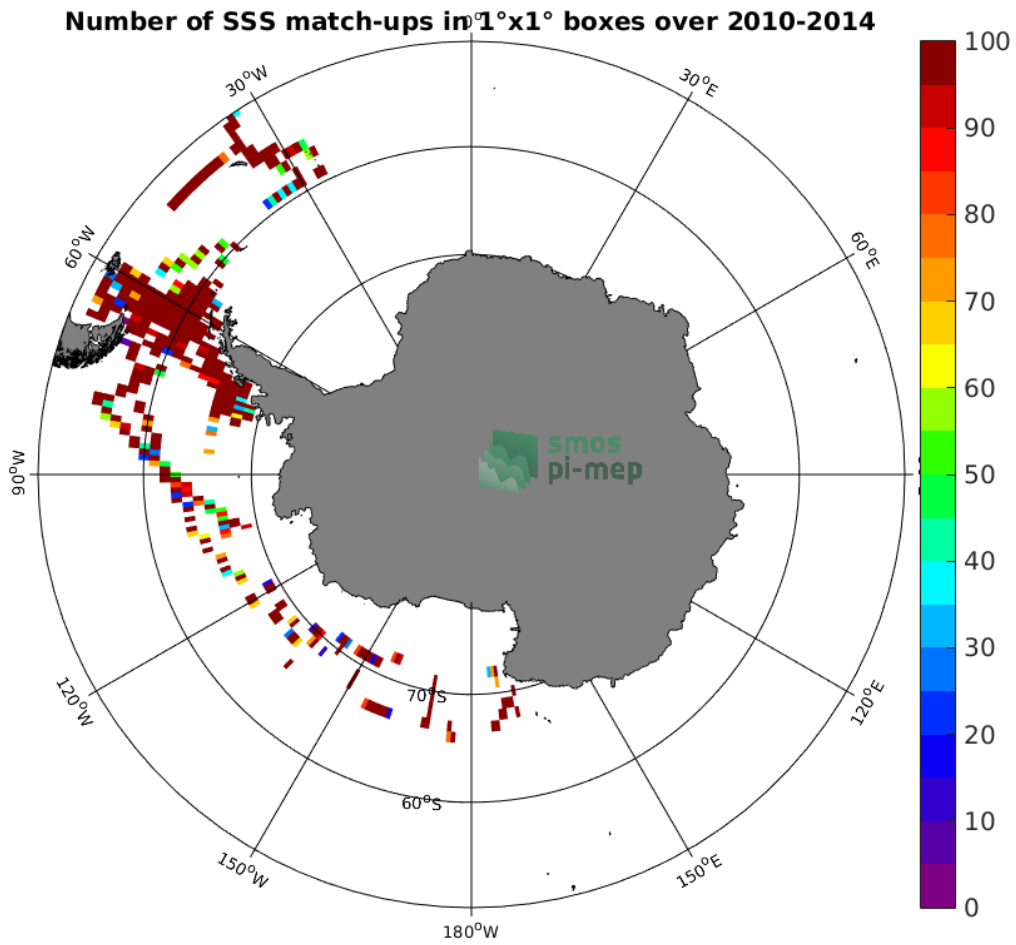
Figure 4: Number of SSS match-ups between TSG-SAMOS SSS and the SMOS-L3-CATDS-CECOS-LOCEAN-V3-9DAYS-25KM SSS product for the Southern Ocean Pi-MEP region over 1°x1° boxes and for the full satellite product period.
