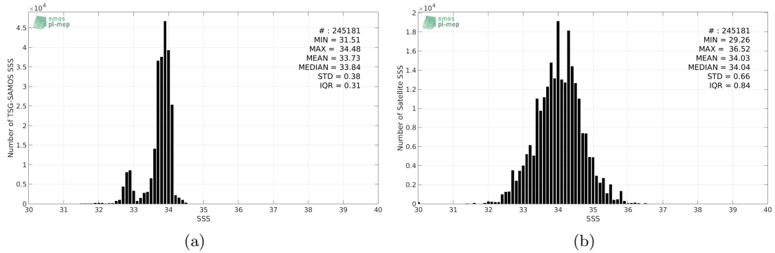
Figure 2: Histograms of SSS from TSG-SAMOS (a) and SMOS-L3-CATDS-CECOS-LOCEAN-V3-9DAYS-25KM (b) considering all match-up pairs per bins of 0.1 over the Southern Ocean Pi-MEP region and for the full satellite product period.
