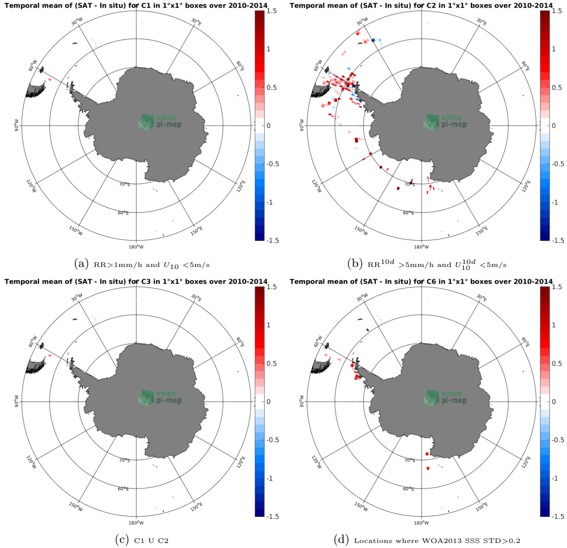
Figure 12: Temporal mean gridded over spatial boxes of size 1^\circ \times 1^\circ of \Delta SSS (SMOS-L3-CATDS-CECOS-LOCEAN-V3-9DAYS-25KM - TSG-SAMOS) for 4 different subdatasets corresponding to: RR > 1mm/h and U_{10} < 5\text{m/s} (a), RR^{10d} > 5\text{mm/h} and U_{10}^{10d} < 5\text{m/s} (b), C1 U C2 (c), Locations where WOA2013 SSS STD > 0.2 (d).
