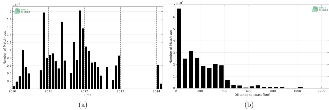
Figure 1: Number of match-ups between TSG-SAMOS and SMOS-L3-CATDS-CECOS-LOCEAN-V3-9DAYS-25KM SSS as a function of time (a) and as function of the distance to coast (b) over the Southern Ocean Pi-MEP region and for the full satellite product period.
