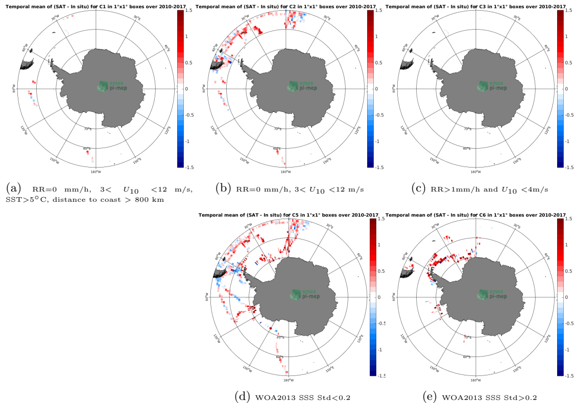
Figure 12: Temporal mean gridded over spatial boxes of size 1^\circ \times 1^\circ of \Delta SSS (SMOS-L3-CATDS-CECOS-LOCEAN-V3-9DAYS-25KM - TSG-POLARSTERN) for 5 different subdatasets corresponding to:RR=0 mm/h, 3 < U_{10} < 12 m/s, SST >5^\circ C, distance to coast > 800 km (a), RR=0 mm/h, 3 < U_{10} < 12 m/s (b), RR >1 mm/h and U_{10} < 4 m/s (c), WOA2013 SSS Std <0.2 (d), WOA2013 SSS Std >0.2 (e).
