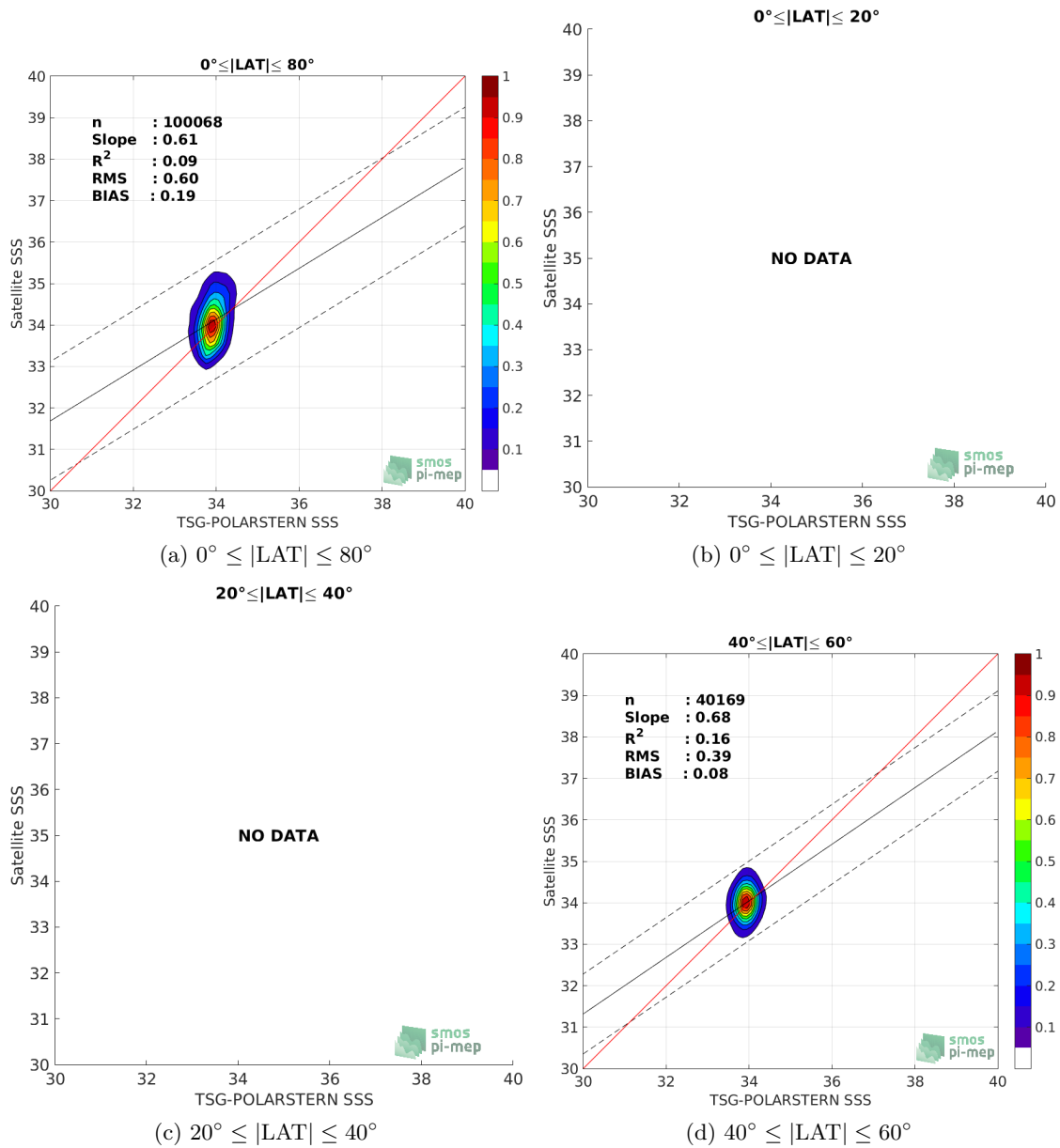
Figure 9: Contour maps of the concentration of SMOS-L3-CATDS-CECOS-LOCEAN-V3-9DAYS-25KM SSS (y-axis) versus TSG-POLARSTERN SSS (x-axis) at match-up pairs for different latitude bands. For each plot, the red line shows x=y . The black thin and dashed lines indicate a linear fit through the data cloud and the \pm 95\% confidence levels, respectively. The number match-up pairs n , the slope and R^2 coefficient of the linear fit, the root mean square (RMS) and the mean bias between satellite and in situ data are indicated for each latitude band in each plots.
