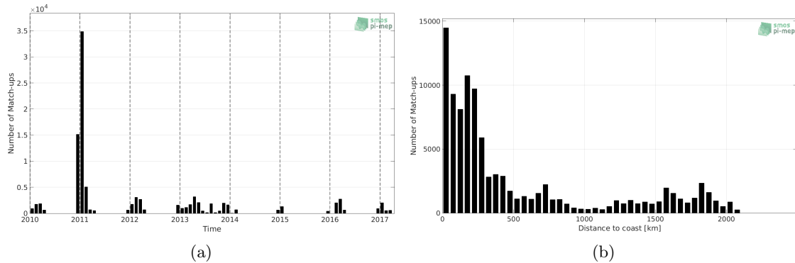
Figure 1: Number of match-ups between TSG-POLARSTERN and SMOS-L3-CATDS-CECOS-LOCEAN-V3-9DAYS-25KM SSS as a function of time (a) and as function of the distance to coast (b) over the Southern Ocean Pi-MEP region and for the full satellite product period.
