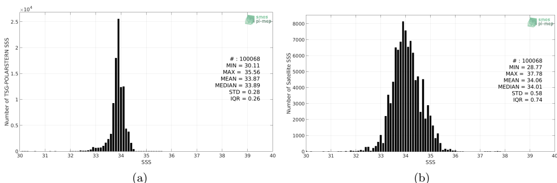
Figure 2: Histograms of SSS from TSG-POLARSTERN (a) and SMOS-L3-CATDS-CECOS-LOCEAN-V3-9DAYS-25KM (b) considering all match-up pairs per bins of 0.1 over the Southern Ocean Pi-MEP region and for the full satellite product period.
