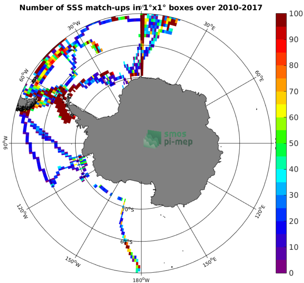
Figure 4: Number of SSS match-ups between TSG-POLARSTERN SSS and the SMOS-L3-CATDS-CECOS-LOCEAN-V3-9DAYS-25KM SSS product for the Southern Ocean Pi-MEP region over 1^\circ \times 1^\circ boxes and for the full satellite product period.
