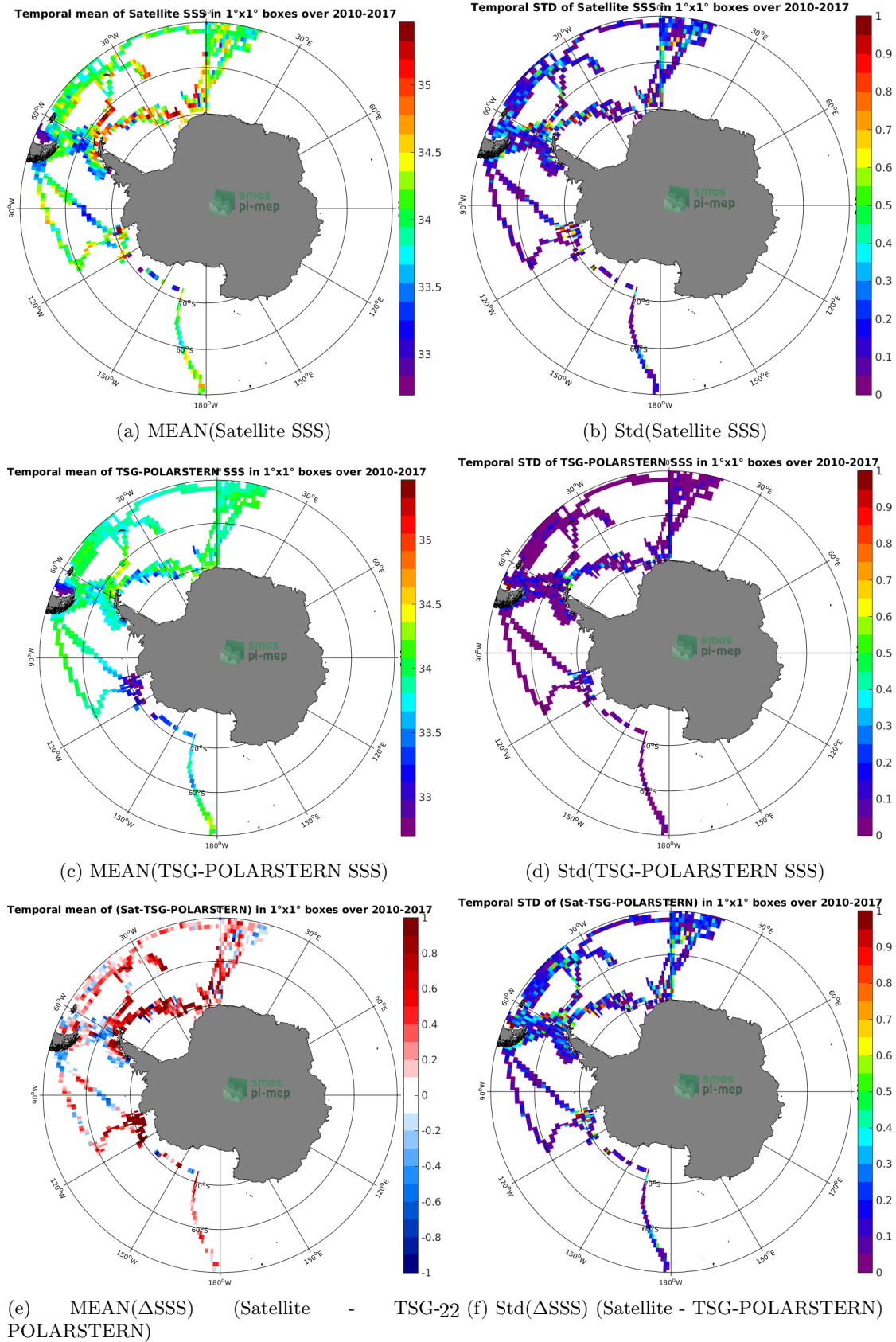
Figure 6: Temporal mean (left) and Std (right) of SSS from SMOS-L3-CATDS-CECOS-LOCEAN-V3-9DAYS-25KM (top), TSG-POLARSTERN (middle), and of \Delta SSS (Satellite - TSG-POLARSTERN). Only match-up pairs are used to generate these maps.
