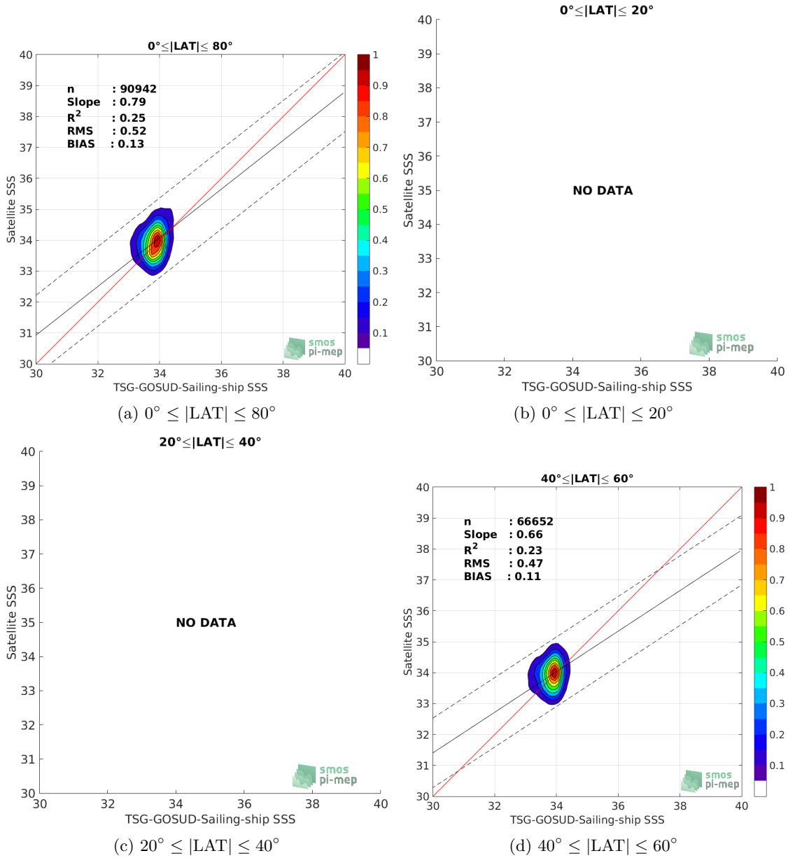
Figure 9: Contour maps of the concentration of SMOS-L3-CATDS-CECOS-LOCEAN-V3-9DAYS-25KM SSS (y-axis) versus TSG-GOSUD-Sailing-ship SSS (x-axis) at match-up pairs for different latitude bands. For each plot, the red line shows x=y . The black thin and dashed lines indicate a linear fit through the data cloud and the \pm 95\% confidence levels, respectively. The number match-up pairs n , the slope and R^2 coefficient of the linear fit, the root mean square (RMS) and the mean bias between satellite and in situ data are indicated for each latitude band in each plots.
