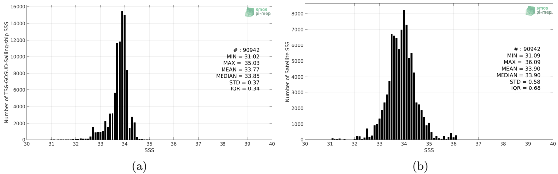
Figure 2: Histograms of SSS from TSG-GOSUD-Sailing-ship (a) and SMOS-L3-CATDS-CECOS-LOCEAN-V3-9DAYS-25KM (b) considering all match-up pairs per bins of 0.1 over the Southern Ocean Pi-MEP region and for the full satellite product period.
