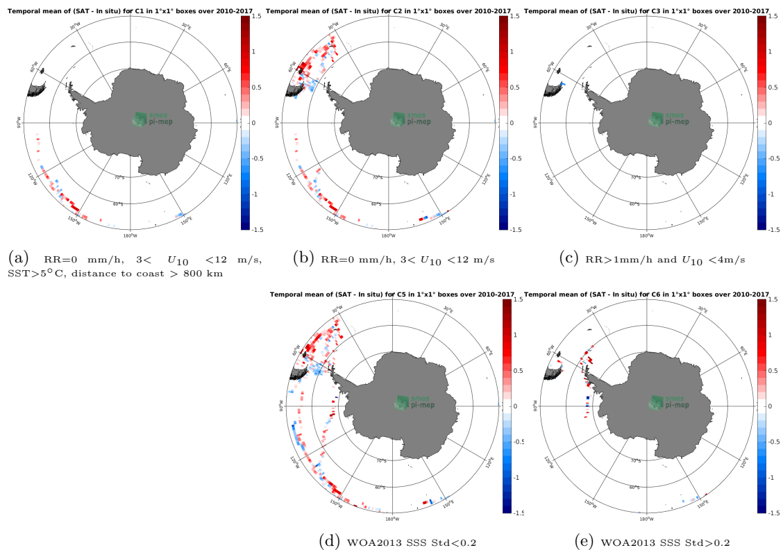
Figure 12: Temporal mean gridded over spatial boxes of size 1^\circ \times 1^\circ of \Delta SSS (SMOS-L3-CATDS-CECOS-LOCEAN-V3-9DAYS-25KM - TSG-GOSUD-Sailing-ship) for 5 different subdatasets corresponding to: RR=0 mm/h, 3 < U_{10} < 12 m/s, SST > 5^\circ\text{C} , distance to coast > 800 km (a), RR=0 mm/h, 3 < U_{10} < 12 m/s (b), RR > 1 mm/h and U_{10} < 4 m/s (c), WOA2013 SSS Std < 0.2 (d), WOA2013 SSS Std > 0.2 (e).
