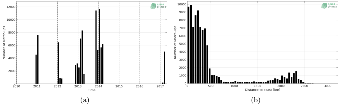
Figure 1: Number of match-ups between TSG-GOSUD-Sailing-ship and SMOS-L3-CATDS-CECOS-LOCEAN-V3-9DAYS-25KM SSS as a function of time (a) and as function of the distance to coast (b) over the Southern Ocean Pi-MEP region and for the full satellite product period.
