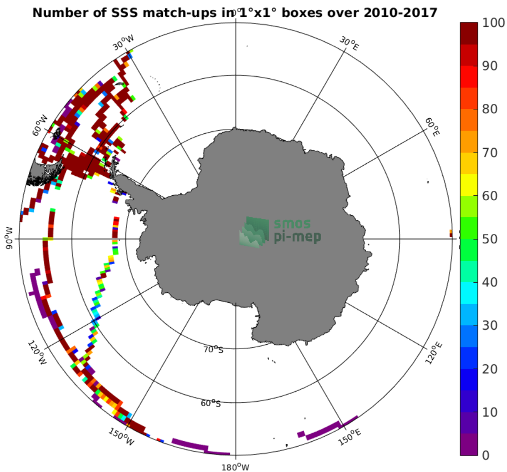
Figure 4: Number of SSS match-ups between TSG-GOSUD-Sailing-ship SSS and the SMOS-L3-CATDS-CECOS-LOCEAN-V3-9DAYS-25KM SSS product for the Southern Ocean Pi-MEP region over 1^\circ \times 1^\circ boxes and for the full satellite product period.
