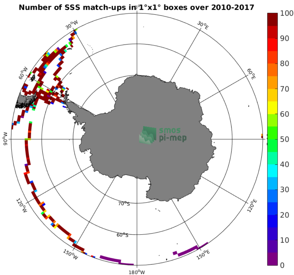
Figure 4: Number of SSS match-ups between TSG-GOSUD-Sailing-ship SSS and the SMOS-L3-CATDS-CECOS-LOCEAN-V3-9DAYS-25KM SSS product for the Southern Ocean Pi-MEP region over 1°x1° boxes and for the full satellite product period.
