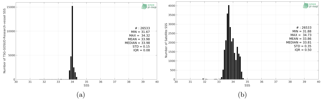
Figure 2: Histograms of SSS from TSG-GOSUD-Research-vessel (a) and SMOS-L3-CATDS-CECOS-LOCEAN-V3-9DAYS-25KM (b) considering all match-up pairs per bins of 0.1 over the Southern Ocean Pi-MEP region and for the full satellite product period.
