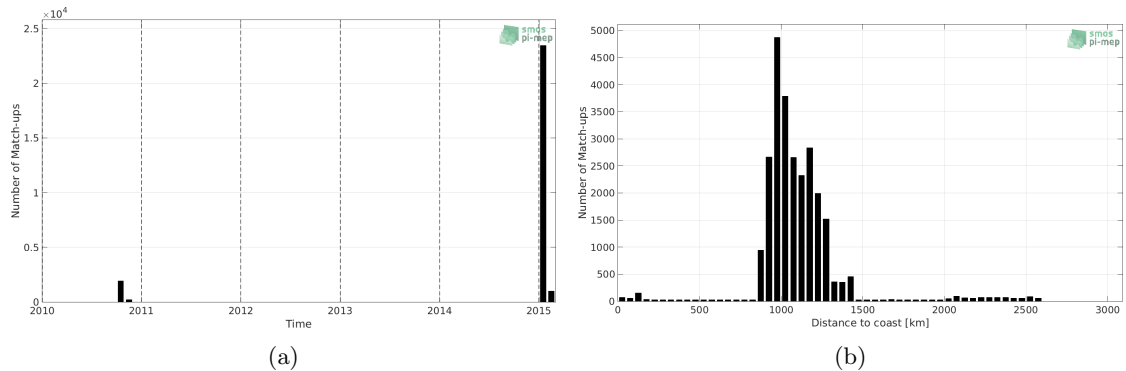
Figure 1: Number of match-ups between TSG-GOSUD-Research-vessel and SMOS-L3-CATDS-CECOS-LOCEAN-V3-9DAYS-25KM SSS as a function of time (a) and as function of the distance to coast (b) over the Southern Ocean Pi-MEP region and for the full satellite product period.
