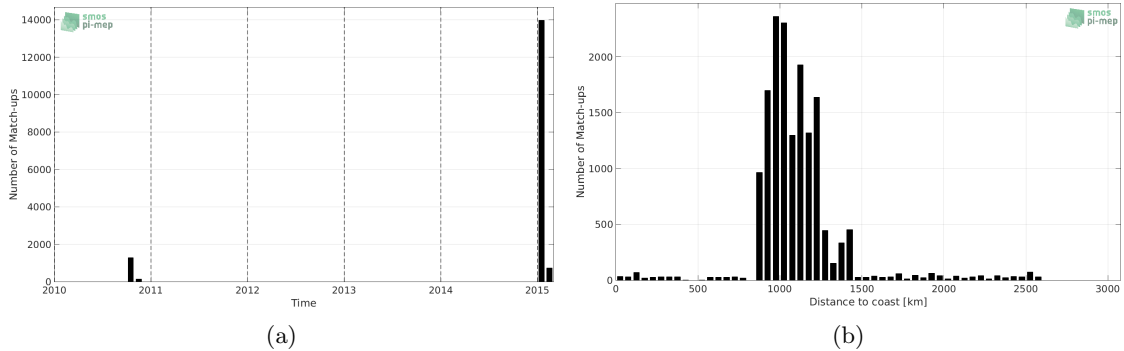
Figure 1: Number of match-ups between TSG-GOSUD-Research-vessel and SMOS-L3-CATDS-CECOS-LOCEAN-V3-9DAYS-25KM SSS as a function of time (a) and as function of the distance to coast (b) over the Southern Ocean Pi-MEP region and for the full satellite product period.
