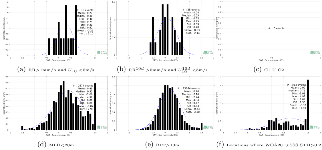
Figure 13: Normalized histogram of \Delta SSS (SMOS-L3-CATDS-CECOS-LOCEAN-V3-9DAYS-25KM - Sea mammals) for 6 different subdatasets corresponding to: RR>1mm/h and U_{10} < 5\text{m/s} (a), RR^{10d} > 5\text{mm/h} and U_{10}^{10d} < 5\text{m/s} (b), C1 U C2 (c),MLD<20m (d),BLT>10m (e),Locations where WOA2013 SSS STD>0.2 (f).
