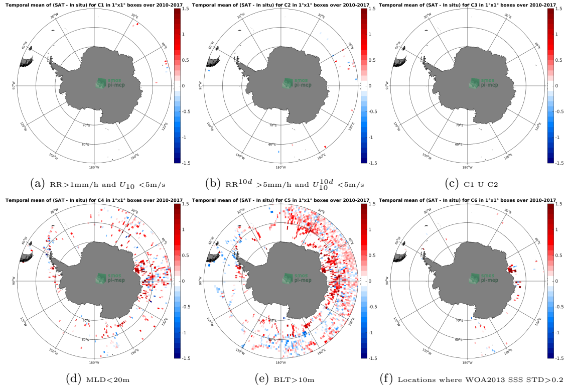
Figure 12: Temporal mean gridded over spatial boxes of size 1^\circ \times 1^\circ of \Delta\text{SSS} (SMOS-L3-CATDS-CECOS-LOCEAN-V3-9DAYS-25KM - Sea mammals) for 6 different subdatasets corresponding to: RR > 1\text{mm/h} and U_{10} < 5\text{m/s} (a), \text{RR}^{10d} > 5\text{mm/h} and U_{10}^{10d} < 5\text{m/s} (b), C1 U C2 (c), \text{MLD} < 20\text{m} (d), \text{BLT} > 10\text{m} (e), Locations where WOA2013 SSS STD > 0.2 (f).
