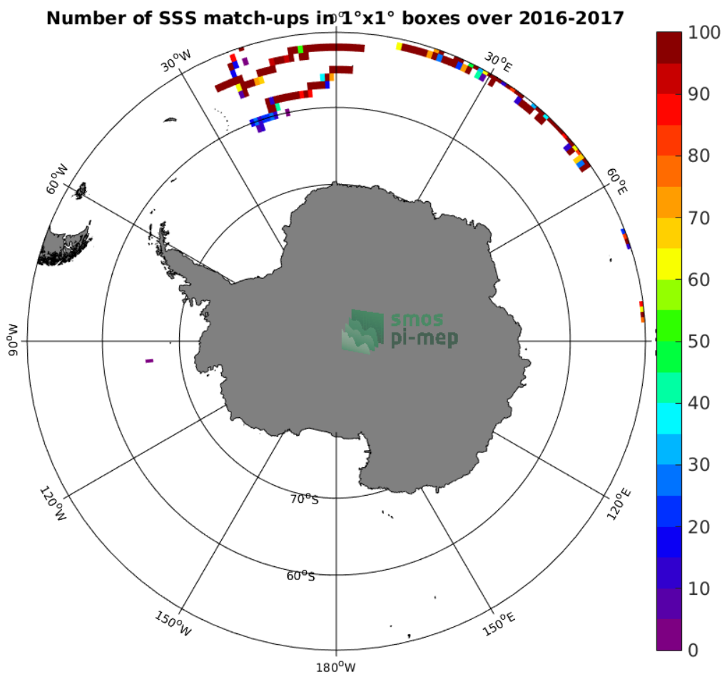
Figure 3: Number of SSS match-ups between Surface drifters SSS and the SMOS-L3-CATDS-CECOS-LOCEAN-V3-9DAYS-25KM SSS product for the Southern Ocean Pi-MEP region over 1^\circ \times 1^\circ boxes and for the full satellite product period.
