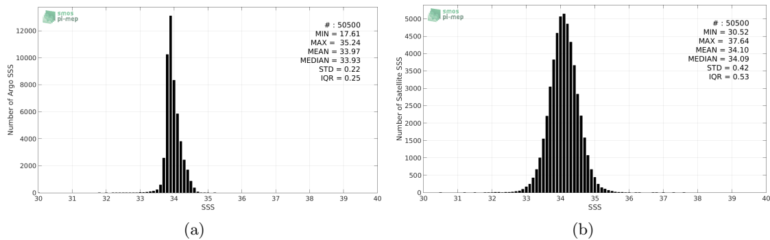
Figure 2: Histograms of SSS from Argo (a) and SMOS-L3-CATDS-CECOS-LOCEAN-V3-9DAYS-25KM (b) considering all match-up pairs per bins of 0.1 over the Southern Ocean Pi-MEP region and for the full satellite product period.
