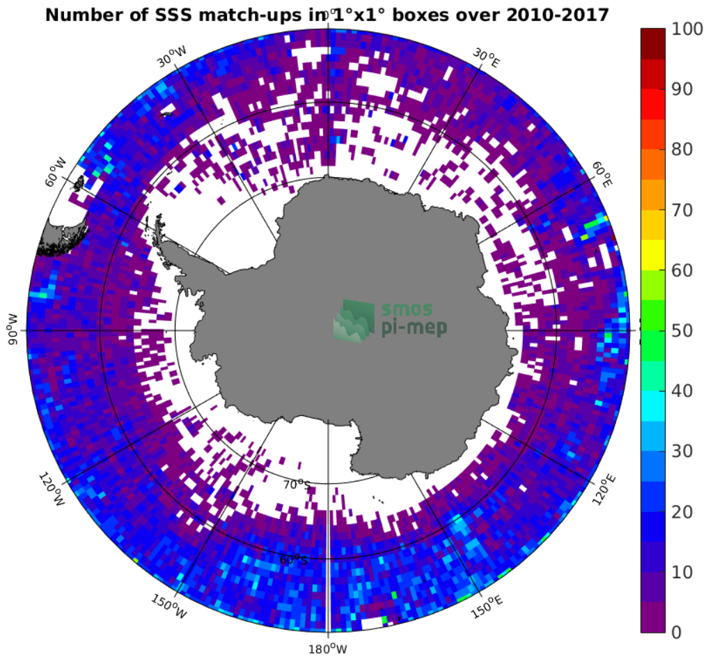
Figure 4: Number of SSS match-ups between Argo SSS and the SMOS-L3-CATDS-CECOS-LOCEAN-V3-9DAYS-25KM SSS product for the Southern Ocean Pi-MEP region over 1^\circ \times 1^\circ boxes and for the full satellite product period.
