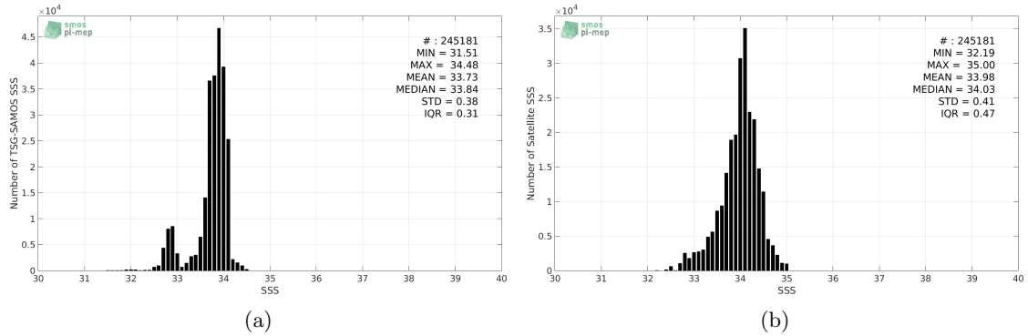
Figure 2: Histograms of SSS from TSG-SAMOS (a) and SMOS-L3-CATDS-CECOS-LOCEAN-V3-18DAYS-25KM (b) considering all match-up pairs per bins of 0.1 over the Southern Ocean Pi-MEP region and for the full satellite product period.
