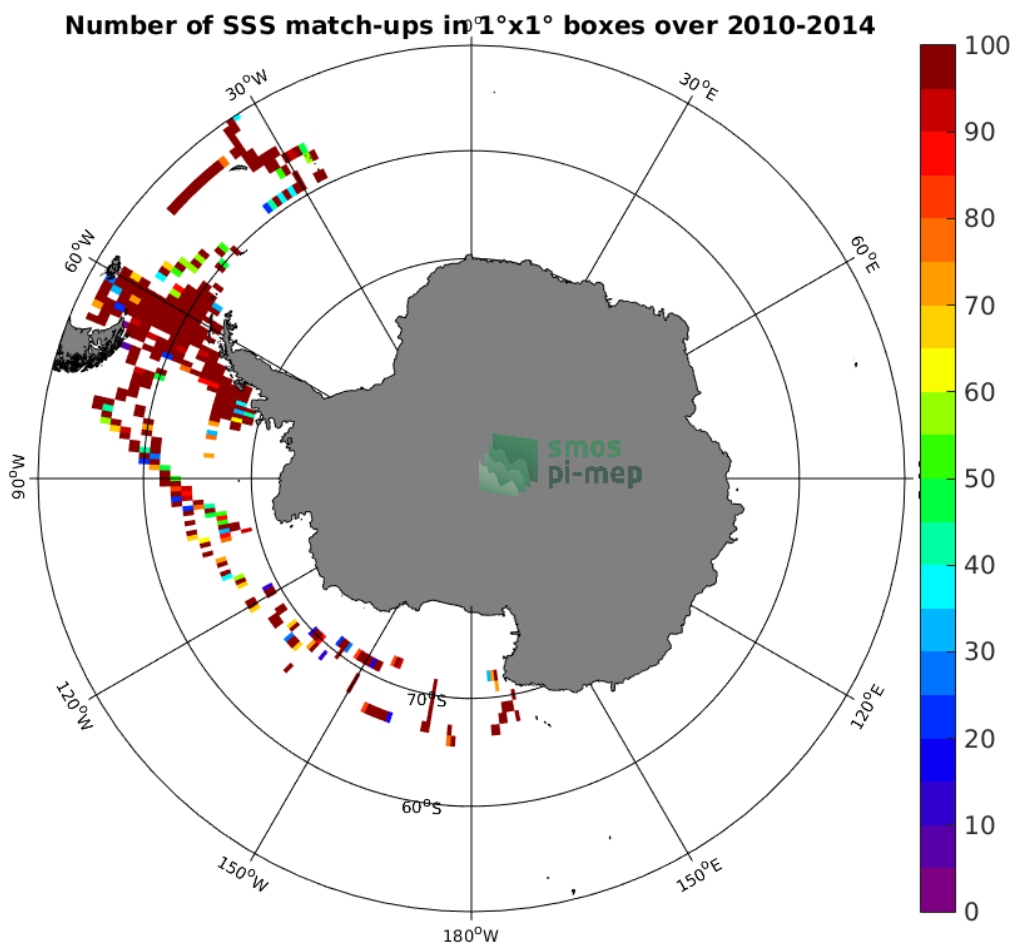
Figure 4: Number of SSS match-ups between TSG-SAMOS SSS and the SMOS-L3-CATDS-CECOS-LOCEAN-V3-18DAYS-25KM SSS product for the Southern Ocean Pi-MEP region over 1^\circ \times 1^\circ boxes and for the full satellite product period.
