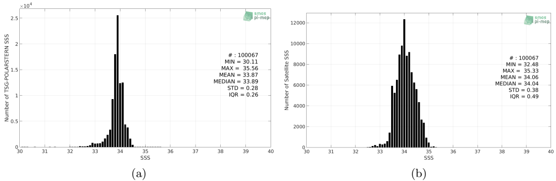
Figure 2: Histograms of SSS from TSG-POLARSTERN (a) and SMOS-L3-CATDS-CECOS-LOCEAN-V3-18DAYS-25KM (b) considering all match-up pairs per bins of 0.1 over the Southern Ocean Pi-MEP region and for the full satellite product period.
