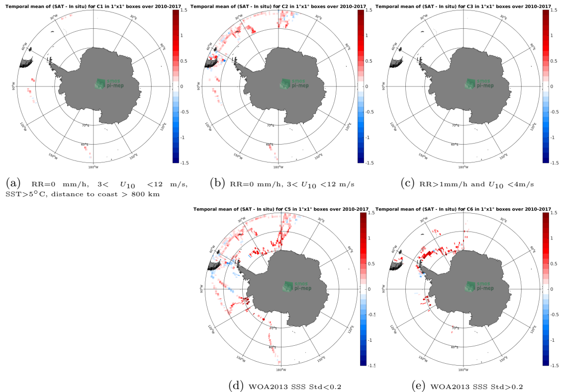
Figure 12: Temporal mean gridded over spatial boxes of size 1^\circ \times 1^\circ of \Delta SSS (SMOS-L3-CATDS-CECOS-LOCEAN-V3-18DAYS-25KM - TSG-POLARSTERN) for 5 different subdatasets corresponding to:RR=0 mm/h, 3 < U_{10} < 12 m/s, SST >5^\circ C, distance to coast > 800 km (a), RR=0 mm/h, 3 < U_{10} < 12 m/s (b), RR >1 mm/h and U_{10} < 4 m/s (c), WOA2013 SSS Std <0.2 (d), WOA2013 SSS Std >0.2 (e).
