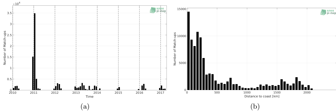
Figure 1: Number of match-ups between TSG-POLARSTERN and SMOS-L3-CATDS-CECOS-LOCEAN-V3-18DAYS-25KM SSS as a function of time (a) and as function of the distance to coast (b) over the Southern Ocean Pi-MEP region and for the full satellite product period.
