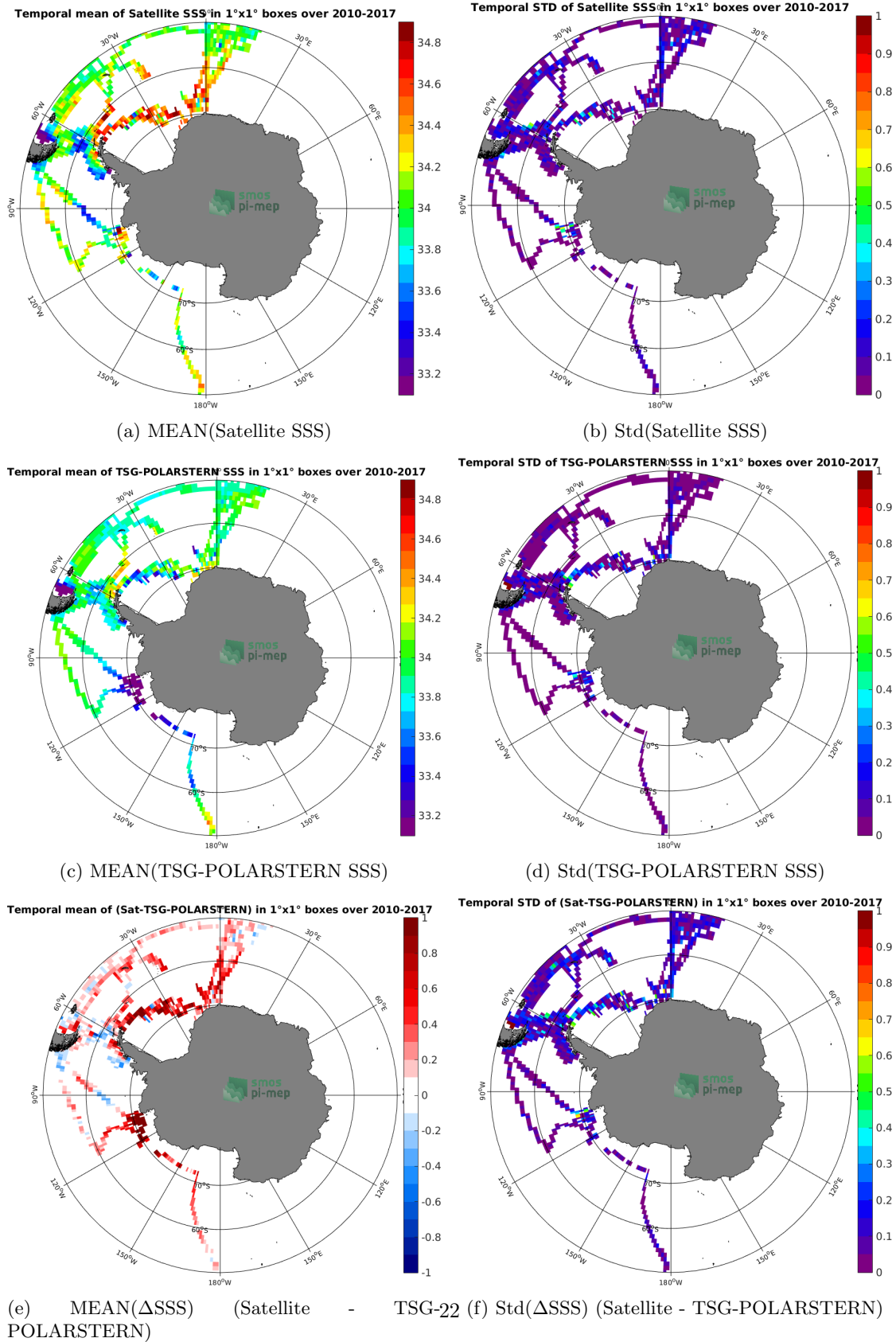
Figure 6: Temporal mean (left) and Std (right) of SSS from SMOS-L3-CATDS-CECOS-LOCEAN-V3-18DAYS-25KM (top), TSG-POLARSTERN (middle), and of \Delta SSS (Satellite - TSG-POLARSTERN). Only match-up pairs are used to generate these maps.
