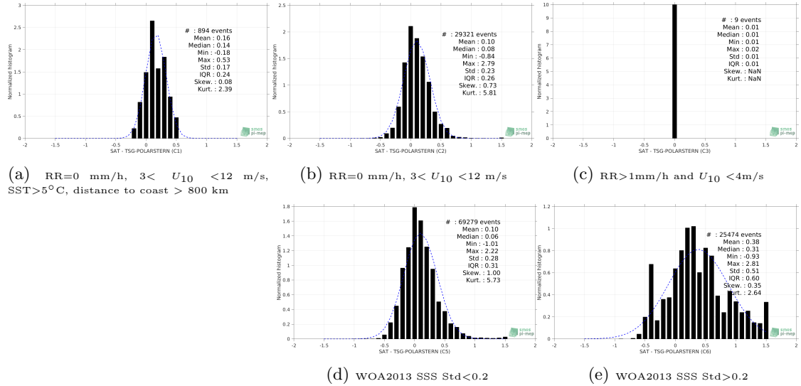
Figure 13: Normalized histogram of \Delta SSS (SMOS-L3-CATDS-CECOS-LOCEAN-V3-18DAYS-25KM - TSG-POLARSTERN) for 5 different subdatasets corresponding to: RR=0 mm/h, 3 < U_{10} < 12 m/s, SST > 5^\circ C , distance to coast > 800 km (a), RR=0 mm/h, 3 < U_{10} < 12 m/s (b), RR > 1 mm/h and U_{10} < 4 m/s (c), WOA2013 SSS Std < 0.2 (d), WOA2013 SSS Std > 0.2 (e).
