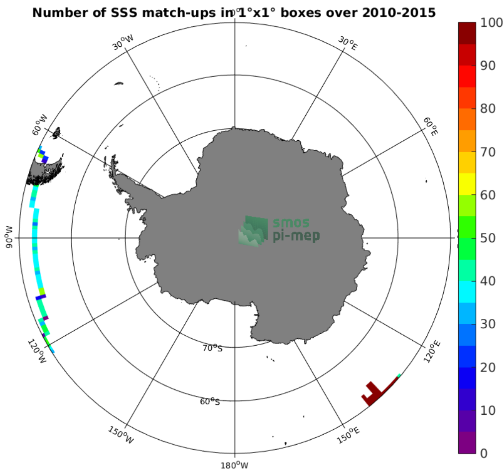
Figure 4: Number of SSS match-ups between TSG-GOSUD-Research-vessel SSS and the SMOS-L3-CATDS-CECOS-LOCEAN-V3-18DAYS-25KM SSS product for the Southern Ocean Pi-MEP region over 1^\circ \times 1^\circ boxes and for the full satellite product period.
