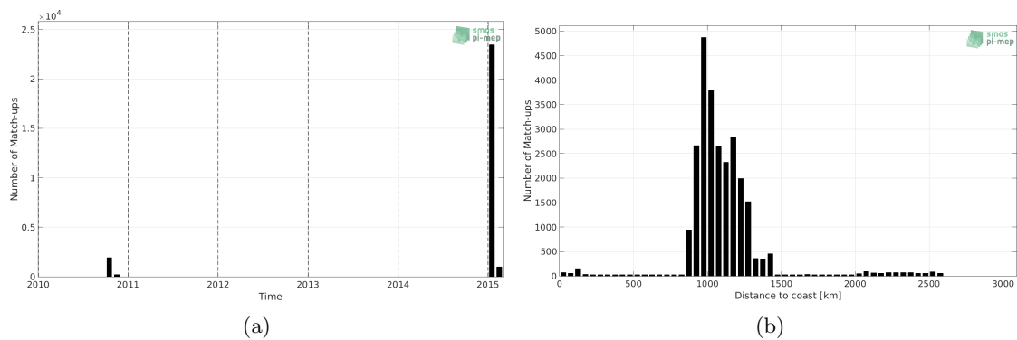
Figure 1: Number of match-ups between TSG-GOSUD-Research-vessel and SMOS-L3-CATDS-CECOS-LOCEAN-V3-18DAYS-25KM SSS as a function of time (a) and as function of the distance to coast (b) over the Southern Ocean Pi-MEP region and for the full satellite product period.
