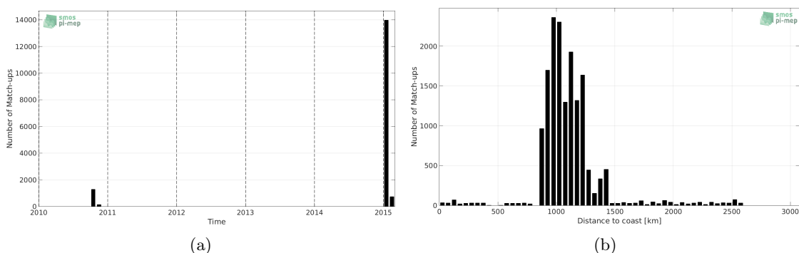
Figure 1: Number of match-ups between TSG-GOSUD-Research-vessel and SMOS-L3-CATDS-CECOS-LOCEAN-V3-18DAYS-25KM SSS as a function of time (a) and as function of the distance to coast (b) over the Southern Ocean Pi-MEP region and for the full satellite product period.
