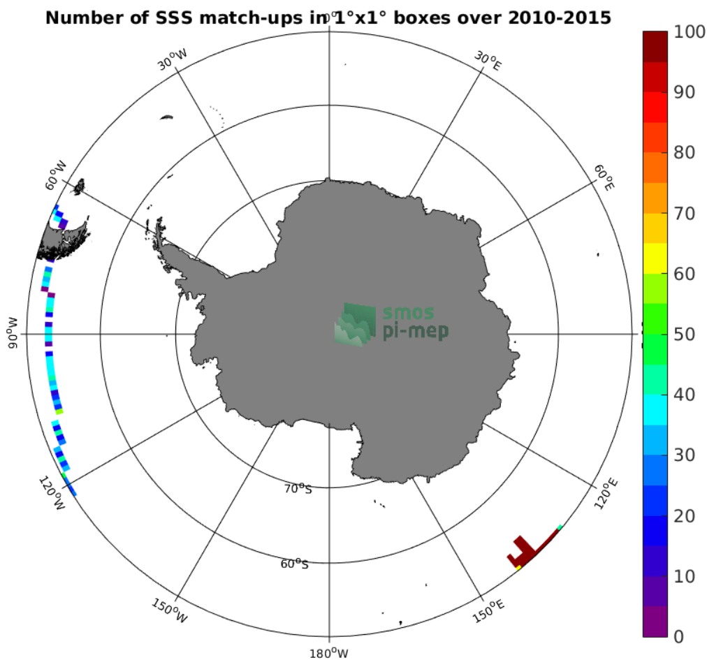
Figure 4: Number of SSS match-ups between TSG-GOSUD-Research-vessel SSS and the SMOS-L3-CATDS-CECOS-LOCEAN-V3-18DAYS-25KM SSS product for the Southern Ocean Pi-MEP region over 1°x1° boxes and for the full satellite product period.
