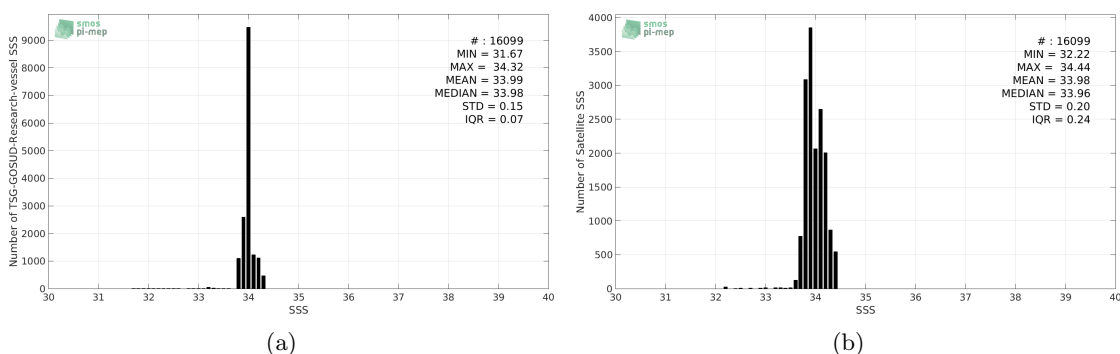
Figure 2: Histograms of SSS from TSG-GOSUD-Research-vessel (a) and SMOS-L3-CATDS-CECOS-LOCEAN-V3-18DAYS-25KM (b) considering all match-up pairs per bins of 0.1 over the Southern Ocean Pi-MEP region and for the full satellite product period.
