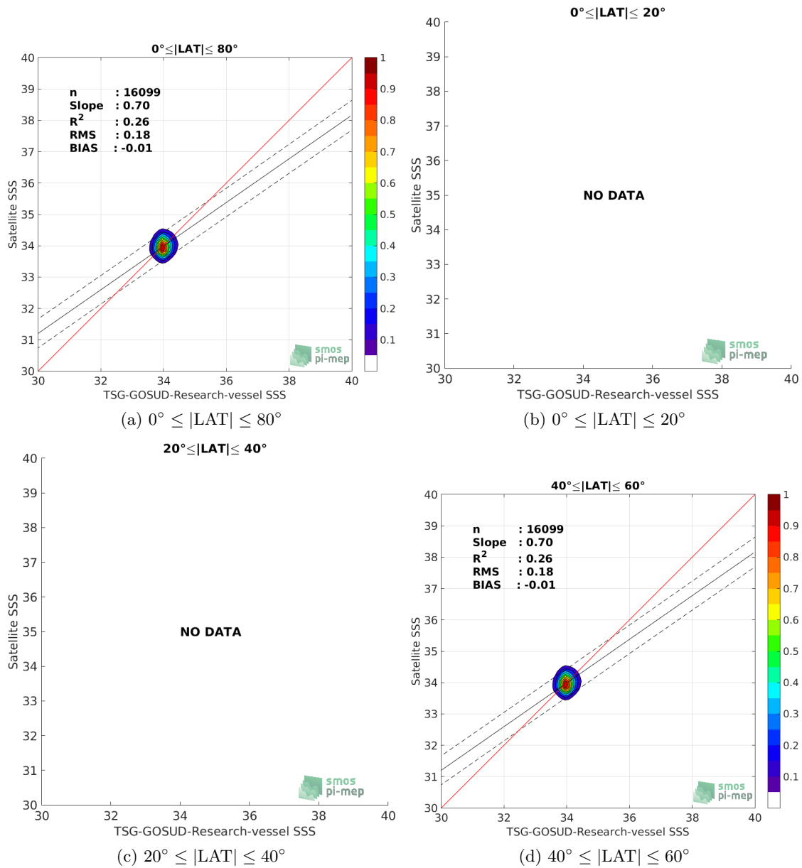
Figure 9: Contour maps of the concentration of SMOS-L3-CATDS-CECOS-LOCEAN-V3-18DAYS-25KM SSS (y-axis) versus TSG-GOSUD-Research-vessel SSS (x-axis) at match-up pairs for different latitude bands. For each plot, the red line shows x=y . The black thin and dashed lines indicate a linear fit through the data cloud and the \pm 95\% confidence levels, respectively. The number match-up pairs n , the slope and R^2 coefficient of the linear fit, the root mean square (RMS) and the mean bias between satellite and in situ data are indicated for each latitude band in each plots.
