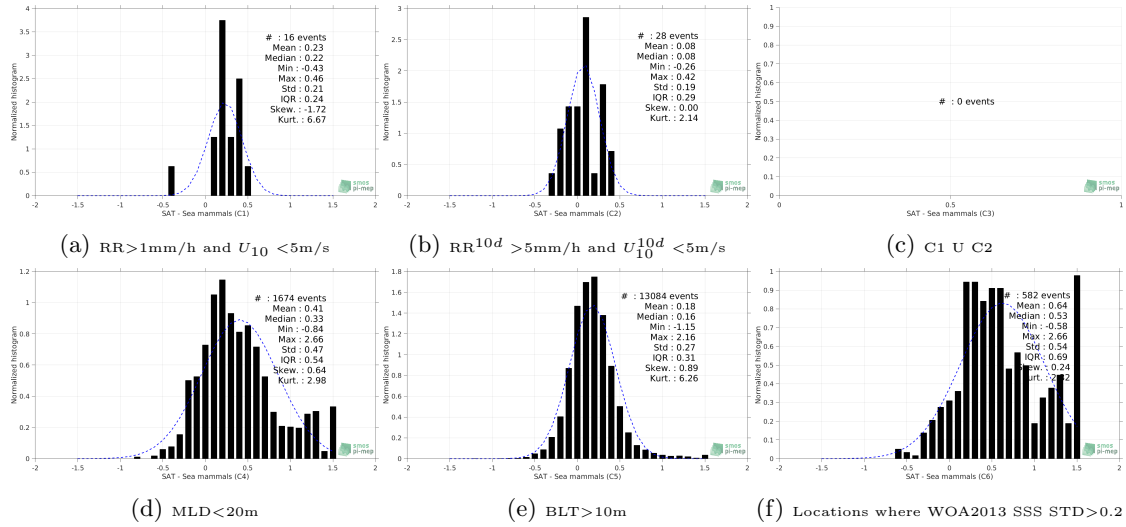
Figure 13: Normalized histogram of \Delta SSS (SMOS-L3-CATDS-CECOS-LOCEAN-V3-18DAYS-25KM - Sea mammals) for 6 different subdatasets corresponding to: RR > 1mm/h and U_{10} < 5 m/s (a), RR^{10d} > 5 mm/h and U_{10}^{10d} < 5 m/s (b), C1 U C2 (c), MLD < 20m (d), BLT > 10m (e), Locations where WOA2013 SSS STD > 0.2 (f).
