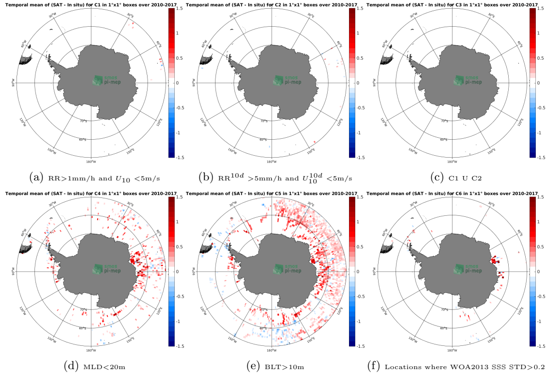
Figure 12: Temporal mean gridded over spatial boxes of size 1^\circ \times 1^\circ of \Delta SSS (SMOS-L3-CATDS-CECOS-LOCEAN-V3-18DAYS-25KM - Sea mammals) for 6 different subdatasets corresponding to: RR > 1\text{mm/h} and U_{10} < 5\text{m/s} (a), RR^{10d} > 5\text{mm/h} and U_{10}^{10d} < 5\text{m/s} (b), C1 U C2 (c), MLD < 20\text{m} (d), BLT > 10\text{m} (e), Locations where WOA2013 SSS STD > 0.2 (f).
