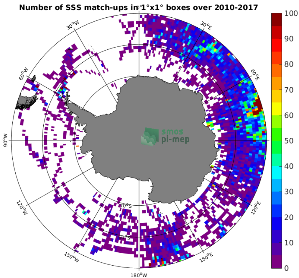
Figure 4: Number of SSS match-ups between Sea mammals SSS and the SMOS-L3-CATDS-CECOS-LOCEAN-V3-18DAYS-25KM SSS product for the Southern Ocean Pi-MEP region over 1°x1° boxes and for the full satellite product period.
