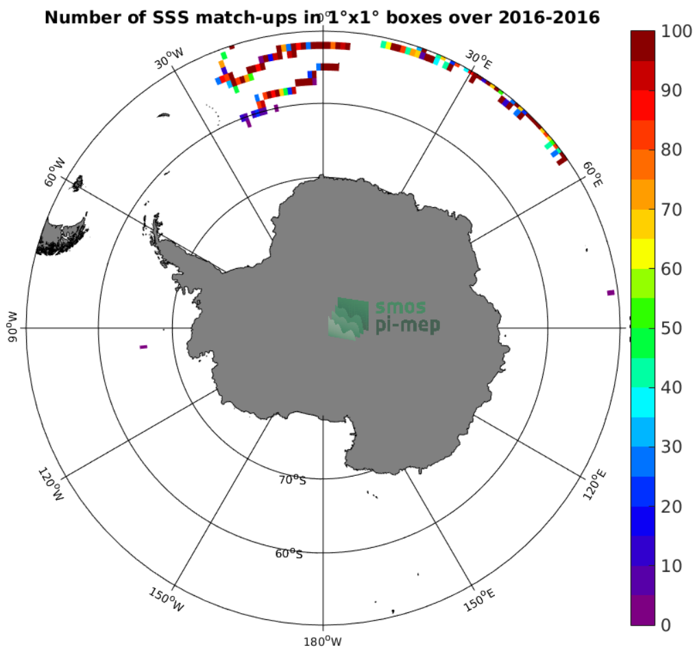
Figure 3: Number of SSS match-ups between Surface drifters SSS and the SMOS-L3-CATDS-CECOS-LOCEAN-V3-18DAYS-25KM SSS product for the Southern Ocean Pi-MEP region over 1°x1° boxes and for the full satellite product period.
