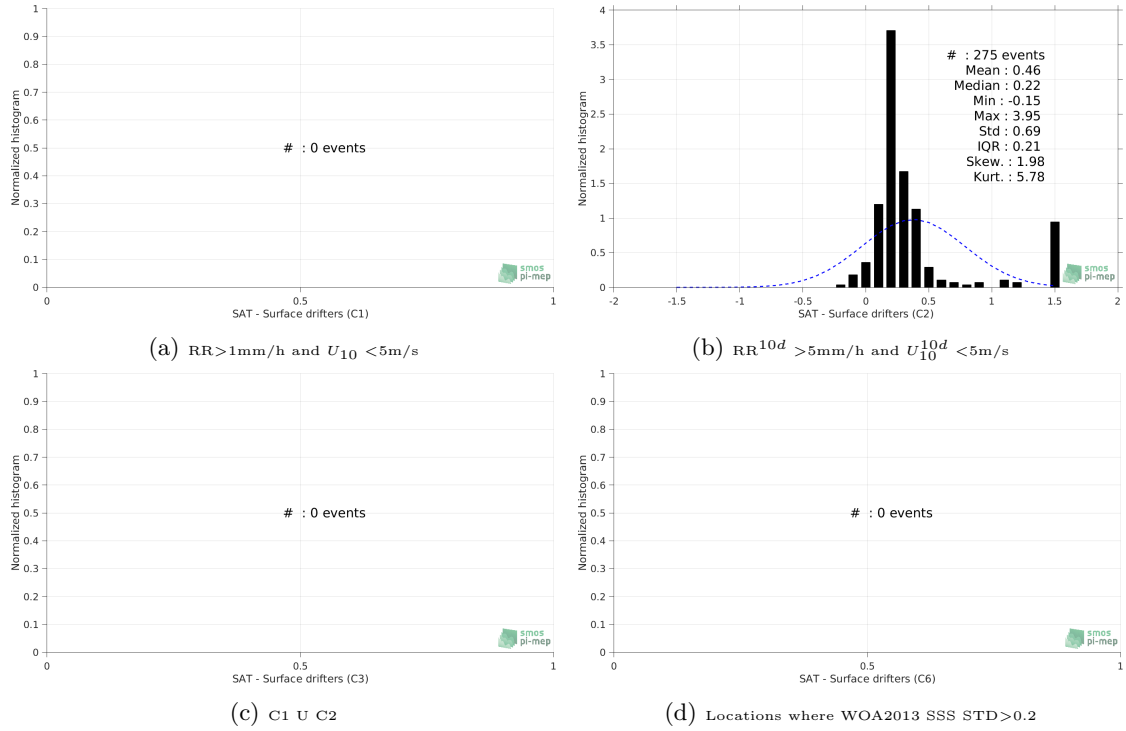
Figure 12: Normalized histogram of \Delta\text{SSS} (SMOS-L3-CATDS-CECOS-LOCEAN-V3-18DAYS-25KM - Surface drifters) for 6 different subdatasets corresponding to: RR > 1\text{mm/h} and U_{10} < 5\text{m/s} (a), RR^{10d} > 5\text{mm/h} and U_{10}^{10d} < 5\text{m/s} (b), C1 \cup C2 (c), Locations where WOA2013 SSS STD > 0.2 (d).
