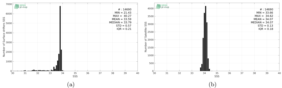
Figure 2: Histograms of SSS from Surface drifters (a) and SMOS-L3-CATDS-CECOS-LOCEAN-V3-18DAYS-25KM (b) considering all match-up pairs per bins of 0.1 over the Southern Ocean Pi-MEP region and for the full satellite product period.
