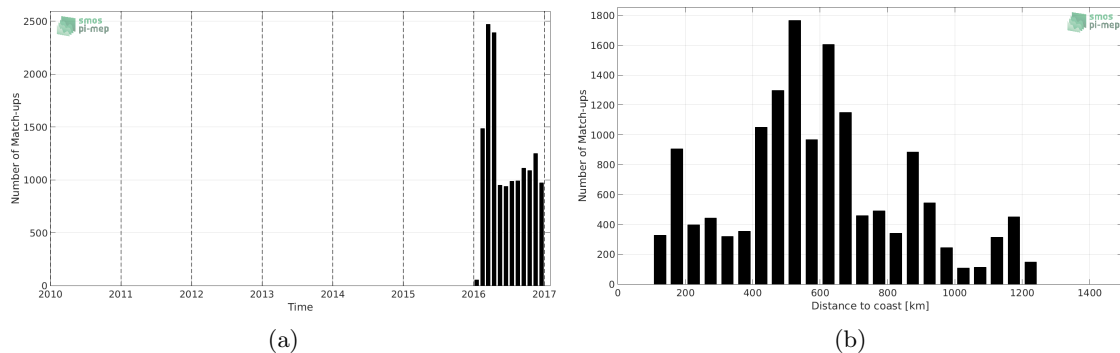
Figure 1: Number of match-ups between Surface drifters and SMOS-L3-CATDS-CECOS-LOCEAN-V3-18DAYS-25KM SSS as a function of time (a) and as function of the distance to coast (b) over the Southern Ocean Pi-MEP region and for the full satellite product period.
