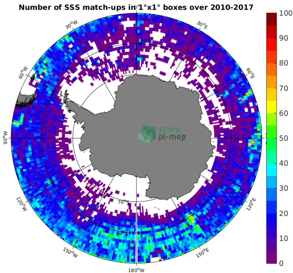
Figure 4: Number of SSS match-ups between Argo SSS and the SMOS-L3-CATDS-CECOS-LOCEAN-V3-18DAYS-25KM SSS product for the Southern Ocean Pi-MEP region over 1°x1° boxes and for the full satellite product period.
