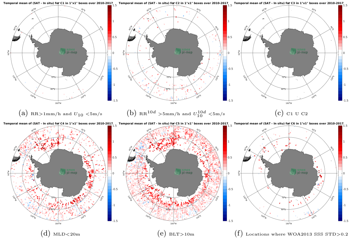
Figure 12: Temporal mean gridded over spatial boxes of size 1^\circ \times 1^\circ of \Delta SSS (SMOS-L3-CATDS-CECOS-LOCEAN-V3-18DAYS-25KM - Argo) for 6 different subdatasets corresponding to: RR > 1\text{mm/h} and U_{10} < 5\text{m/s} (a), RR^{10d} > 5\text{mm/h} and U_{10}^{10d} < 5\text{m/s} (b), C1 U C2 (c), MLD < 20\text{m} (d), BLT > 10\text{m} (e), Locations where WOA2013 SSS STD > 0.2 (f).
