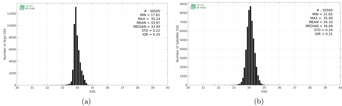
Figure 2: Histograms of SSS from Argo (a) and SMOS-L3-CATDS-CECOS-LOCEAN-V3-18DAYS-25KM (b) considering all match-up pairs per bins of 0.1 over the Southern Ocean Pi-MEP region and for the full satellite product period.
