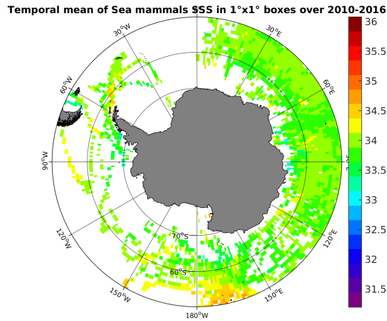
(c) MEAN(Sea mammals SSS)
