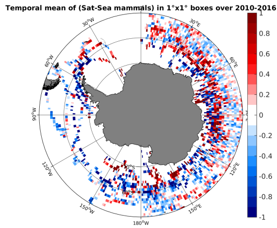
(e) MEAN( \Delta SSS) (Satellite - Sea mammals)
