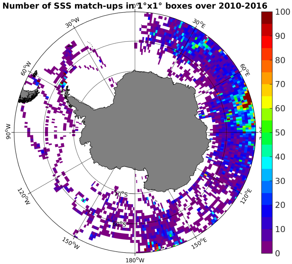
Figure 4: Number of SSS match-ups between Sea mammals SSS and the SMOS-L3-CATDS-CECOS-LOCEAN-V2-9DAYS-25KM SSS product for the Southern Ocean Pi-MEP region over 1^\circ \times 1^\circ boxes and for the full satellite product period.
