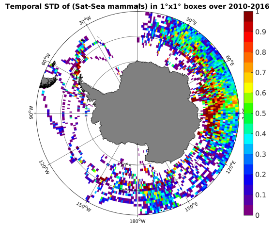
(f) STD( \Delta SSS) (Satellite - Sea mammals)
