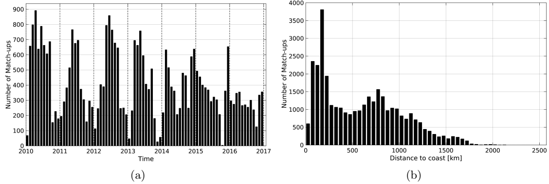
Figure 1: Number of match-ups between Sea mammals and SMOS-L3-CATDS-CECOS-LOCEAN-V2-9DAYS-25KM SSS as a function of time (a) and as function of the distance to coast (b) over the Southern Ocean Pi-MEP region and for the full satellite product period.
