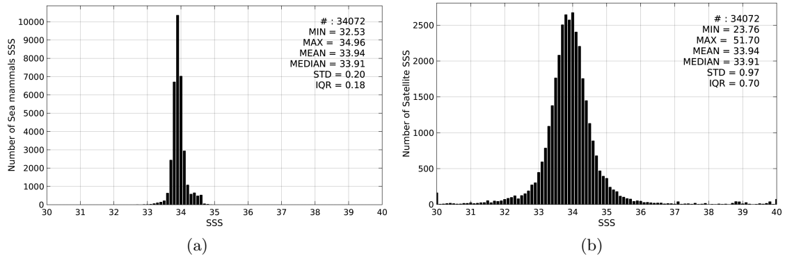
Figure 2: Histograms of SSS from Sea mammals (a) and SMOS-L3-CATDS-CECOS-LOCEAN-V2-9DAYS-25KM (b) considering all match-up pairs per bins of 0.1 over the Southern Ocean Pi-MEP region and for the full satellite product period.
