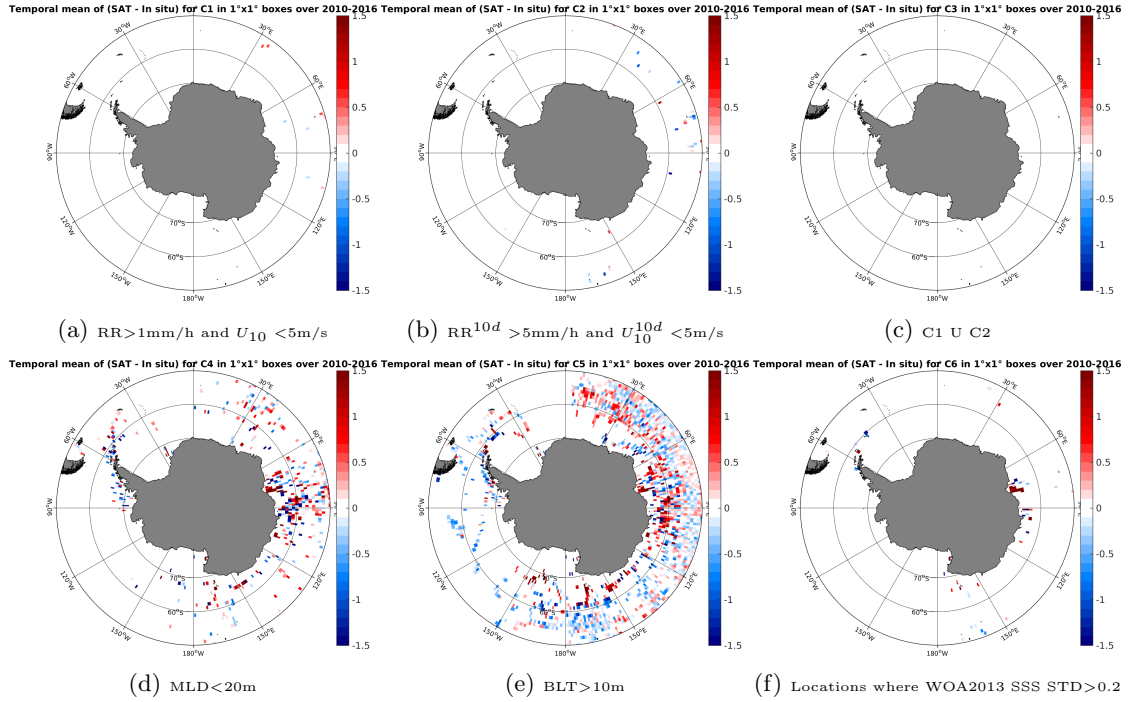
Figure 12: Temporal mean gridded over spatial boxes of size 1^\circ \times 1^\circ of \Delta SSS (SMOS-L3-CATDS-CECOS-LOCEAN-V2-9DAYS-25KM - Sea mammals) for 6 different subdatasets corresponding to: RR > 1\text{mm/h} and U_{10} < 5\text{m/s} (a), RR^{10d} > 5\text{mm/h} and U_{10}^{10d} < 5\text{m/s} (b), C1 U C2 (c), MLD < 20\text{m} (d), BLT > 10\text{m} (e), Locations where WOA2013 SSS STD > 0.2 (f).
