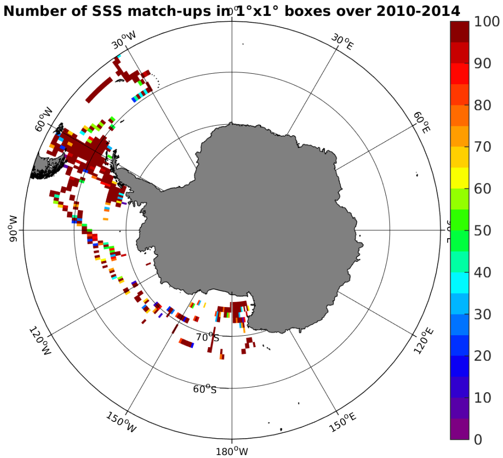
Figure 4: Number of SSS match-ups between TSG-SAMOS SSS and the SMOS-L3-CATDS-CECOS-LOCEAN-V2-18DAYS-25KM SSS product for the Southern Ocean Pi-MEP region over 1°x1° boxes and for the full satellite product period.
