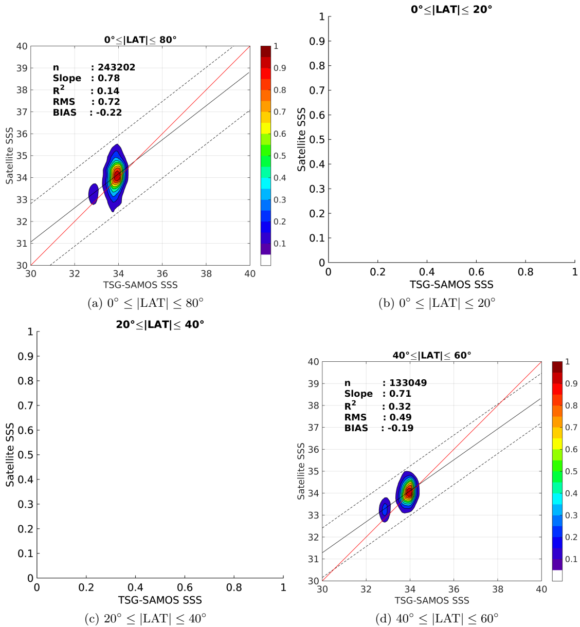
Figure 9: Contour maps of the concentration of SMOS-L3-CATDS-CECOS-LOCEAN-V2-18DAYS-25KM SSS (y-axis) versus TSG-SAMOS SSS (x-axis) at match-up pairs for different latitude bands. For each plot, the red line shows x=y . The black thin and dashed lines indicate a linear fit through the data cloud and the \pm 95\% confidence levels, respectively. The number match-up pairs n , the slope and R^2 coefficient of the linear fit, the root mean square (RMS) and the mean bias between satellite and in situ data are indicated for each latitude band in each plots.
