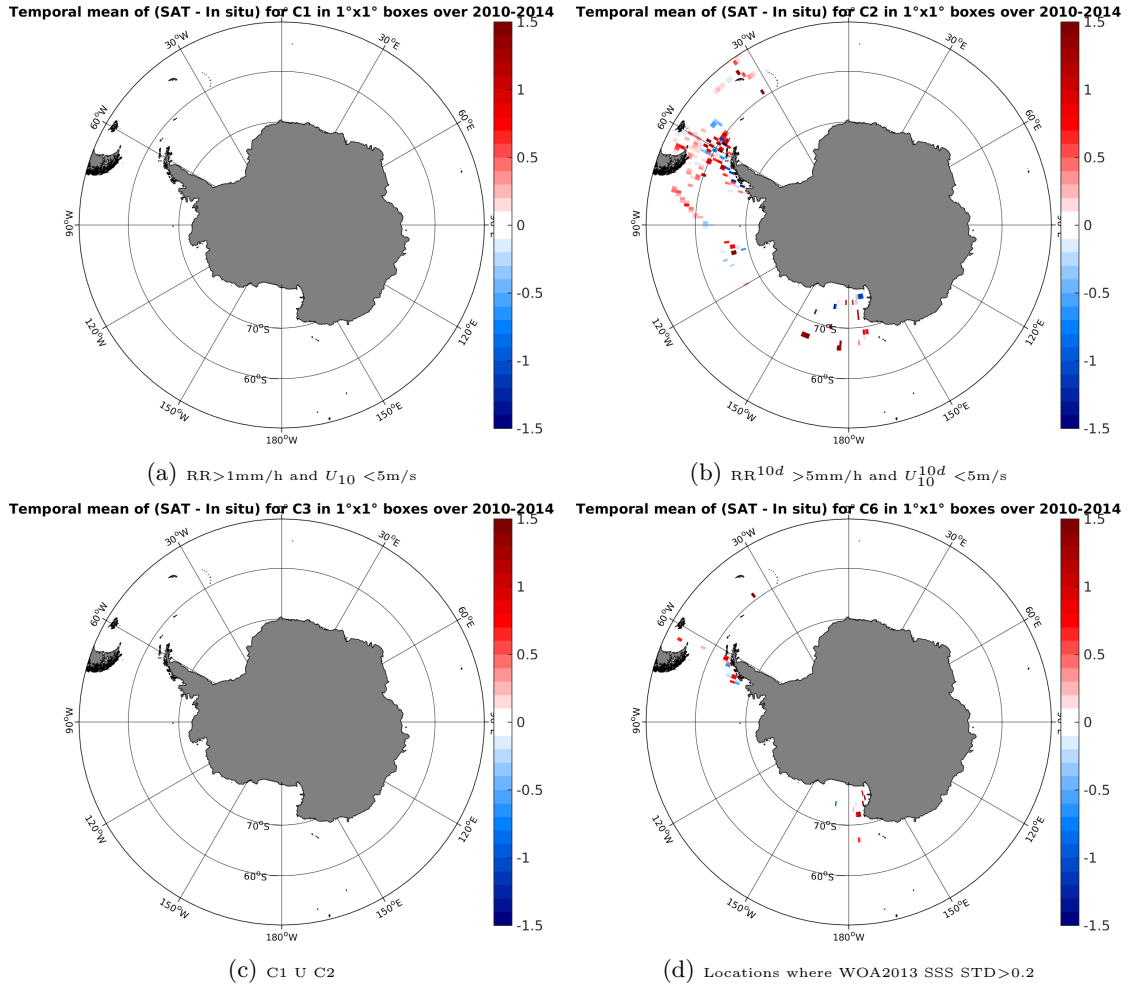
Figure 12: Temporal mean gridded over spatial boxes of size 1°x1° of \Delta SSS (SMOS-L3-CATDS-CECOS-LOCEAN-V2-18DAYS-25KM - TSG-SAMOS) for 4 different subdatasets corresponding to: RR > 1\text{mm/h} and U_{10} < 5\text{m/s} (a), RR^{10d} > 5\text{mm/h} and U_{10}^{10d} < 5\text{m/s} (b), C1 U C2 (c), Locations where WOA2013 SSS STD > 0.2 (d).
