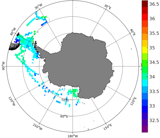
(c) MEAN(TSG-SAMOS SSS)
