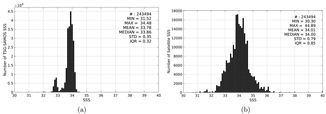
Figure 2: Histograms of SSS from TSG-SAMOS (a) and SMOS-L3-CATDS-CECOS-LOCEAN-V2-18DAYS-25KM (b) considering all match-up pairs per bins of 0.1 over the Southern Ocean Pi-MEP region and for the full satellite product period.
