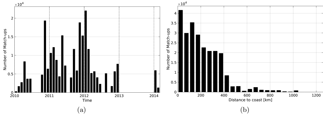
Figure 1: Number of match-ups between TSG-SAMOS and SMOS-L3-CATDS-CECOS-LOCEAN-V2-18DAYS-25KM SSS as a function of time (a) and as function of the distance to coast (b) over the Southern Ocean Pi-MEP region and for the full satellite product period.
