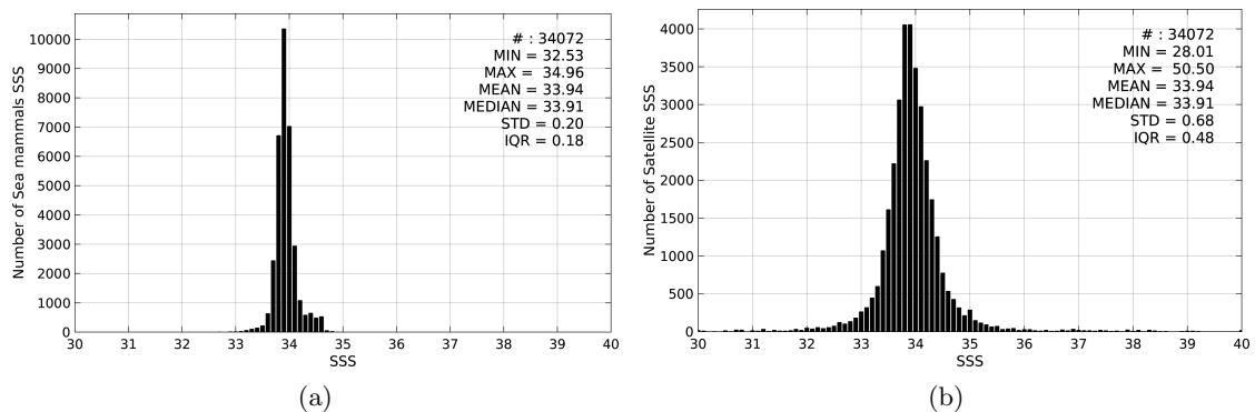
Figure 2: Histograms of SSS from Sea mammals (a) and SMOS-L3-CATDS-CECOS-LOCEAN-V2-18DAYS-25KM (b) considering all match-up pairs per bins of 0.1 over the Southern Ocean Pi-MEP region and for the full satellite product period.
