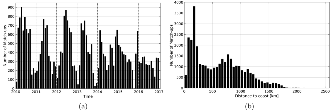
Figure 1: Number of match-ups between Sea mammals and SMOS-L3-CATDS-CECOS-LOCEAN-V2-18DAYS-25KM SSS as a function of time (a) and as function of the distance to coast (b) over the Southern Ocean Pi-MEP region and for the full satellite product period.
