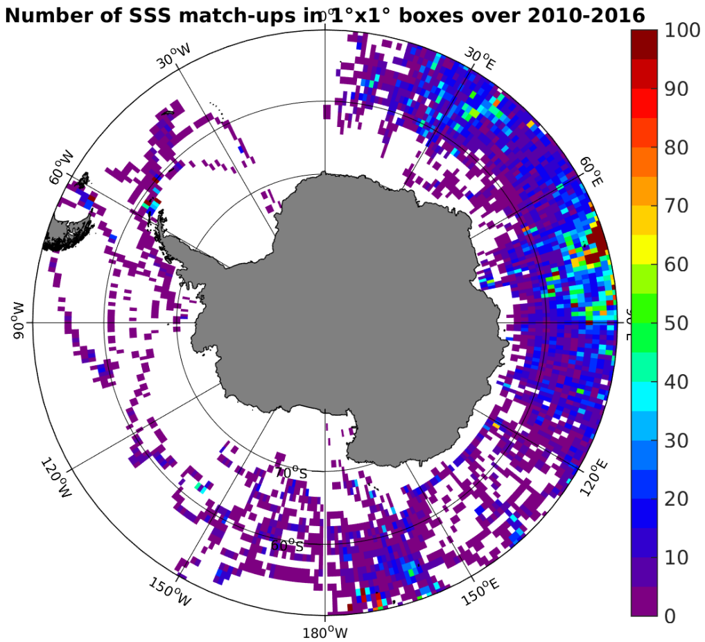
Figure 4: Number of SSS match-ups between Sea mammals SSS and the SMOS-L3-CATDS-CECOS-LOCEAN-V2-18DAYS-25KM SSS product for the Southern Ocean Pi-MEP region over 1°x1° boxes and for the full satellite product period.
