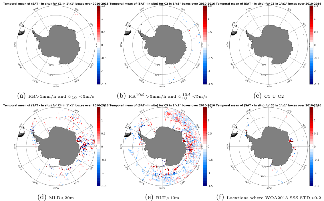
Figure 12: Temporal mean gridded over spatial boxes of size 1^\circ \times 1^\circ of \Delta SSS (SMOS-L3-CATDS-CECOS-LOCEAN-V2-18DAYS-25KM - Sea mammals) for 6 different subdatasets corresponding to: RR > 1\text{mm/h} and U_{10} < 5\text{m/s} (a), RR^{10d} > 5\text{mm/h} and U_{10}^{10d} < 5\text{m/s} (b), C1 U C2 (c), MLD < 20\text{m} (d), BLT > 10\text{m} (e), Locations where WOA2013 SSS STD > 0.2 (f).
