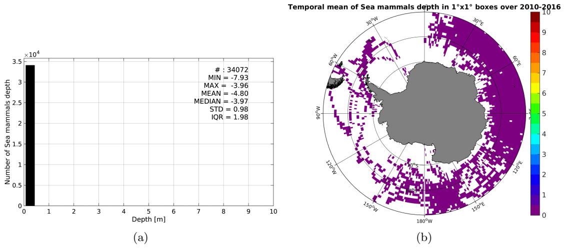
Figure 3: Histograms of the depth of the upper level SSS measurements from Sea mammals in the Match-up DataBase for the Southern Ocean Pi-MEP region (a) and temporal mean spatial distribution of pressure of the in situ SSS data over 1^\circ \times 1^\circ boxes and for the full satellite product period (b).
