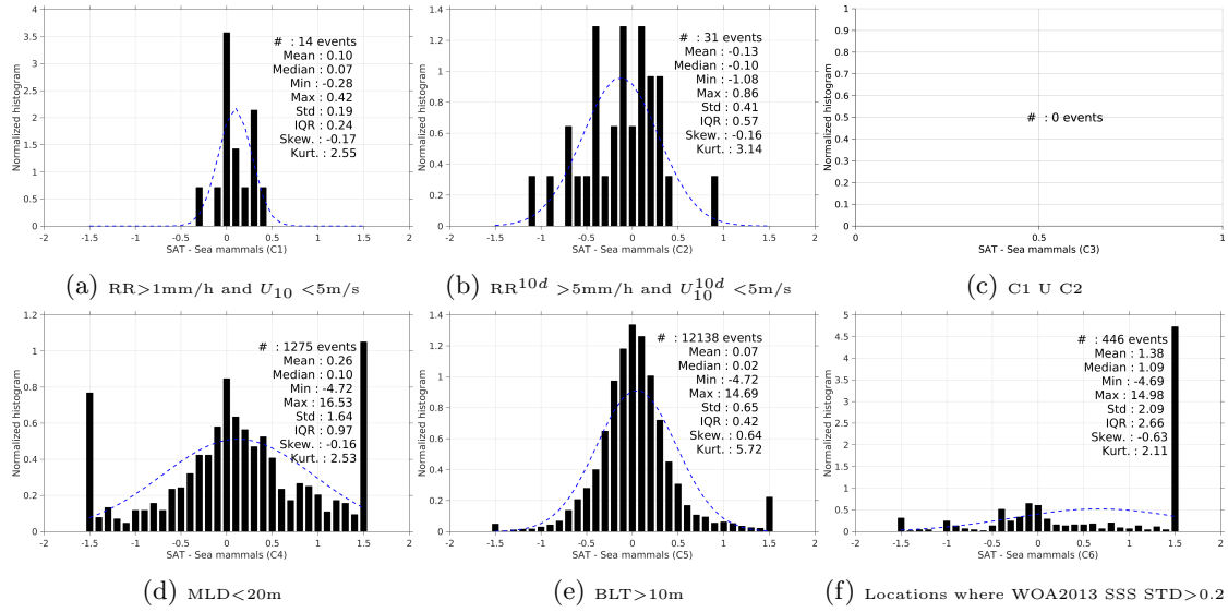
Figure 13: Normalized histogram of \Delta SSS (SMOS-L3-CATDS-CECOS-LOCEAN-V2-18DAYS-25KM - Sea mammals) for 6 different subdatasets corresponding to: RR>1mm/h and U_{10} < 5\text{m/s} (a), RR^{10d} > 5\text{mm/h} and U_{10}^{10d} < 5\text{m/s} (b), C1 U C2 (c),MLD<20m (d),BLT>10m (e),Locations where WOA2013 SSS STD>0.2 (f).
