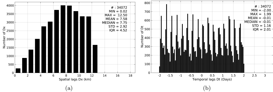
Figure 5: Histograms of the spatial (a) and temporal (b) lags between the time of the Sea mammals measurements and the date of the corresponding SMOS-L3-CATDS-CECOS-LOCEAN-V2-18DAYS-25KM SSS product.
