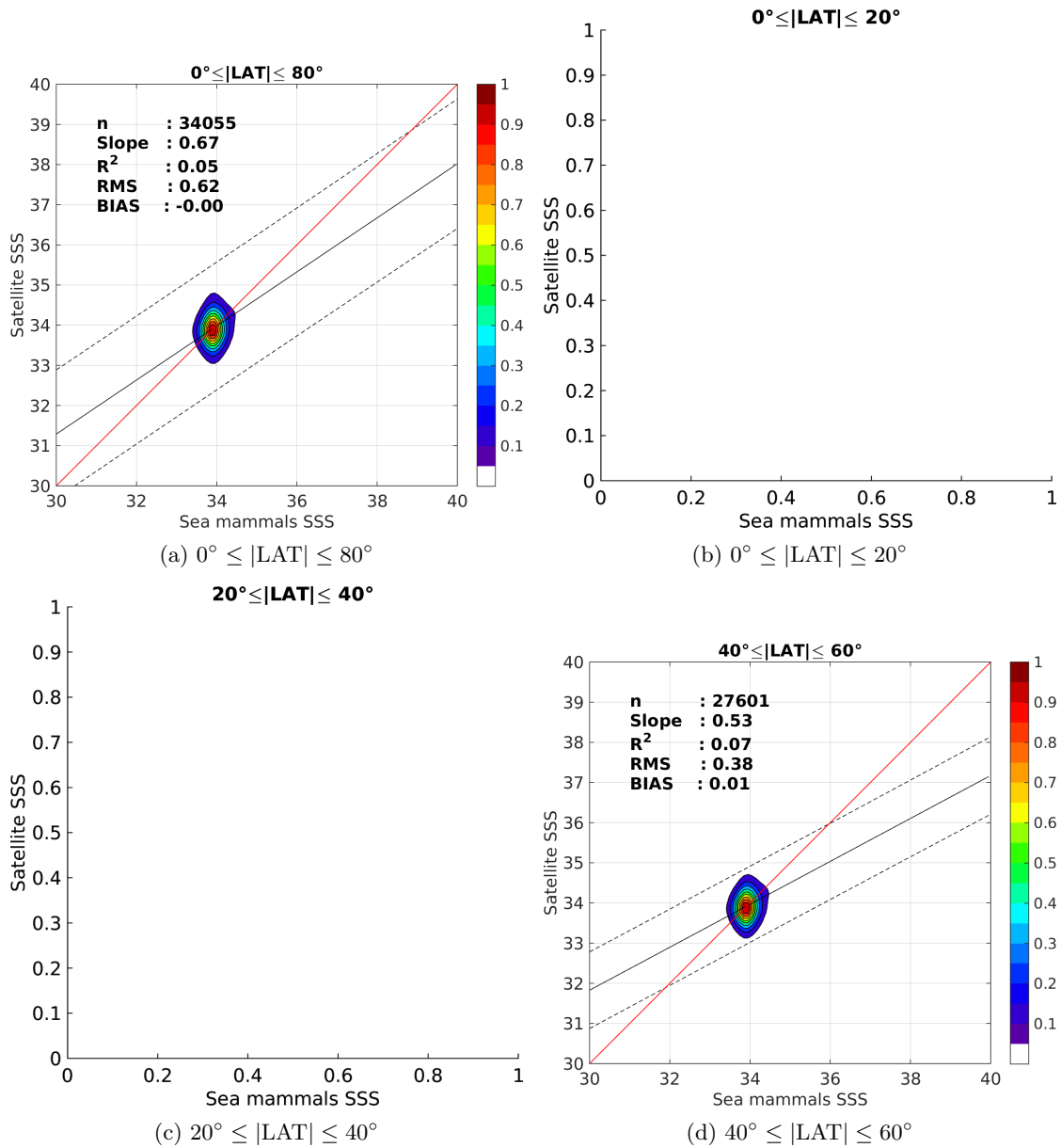
Figure 9: Contour maps of the concentration of SMOS-L3-CATDS-CECOS-LOCEAN-V2-18DAYS-25KM SSS (y-axis) versus Sea mammals SSS (x-axis) at match-up pairs for different latitude bands. For each plot, the red line shows x=y . The black thin and dashed lines indicate a linear fit through the data cloud and the \pm 95\% confidence levels, respectively. The number match-up pairs n , the slope and R^2 coefficient of the linear fit, the root mean square (RMS) and the mean bias between satellite and in situ data are indicated for each latitude band in each plots.
