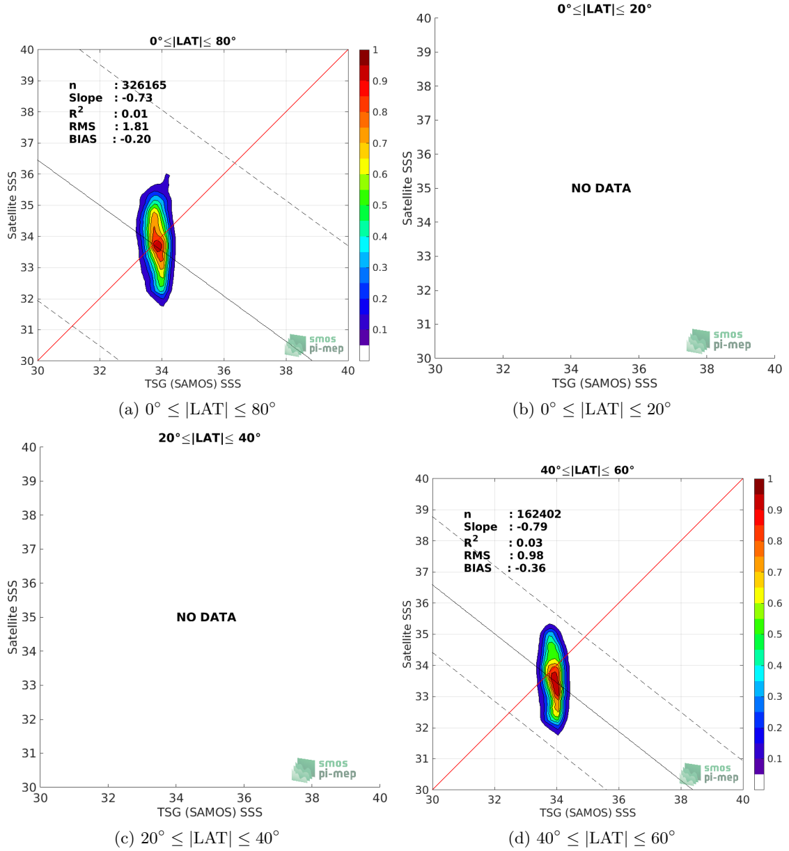
Figure 9: Contour maps of the concentration of SMOS SSS L3 v2 - Monthly - 0.25 Deg (CATDS-CECOS-IFREMER) SSS (y-axis) versus TSG (SAMOS) SSS (x-axis) at match-up pairs for different latitude bands. For each plot, the red line shows x=y . The black thin and dashed lines indicate a linear fit through the data cloud and the \pm 95\% confidence levels, respectively. The number match-up pairs n , the slope and R^2 coefficient of the linear fit, the root mean square (RMS) and the mean bias between satellite and in situ data are indicated for each latitude band in each plots.
