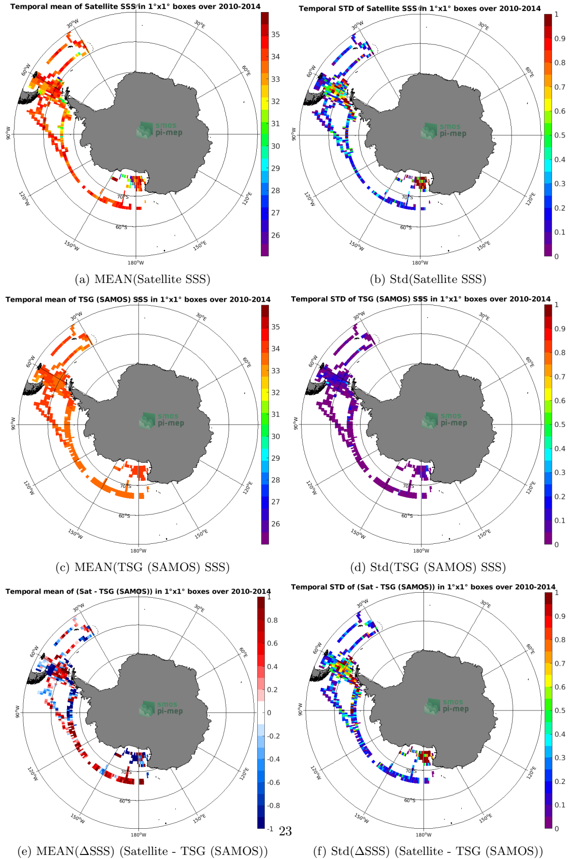
Figure 6: Temporal mean (left) and Std (right) of SSS from SMOS SSS L3 v2 - Monthly - 0.25 Deg (CATDS-CECOS-IFREMER) (top), TSG (SAMOS) (middle), and of \Delta SSS (Satellite - TSG (SAMOS)). Only match-up pairs are used to generate these maps.
