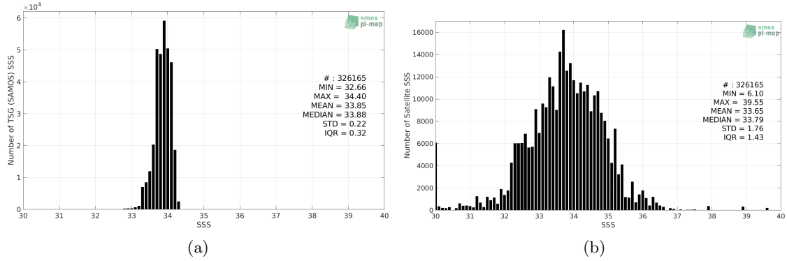
Figure 2: Histograms of SSS from TSG (SAMOS) (a) and SMOS SSS L3 v2 - Monthly - 0.25 Deg (CATDS-CECOS-IFREMER) (b) considering all match-up pairs per bins of 0.1 over the Southern Ocean Pi-MEP region and for the full satellite product period.
