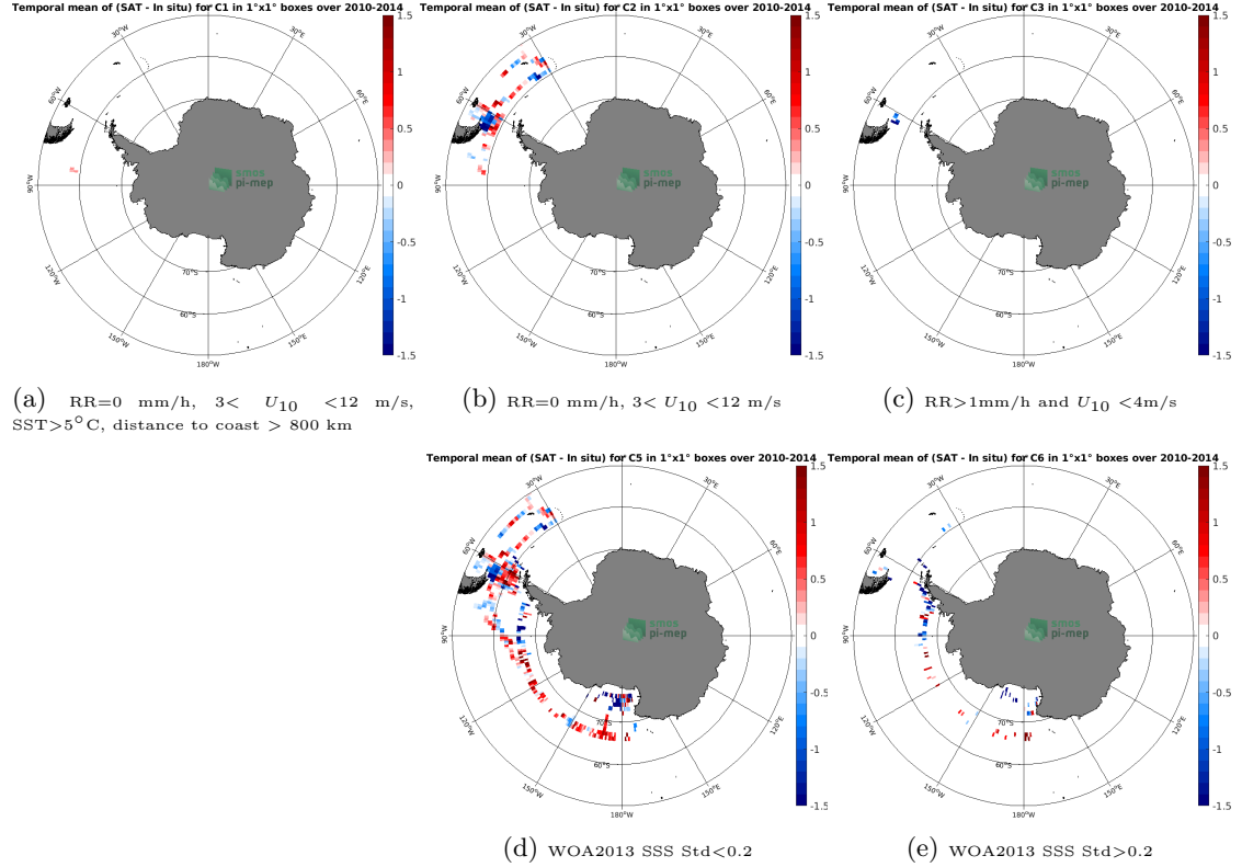
Figure 12: Temporal mean gridded over spatial boxes of size 1^{\circ}\times 1^{\circ} of \Delta\text{SSS} (SMOS SSS L3 v2 - Monthly - 0.25 Deg (CATDS-CECOS-IFREMER) - TSG (SAMOS)) for 5 different subdatasets corresponding to: RR=0 mm/h, 3 < U_{10} < 12 m/s, SST > 5^{\circ}\text{C} , distance to coast > 800 km (a), RR=0 mm/h, 3 < U_{10} < 12 m/s (b), RR > 1 mm/h and U_{10} < 4 m/s (c), WOA2013 SSS Std < 0.2 (d), WOA2013 SSS Std > 0.2 (e).
