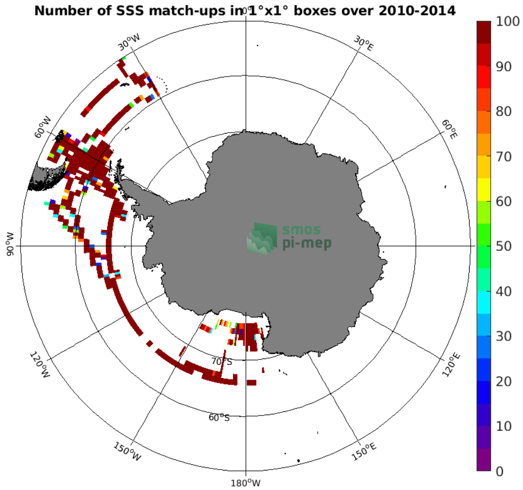
Figure 4: Number of SSS match-ups between TSG (SAMOS) SSS and the SMOS SSS L3 v2 - Monthly - 0.25 Deg (CATDS-CECOS-IFREMER) SSS product for the Southern Ocean Pi-MEP region over 1^\circ \times 1^\circ boxes and for the full satellite product period.
