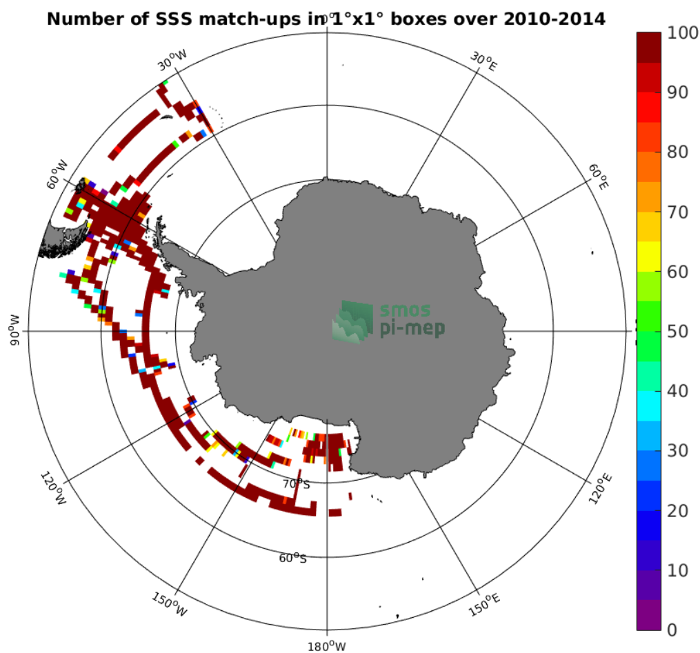
Figure 4: Number of SSS match-ups between TSG-SAMOS SSS and the SMOS L3 v2 - Monthly - 0.25 Deg (CATDS-CECOS-IFREMER) SSS product for the Southern Ocean Pi-MEP region over 1^\circ \times 1^\circ boxes and for the full satellite product period.
