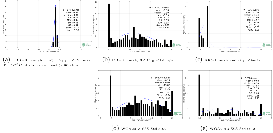
Figure 13: Normalized histogram of \Delta SSS (SMOS L3 v2 - Monthly - 0.25 Deg (CATDS-CECOS-IFREMER) - TSG-SAMOS) for 5 different subdatasets corresponding to: RR=0 mm/h, 3 < U_{10} < 12 m/s, SST>5°C, distance to coast > 800 km (a), RR=0 mm/h, 3 < U_{10} < 12 m/s (b), RR>1mm/h and U_{10} < 4 m/s (c), WOA2013 SSS Std<0.2 (d), WOA2013 SSS Std>0.2 (e).
