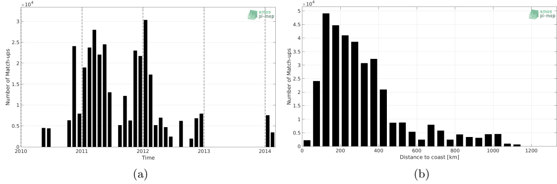
Figure 1: Number of match-ups between TSG-SAMOS and SMOS L3 v2 - Monthly - 0.25 Deg (CATDS-CECOS-IFREMER) SSS as a function of time (a) and as function of the distance to coast (b) over the Southern Ocean Pi-MEP region and for the full satellite product period.
