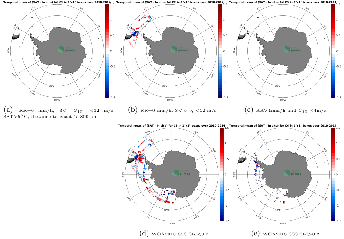
Figure 12: Temporal mean gridded over spatial boxes of size 1^{\circ}\times 1^{\circ} of \Delta\text{SSS} (SMOS L3 v2 - Monthly - 0.25 Deg (CATDS-CECOS-IFREMER) - TSG-SAMOS) for 5 different subdatasets corresponding to:RR=0 mm/h, 3 < U_{10} < 12 m/s, SST >5^{\circ}\text{C} , distance to coast > 800 km (a), RR=0 mm/h, 3 < U_{10} < 12 m/s (b), RR >1 mm/h and U_{10} < 4 m/s (c), WOA2013 SSS Std <0.2 (d), WOA2013 SSS Std >0.2 (e).
