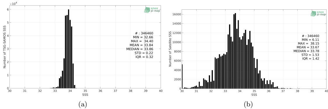
Figure 2: Histograms of SSS from TSG-SAMOS (a) and SMOS L3 v2 - Monthly - 0.25 Deg (CATDS-CECOS-IFREMER) (b) considering all match-up pairs per bins of 0.1 over the Southern Ocean Pi-MEP region and for the full satellite product period.
