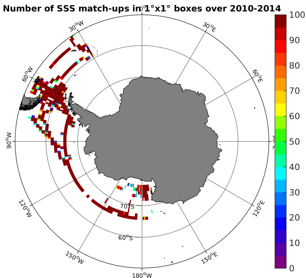
Figure 4: Number of SSS match-ups between TSG-SAMOS SSS and the SMOS-L3-CATDS-IFREMER-CECOS-V2-MONTHLY-0.25DEG SSS product for the Southern Ocean Pi-MEP region over 1^\circ \times 1^\circ boxes and for the full satellite product period.
