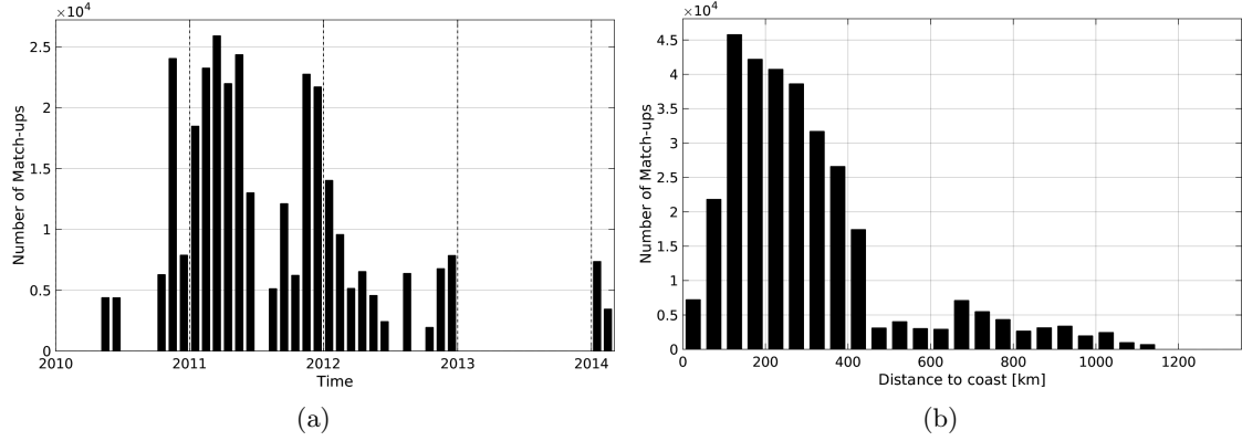
Figure 1: Number of match-ups between TSG-SAMOS and SMOS-L3-CATDS-IFREMER-CECOS-V2-MONTHLY-0.25DEG SSS as a function of time (a) and as function of the distance to coast (b) over the Southern Ocean Pi-MEP region and for the full satellite product period.
