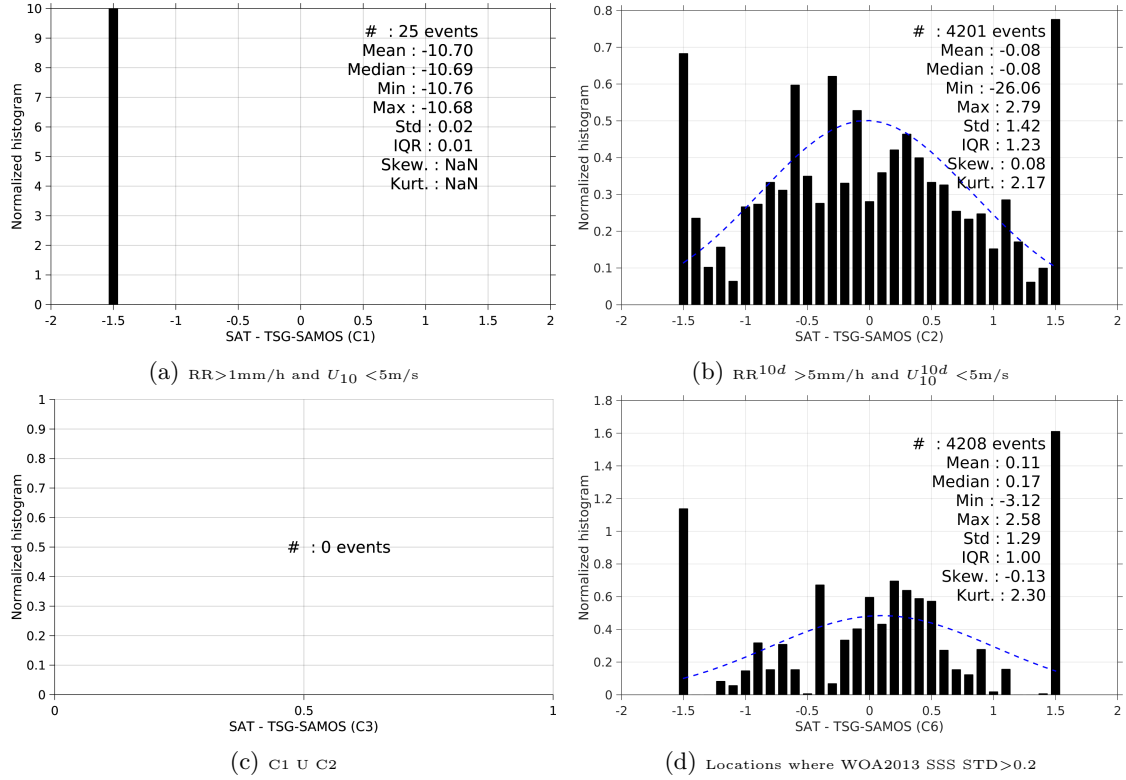
Figure 13: Normalized histogram of \Delta SSS (SMOS-L3-CATDS-IFREMER-CECOS-V2-MONTHLY-0.25DEG - TSG-SAMOS) for 6 different subdatasets corresponding to: RR > 1mm/h and U_{10} < 5\text{m/s} (a), RR^{10d} > 5\text{mm/h} and U_{10}^{10d} < 5\text{m/s} (b), C1 U C2 (c), Locations where WOA2013 SSS STD > 0.2 (d).
