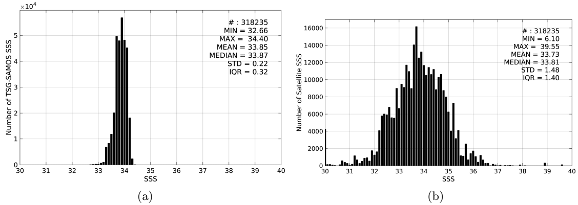
Figure 2: Histograms of SSS from TSG-SAMOS (a) and SMOS-L3-CATDS-IFREMER-CECOS-V2-MONTHLY-0.25DEG (b) considering all match-up pairs per bins of 0.1 over the Southern Ocean Pi-MEP region and for the full satellite product period.
