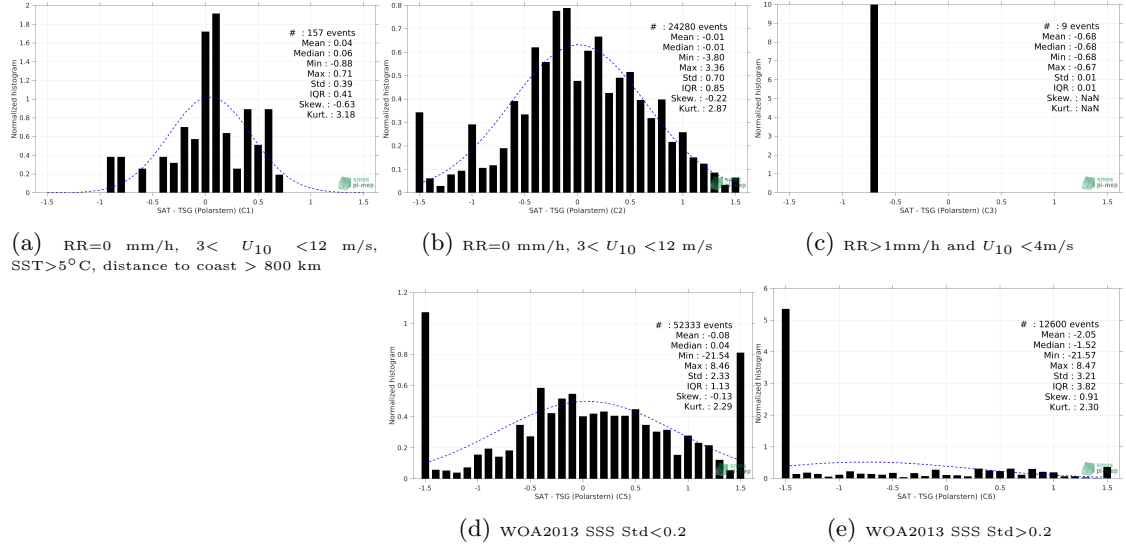
Figure 13: Normalized histogram of \Delta SSS (SMOS SSS L3 v2 - Monthly - 0.25 Deg (CATDS-CECOS-IFREMER) - TSG (Polarstern)) for 5 different subdatasets corresponding to: RR=0 mm/h, 3 < U_{10} < 12 m/s, SST>5°C, distance to coast > 800 km (a), RR=0 mm/h, 3 < U_{10} < 12 m/s (b), RR>1mm/h and U_{10} < 4 m/s (c), WOA2013 SSS Std<0.2 (d), WOA2013 SSS Std>0.2 (e).
