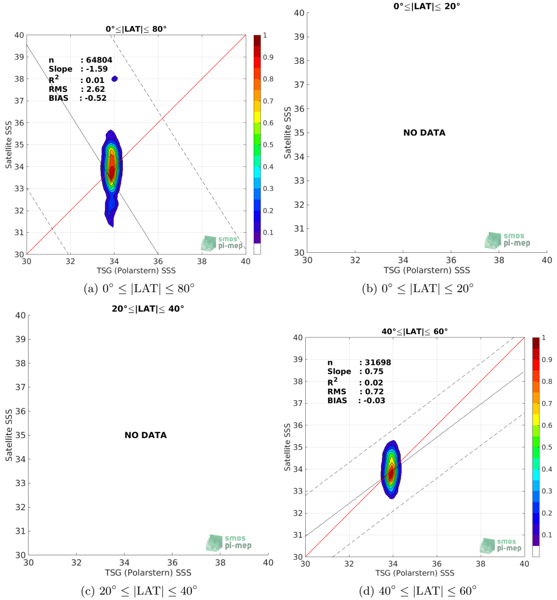
Figure 9: Contour maps of the concentration of SMOS SSS L3 v2 - Monthly - 0.25 Deg (CATDS-CECOS-IFREMER) SSS (y-axis) versus TSG (Polarstern) SSS (x-axis) at match-up pairs for different latitude bands. For each plot, the red line shows x=y . The black thin and dashed lines indicate a linear fit through the data cloud and the \pm 95\% confidence levels, respectively. The number match-up pairs n , the slope and R^2 coefficient of the linear fit, the root mean square (RMS) and the mean bias between satellite and in situ data are indicated for each latitude band in each plots.
