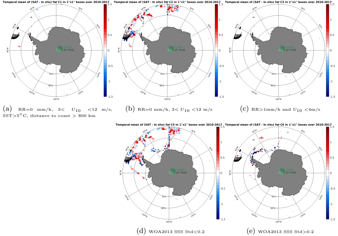
Figure 12: Temporal mean gridded over spatial boxes of size 1^{\circ}\times 1^{\circ} of \Delta\text{SSS} (SMOS SSS L3 v2 - Monthly - 0.25 Deg (CATDS-CECOS-IFREMER) - TSG (Polarstern)) for 5 different subdatasets corresponding to: RR=0 mm/h, 3 < U_{10} < 12 m/s, SST > 5^{\circ}\text{C} , distance to coast > 800 km (a), RR=0 mm/h, 3 < U_{10} < 12 m/s (b), RR > 1 mm/h and U_{10} < 4 m/s (c), WOA2013 SSS Std < 0.2 (d), WOA2013 SSS Std > 0.2 (e).
