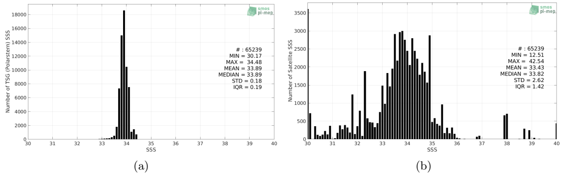
Figure 2: Histograms of SSS from TSG (Polarstern) (a) and SMOS SSS L3 v2 - Monthly - 0.25 Deg (CATDS-CECOS-IFREMER) (b) considering all match-up pairs per bins of 0.1 over the Southern Ocean Pi-MEP region and for the full satellite product period.
