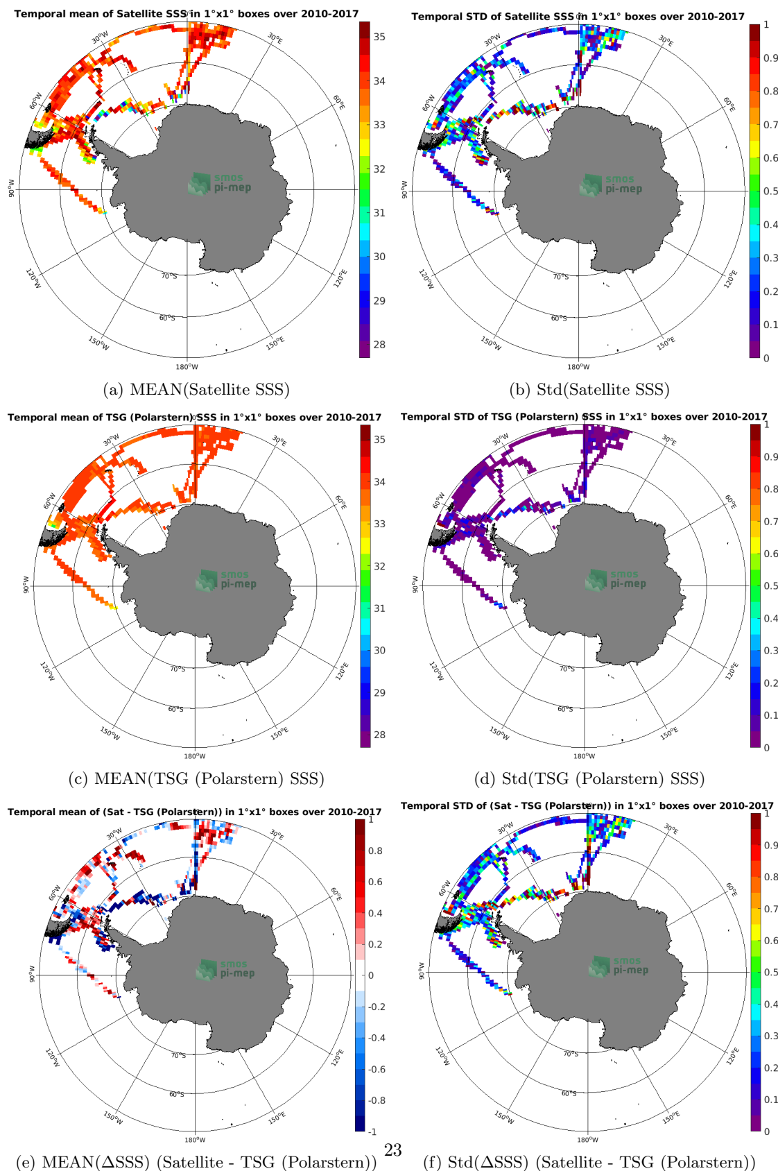
Figure 6: Temporal mean (left) and Std (right) of SSS from SMOS SSS L3 v2 - Monthly - 0.25 Deg (CATDS-CECOS-IFREMER) (top), TSG (Polarstern) (middle), and of \Delta SSS (Satellite - TSG (Polarstern)). Only match-up pairs are used to generate these maps.
