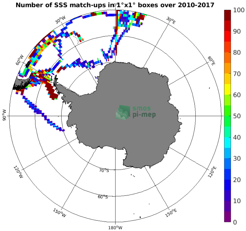
Figure 4: Number of SSS match-ups between TSG (Polarstern) SSS and the SMOS SSS L3 v2 - Monthly - 0.25 Deg (CATDS-CECOS-IFREMER) SSS product for the Southern Ocean Pi-MEP region over 1^\circ \times 1^\circ boxes and for the full satellite product period.
