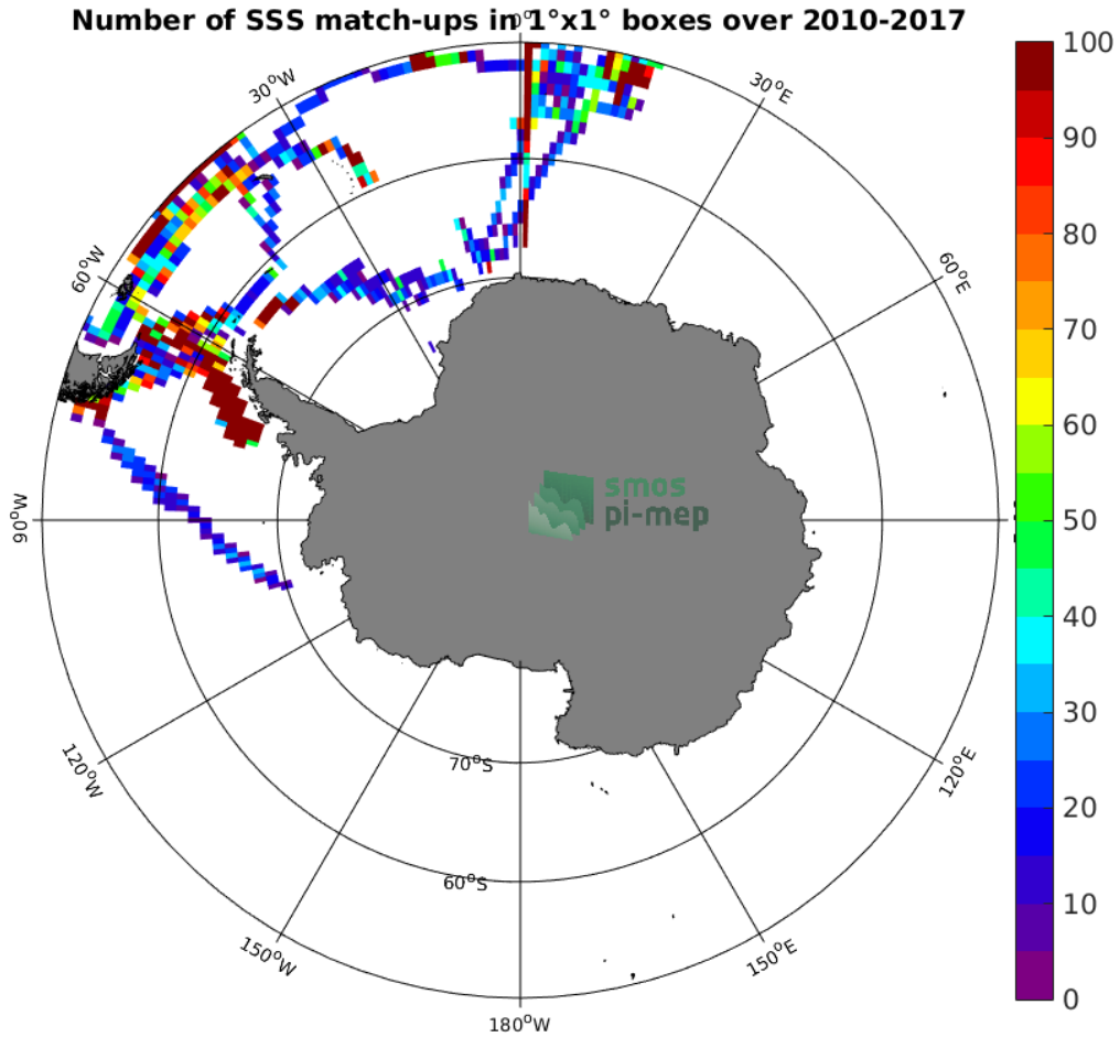
Figure 4: Number of SSS match-ups between TSG (Polarstern) SSS and the SMOS SSS L3 v2 - Monthly - 0.25 Deg (CATDS-CECOS-IFREMER) SSS product for the Southern Ocean Pi-MEP region over 1^\circ \times 1^\circ boxes and for the full satellite product period.
