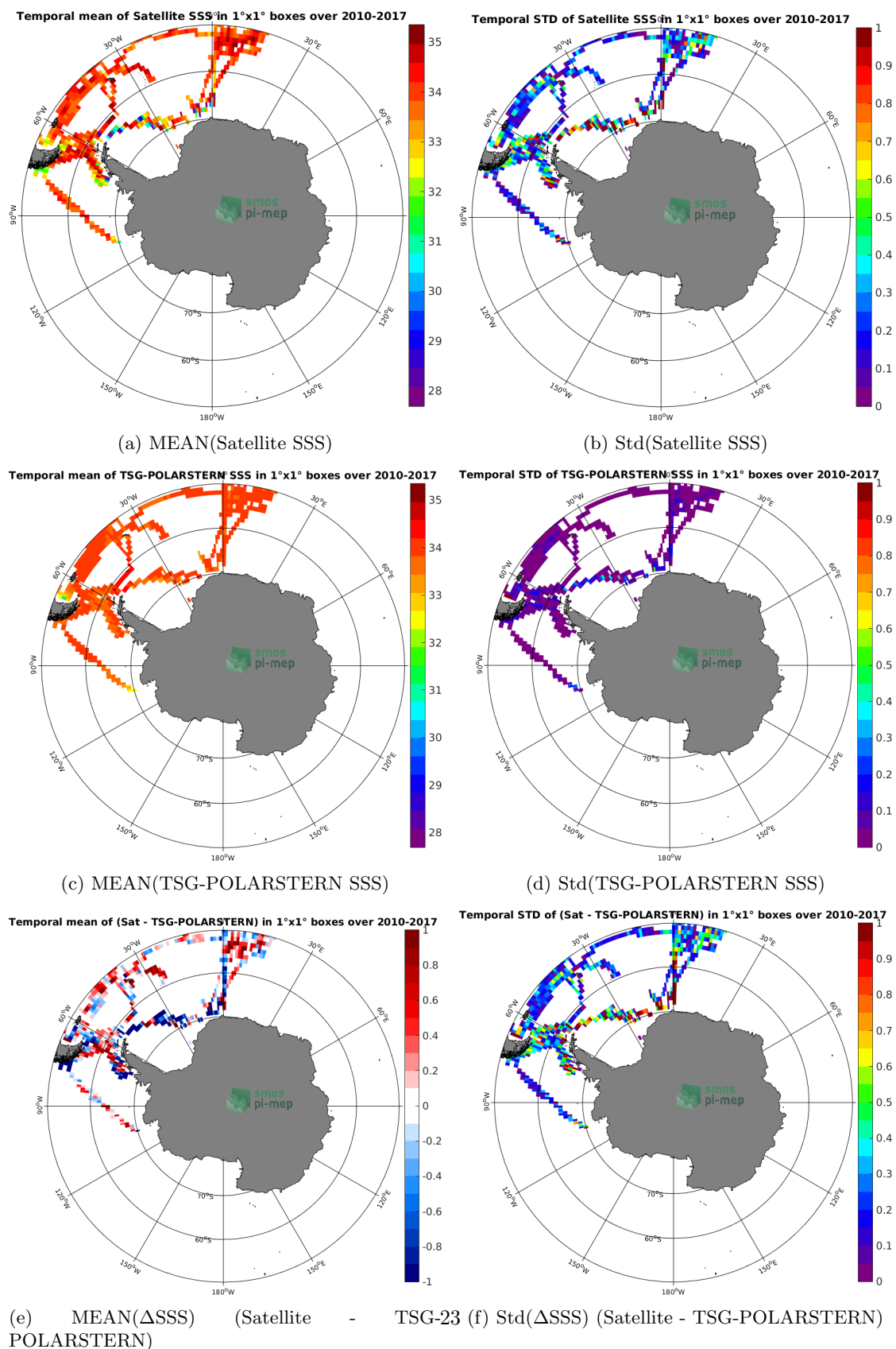
Figure 6: Temporal mean (left) and Std (right) of SSS from SMOS L3 v2 - Monthly - 0.25 Deg (CATDS-CECOS-IFREMER) (top), TSG-POLARSTERN (middle), and of \Delta SSS (Satellite - TSG-POLARSTERN). Only match-up pairs are used to generate these maps.
