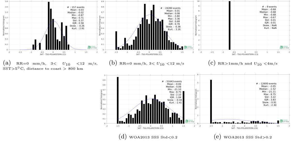
Figure 13: Normalized histogram of \Delta\text{SSS} (SMOS L3 v2 - Monthly - 0.25 Deg (CATDS-CECOS-IFREMER) - TSG-POLARSTERN) for 5 different subdatasets corresponding to: RR=0 mm/h, 3 < U_{10} < 12 m/s, SST > 5^{\circ}\text{C} , distance to coast > 800 km (a), RR=0 mm/h, 3 < U_{10} < 12 m/s (b), RR > 1\text{mm/h} and U_{10} < 4\text{m/s} (c), WOA2013 SSS Std < 0.2 (d), WOA2013 SSS Std > 0.2 (e).
