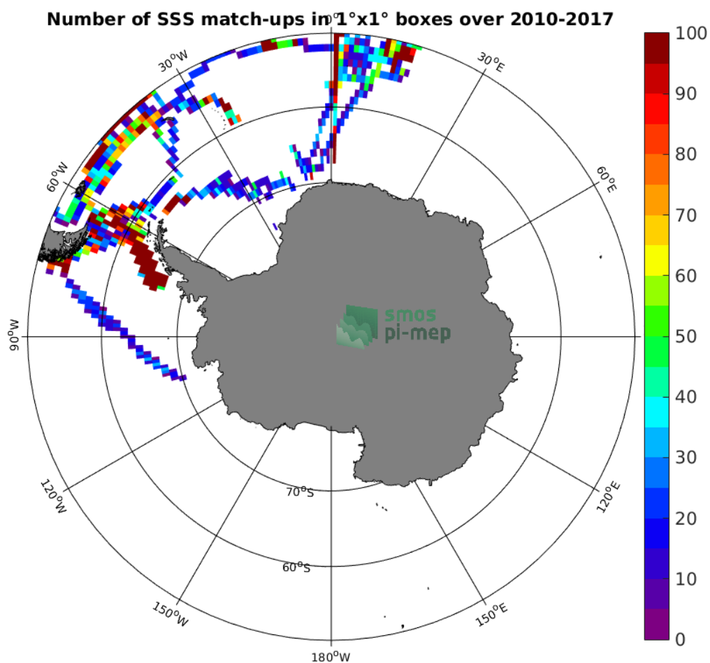
Figure 4: Number of SSS match-ups between TSG-POLARSTERN SSS and the SMOS L3 v2 - Monthly - 0.25 Deg (CATDS-CECOS-IFREMER) SSS product for the Southern Ocean Pi-MEP region over 1^\circ \times 1^\circ boxes and for the full satellite product period.
