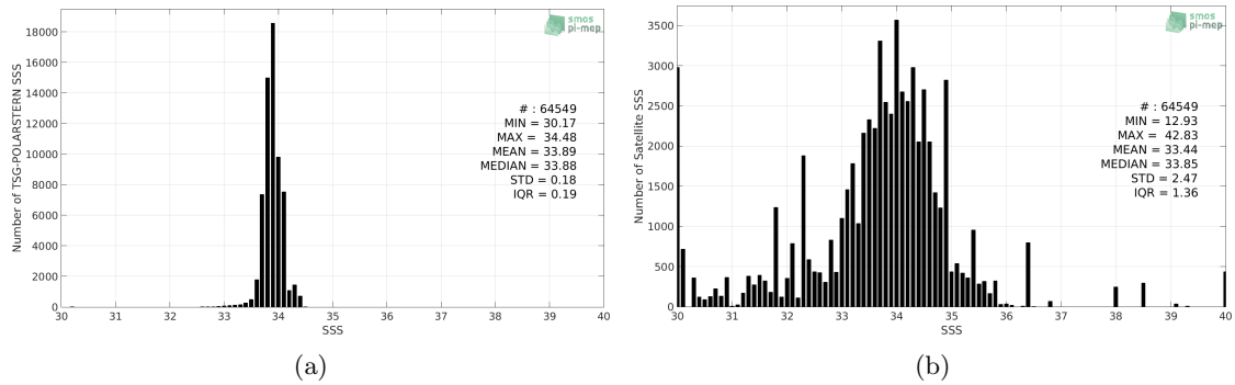
Figure 2: Histograms of SSS from TSG-POLARSTERN (a) and SMOS L3 v2 - Monthly - 0.25 Deg (CATDS-CECOS-IFREMER) (b) considering all match-up pairs per bins of 0.1 over the Southern Ocean Pi-MEP region and for the full satellite product period.
