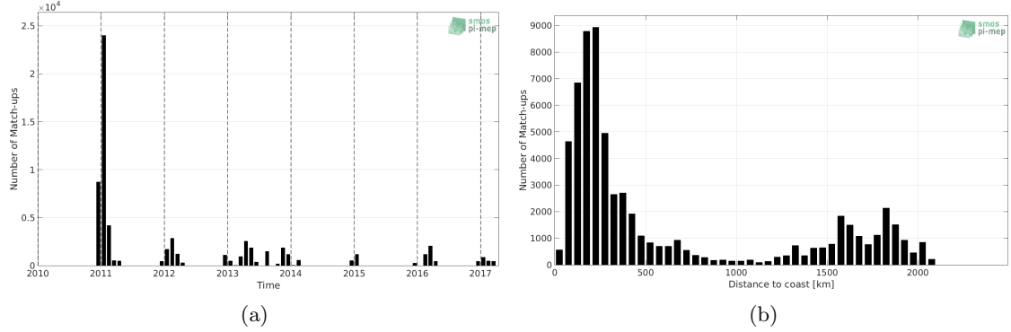
Figure 1: Number of match-ups between TSG-POLARSTERN and SMOS L3 v2 - Monthly - 0.25 Deg (CATDS-CECOS-IFREMER) SSS as a function of time (a) and as function of the distance to coast (b) over the Southern Ocean Pi-MEP region and for the full satellite product period.
