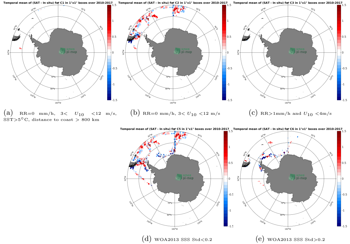
Figure 12: Temporal mean gridded over spatial boxes of size 1^{\circ}\times 1^{\circ} of \Delta\text{SSS} (SMOS L3 v2 - Monthly - 0.25 Deg (CATDS-CECOS-IFREMER) - TSG-POLARSTERN) for 5 different sub-datasets corresponding to:RR=0 mm/h, 3 < U_{10} < 12 m/s, SST >5^{\circ}\text{C} , distance to coast > 800 km (a), RR=0 mm/h, 3 < U_{10} < 12 m/s (b), RR >1 mm/h and U_{10} < 4 m/s (c), WOA2013 SSS Std <0.2 (d), WOA2013 SSS Std >0.2 (e).
