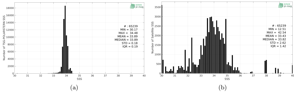
Figure 2: Histograms of SSS from TSG-POLARSTERN (a) and SMOS-L3-CATDS-IFREMER-CECOS-V2-MONTHLY-0.25DEG (b) considering all match-up pairs per bins of 0.1 over the Southern Ocean Pi-MEP region and for the full satellite product period.
