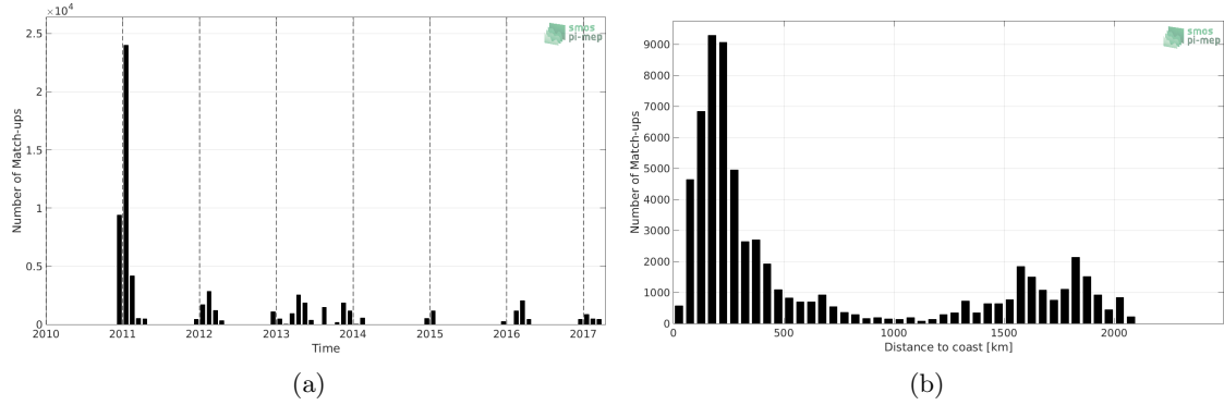
Figure 1: Number of match-ups between TSG-POLARSTERN and SMOS-L3-CATDS-IFREMER-CECOS-V2-MONTHLY-0.25DEG SSS as a function of time (a) and as function of the distance to coast (b) over the Southern Ocean Pi-MEP region and for the full satellite product period.
