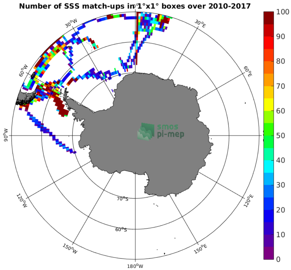
Figure 4: Number of SSS match-ups between TSG-POLARSTERN SSS and the SMOS-L3-CATDS-IFREMER-CECOS-V2-MONTHLY-0.25DEG SSS product for the Southern Ocean Pi-MEP region over 1^\circ \times 1^\circ boxes and for the full satellite product period.
