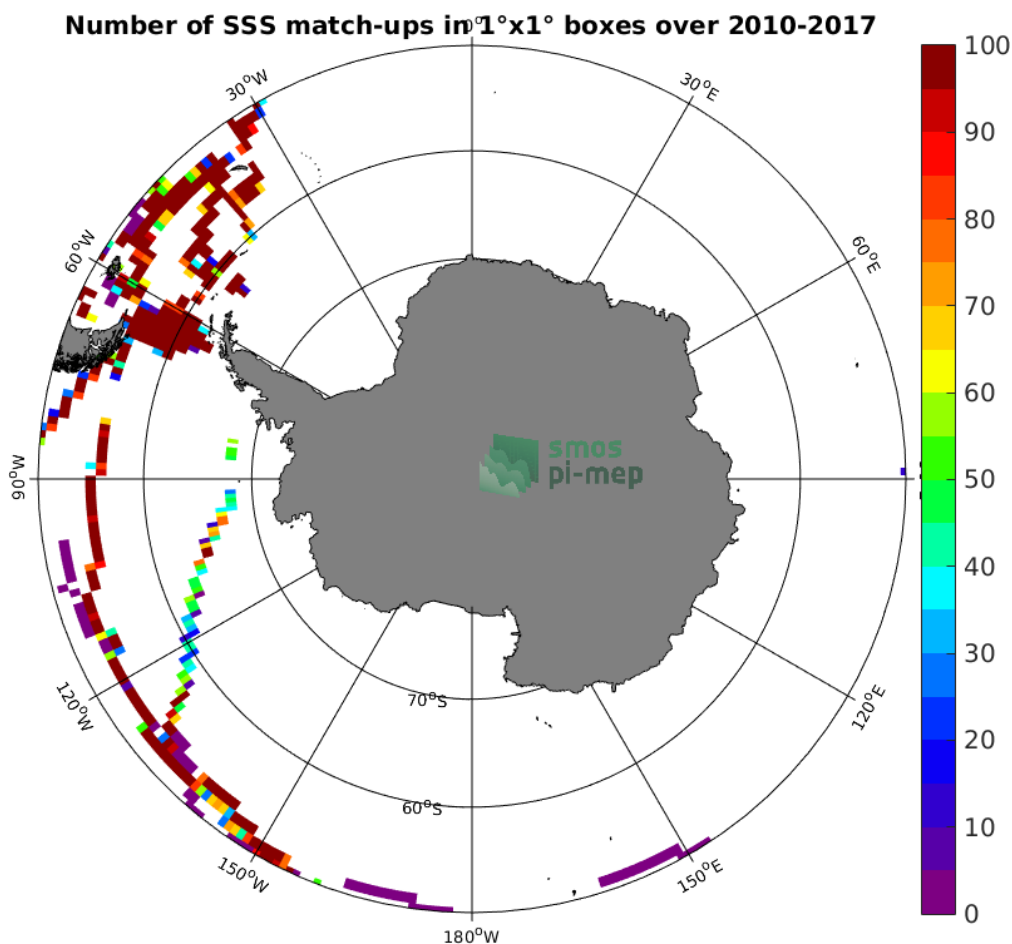
Figure 4: Number of SSS match-ups between TSG (GOSUD-Sailing-ship) SSS and the SMOS SSS L3 v2 - Monthly - 0.25 Deg (CATDS-CECOS-IFREMER) SSS product for the Southern Ocean Pi-MEP region over 1^\circ \times 1^\circ boxes and for the full satellite product period.
