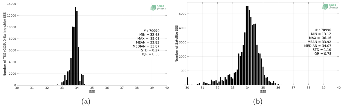
Figure 2: Histograms of SSS from TSG (GOSUD-Sailing-ship) (a) and SMOS SSS L3 v2 - Monthly - 0.25 Deg (CATDS-CECOS-IFREMER) (b) considering all match-up pairs per bins of 0.1 over the Southern Ocean Pi-MEP region and for the full satellite product period.
