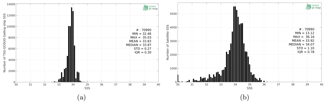
Figure 2: Histograms of SSS from TSG-GOSUD-Sailing-ship (a) and SMOS L3 v2 - Monthly - 0.25 Deg (CATDS-CECOS-IFREMER) (b) considering all match-up pairs per bins of 0.1 over the Southern Ocean Pi-MEP region and for the full satellite product period.
