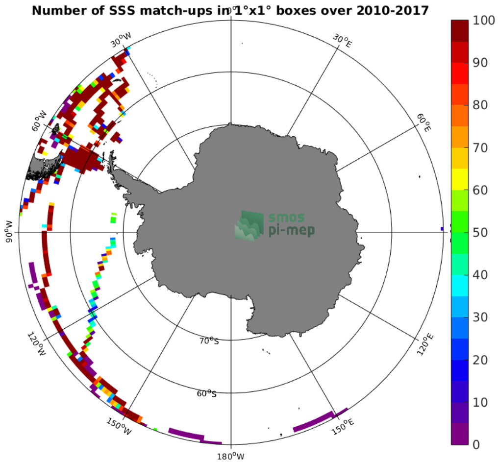
Figure 4: Number of SSS match-ups between TSG-GOSUD-Sailing-ship SSS and the SMOS L3 v2 - Monthly - 0.25 Deg (CATDS-CECOS-IFREMER) SSS product for the Southern Ocean Pi-MEP region over 1^\circ \times 1^\circ boxes and for the full satellite product period.
