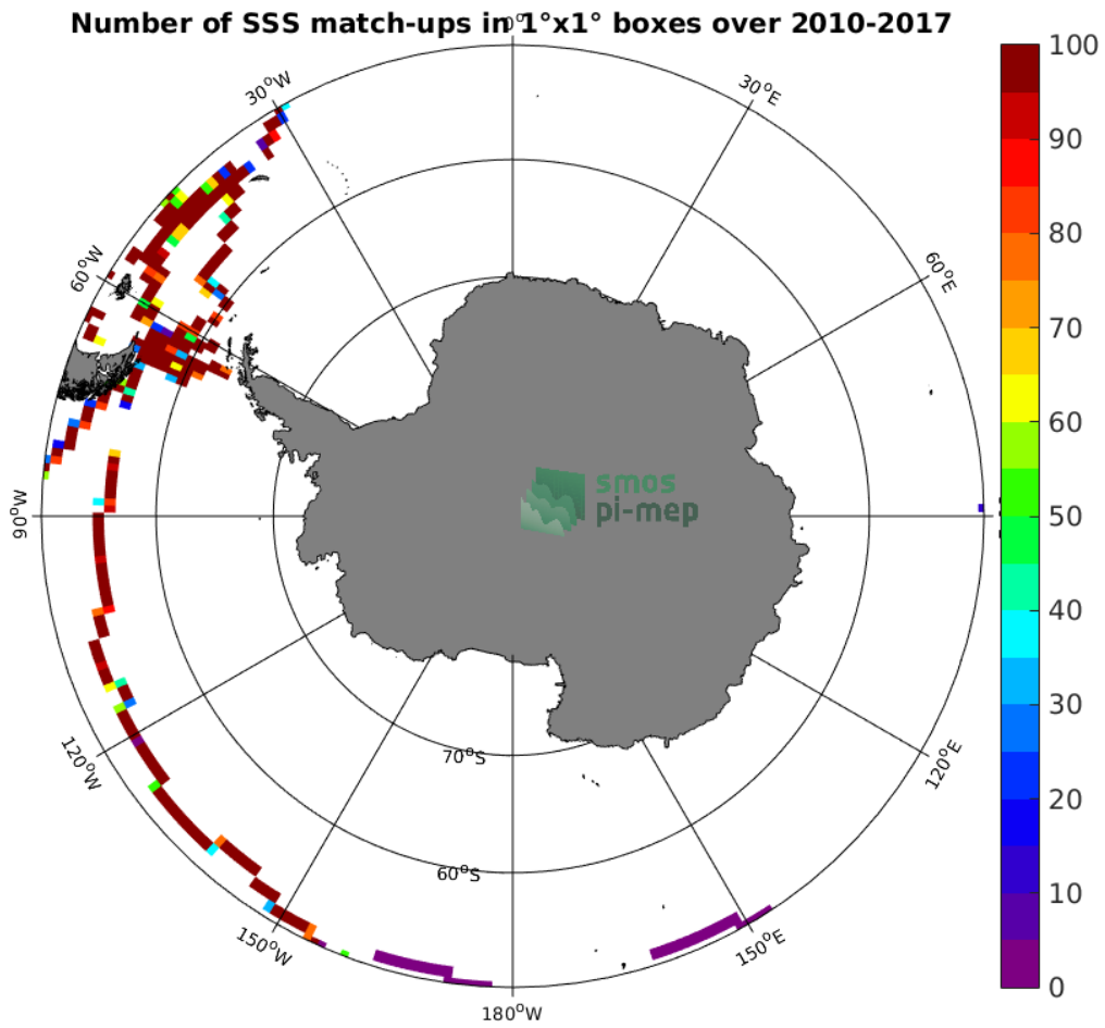
Figure 4: Number of SSS match-ups between TSG-GOSUD-Sailing-ship SSS and the SMOS-L3-CATDS-IFREMER-CECOS-V2-MONTHLY-0.25DEG SSS product for the Southern Ocean Pi-MEP region over 1°x1° boxes and for the full satellite product period.
