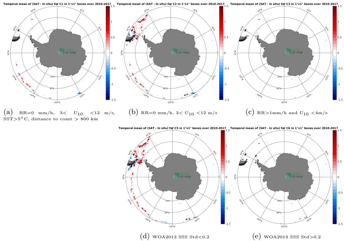
Figure 12: Temporal mean gridded over spatial boxes of size 1^\circ \times 1^\circ of \Delta SSS (SMOS-L3-CATDS-IFREMER-CECOS-V2-MONTHLY-0.25DEG - TSG-GOSUD-Sailing-ship) for 5 different sub-datasets corresponding to:RR=0 mm/h, 3 < U_{10} < 12 m/s, SST >5^\circ C, distance to coast > 800 km (a), RR=0 mm/h, 3 < U_{10} < 12 m/s (b), RR >1 mm/h and U_{10} < 4 m/s (c), WOA2013 SSS Std <0.2 (d), WOA2013 SSS Std >0.2 (e).
