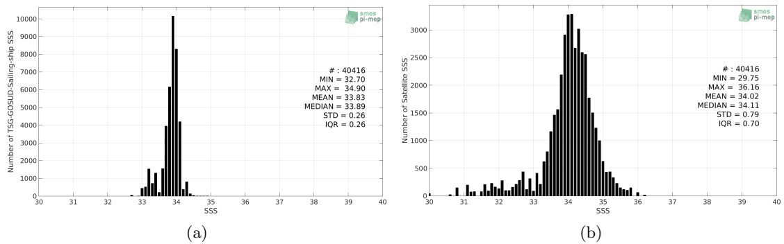
Figure 2: Histograms of SSS from TSG-GOSUD-Sailing-ship (a) and SMOS-L3-CATDS-IFREMER-CECOS-V2-MONTHLY-0.25DEG (b) considering all match-up pairs per bins of 0.1 over the Southern Ocean Pi-MEP region and for the full satellite product period.
