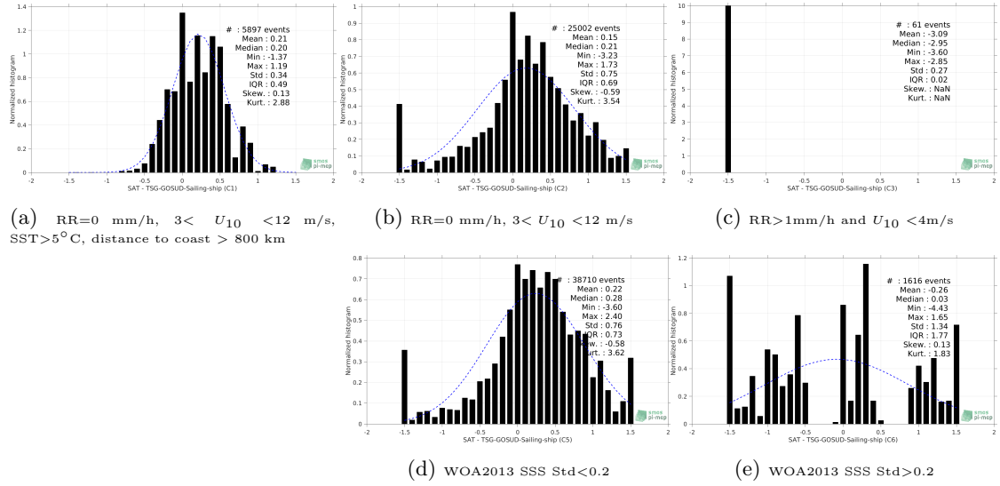
Figure 13: Normalized histogram of \Delta SSS (SMOS-L3-CATDS-IFREMER-CECOS-V2-MONTHLY-0.25DEG - TSG-GOSUD-Sailing-ship) for 5 different subdatasets corresponding to: RR=0 mm/h, 3 < U_{10} < 12 m/s, SST>5°C, distance to coast > 800 km (a), RR=0 mm/h, 3 < U_{10} < 12 m/s (b), RR>1mm/h and U_{10} < 4 m/s (c), WOA2013 SSS Std<0.2 (d), WOA2013 SSS Std>0.2 (e).
