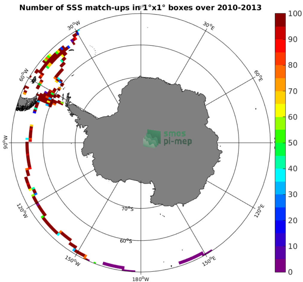
Figure 4: Number of SSS match-ups between TSG-GOSUD-Sailing-ship SSS and the SMOS-L3-CATDS-IFREMER-CECOS-V2-MONTHLY-0.25DEG SSS product for the Southern Ocean Pi-MEP region over 1^\circ \times 1^\circ boxes and for the full satellite product period.
