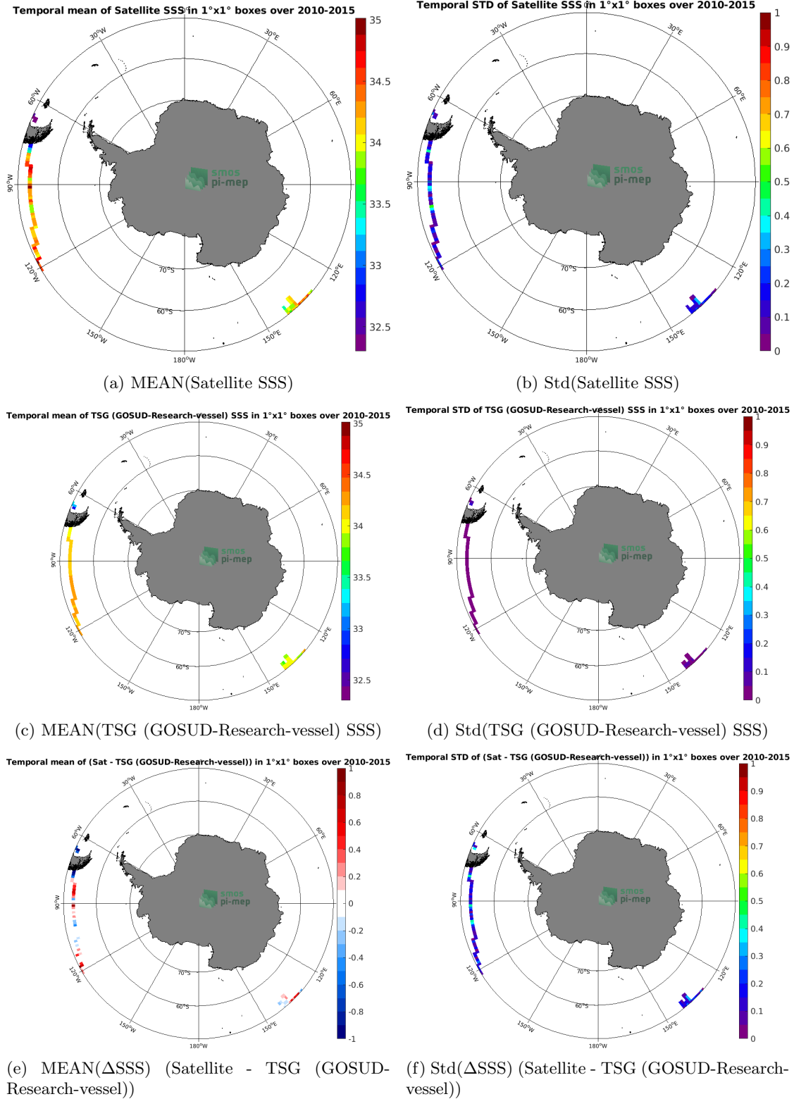
Figure 6: Temporal mean (left) and Std (right) of SSS from SMOS SSS L3 v2 - Monthly - 0.25 Deg (CATDS-CECOS-IFREMER) (top), TSG (GOSUD-Research-vessel) (middle), and of \Delta SSS (Satellite - TSG (GOSUD-Research-vessel)). Only match-up pairs are used to generate these maps.
