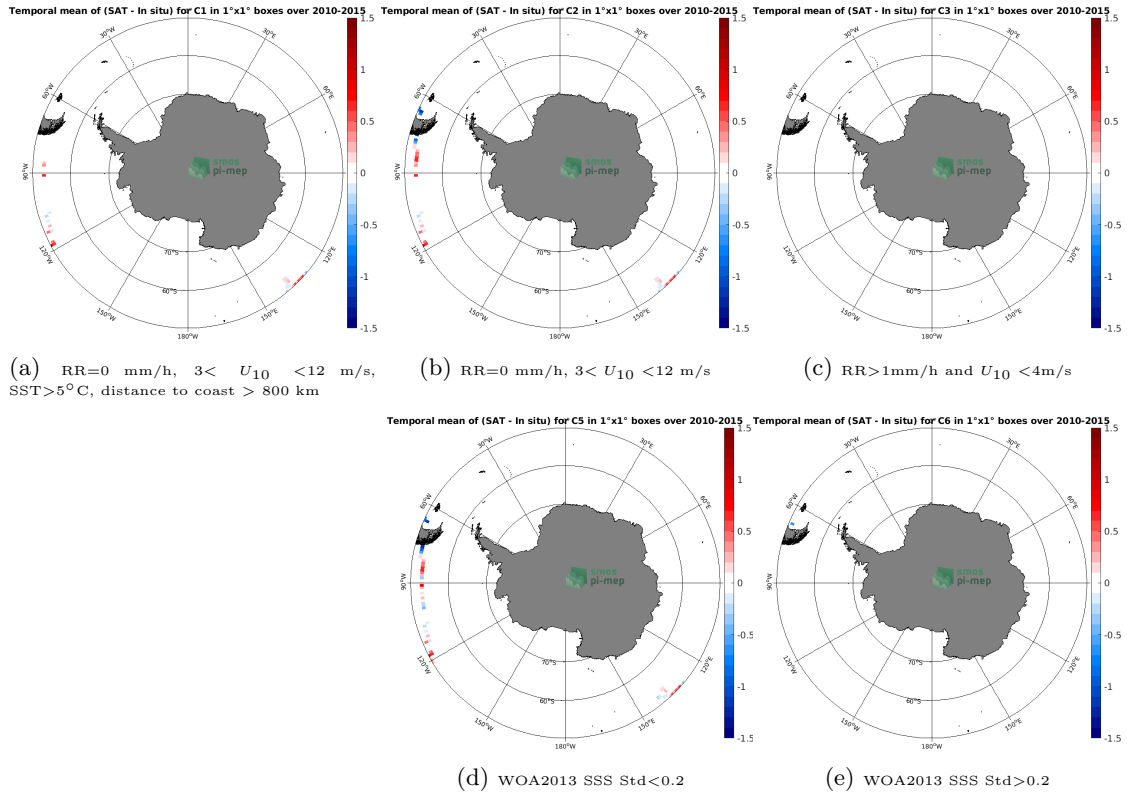
Figure 12: Temporal mean gridded over spatial boxes of size 1°x1° of \Delta SSS (SMOS SSS L3 v2 - Monthly - 0.25 Deg (CATDS-CECOS-IFREMER) - TSG (GOSUD-Research-vessel)) for 5 different subdatasets corresponding to:RR=0 mm/h, 3 < U_{10} < 12 m/s, SST>5°C, distance to coast > 800 km (a), RR=0 mm/h, 3 < U_{10} < 12 m/s (b), RR>1mm/h and U_{10} < 4 m/s (c), WOA2013 SSS Std<0.2 (d), WOA2013 SSS Std>0.2 (e).
