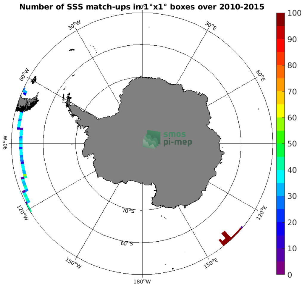
Figure 4: Number of SSS match-ups between TSG (GOSUD-Research-vessel) SSS and the SMOS SSS L3 v2 - Monthly - 0.25 Deg (CATDS-CECOS-IFREMER) SSS product for the Southern Ocean Pi-MEP region over 1^\circ \times 1^\circ boxes and for the full satellite product period.
