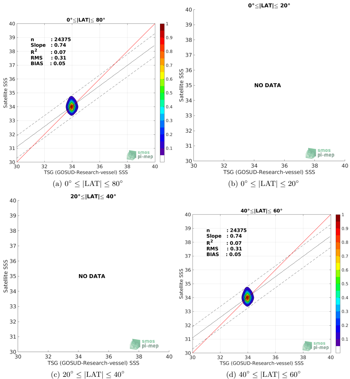
Figure 9: Contour maps of the concentration of SMOS SSS L3 v2 - Monthly - 0.25 Deg (CATDS-CECOS-IFREMER) SSS (y-axis) versus TSG (GOSUD-Research-vessel) SSS (x-axis) at match-up pairs for different latitude bands. For each plot, the red line shows x=y . The black thin and dashed lines indicate a linear fit through the data cloud and the \pm 95\% confidence levels, respectively. The number match-up pairs n , the slope and R^2 coefficient of the linear fit, the root mean square (RMS) and the mean bias between satellite and in situ data are indicated for each latitude band in each plots.
