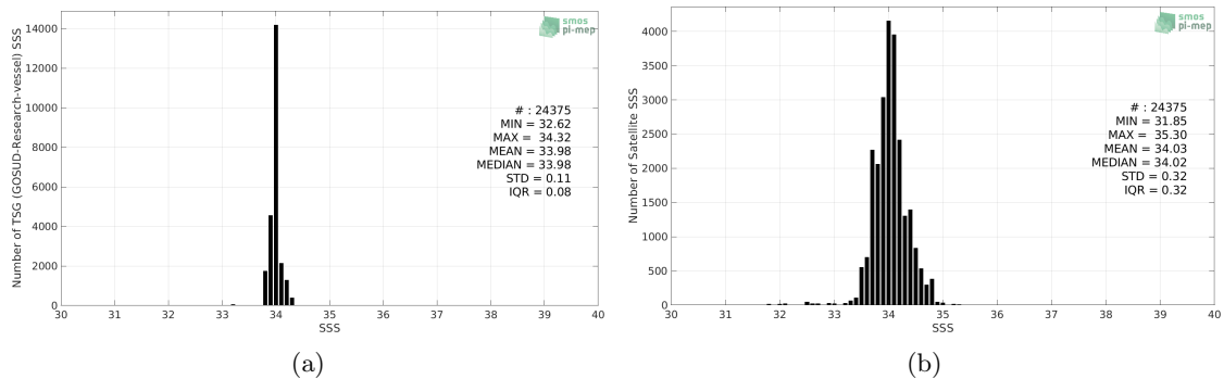
Figure 2: Histograms of SSS from TSG (GOSUD-Research-vessel) (a) and SMOS SSS L3 v2 - Monthly - 0.25 Deg (CATDS-CECOS-IFREMER) (b) considering all match-up pairs per bins of 0.1 over the Southern Ocean Pi-MEP region and for the full satellite product period.
