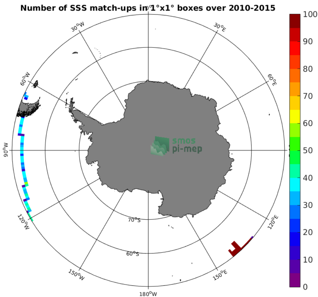
Figure 4: Number of SSS match-ups between TSG (GOSUD-Research-vessel) SSS and the SMOS SSS L3 v2 - Monthly - 0.25 Deg (CATDS-CECOS-IFREMER) SSS product for the Southern Ocean Pi-MEP region over 1°x1° boxes and for the full satellite product period.
