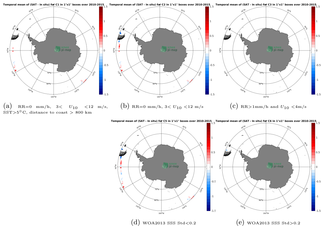
Figure 12: Temporal mean gridded over spatial boxes of size 1^\circ \times 1^\circ of \Delta\text{SSS} (SMOS-L3-CATDS-IFREMER-CECOS-V2-MONTHLY-0.25DEG - TSG-GOSUD-Research-vessel) for 5 different subdatasets corresponding to:RR=0 mm/h, 3 < U_{10} < 12 m/s, SST>5°C, distance to coast > 800 km (a), RR=0 mm/h, 3 < U_{10} < 12 m/s (b), RR>1mm/h and U_{10} < 4 m/s (c), WOA2013 SSS Std<0.2 (d), WOA2013 SSS Std>0.2 (e).
