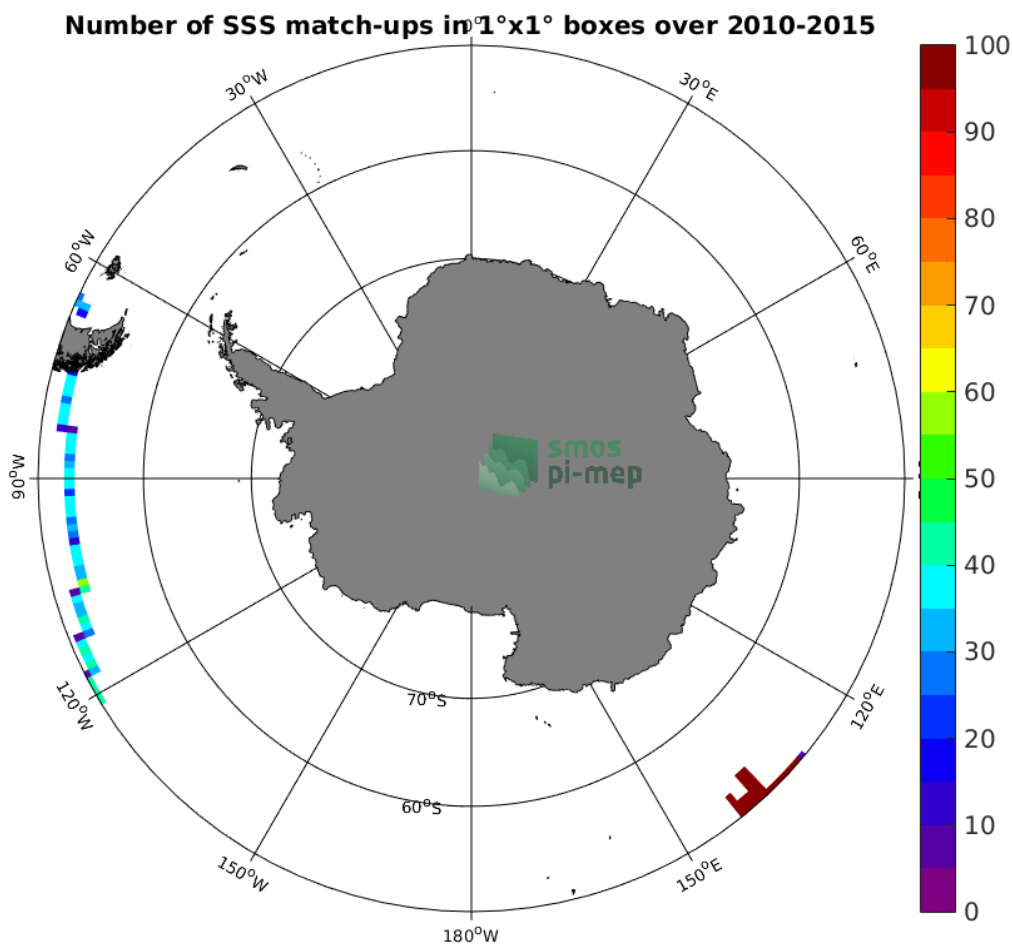
Figure 4: Number of SSS match-ups between TSG-GOSUD-Research-vessel SSS and the SMOS-L3-CATDS-IFREMER-CECOS-V2-MONTHLY-0.25DEG SSS product for the Southern Ocean Pi-MEP region over 1°x1° boxes and for the full satellite product period.
