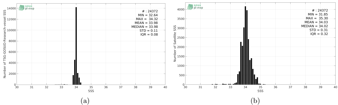
Figure 2: Histograms of SSS from TSG-GOSUD-Research-vessel (a) and SMOS-L3-CATDS-IFREMER-CECOS-V2-MONTHLY-0.25DEG (b) considering all match-up pairs per bins of 0.1 over the Southern Ocean Pi-MEP region and for the full satellite product period.
