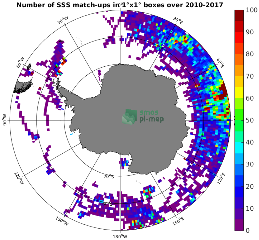
Figure 4: Number of SSS match-ups between Sea mammals SSS and the SMOS-L3-CATDS-IFREMER-CECOS-V2-MONTHLY-0.25DEG SSS product for the Southern Ocean Pi-MEP region over 1°x1° boxes and for the full satellite product period.
