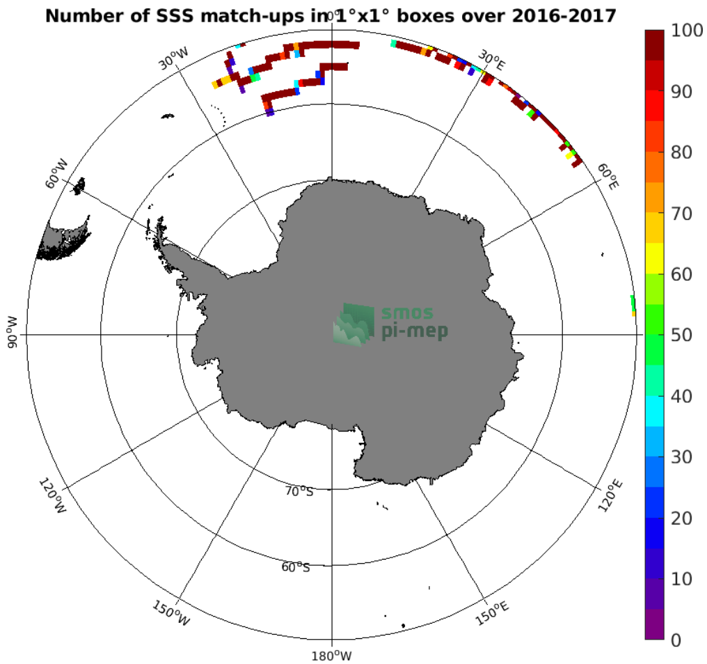
Figure 3: Number of SSS match-ups between Surface drifters SSS and the SMOS SSS L3 v2 - Monthly - 0.25 Deg (CATDS-CECOS-IFREMER) SSS product for the Southern Ocean Pi-MEP region over 1^\circ \times 1^\circ boxes and for the full satellite product period.
