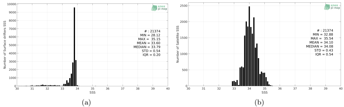
Figure 2: Histograms of SSS from Surface drifters (a) and SMOS SSS L3 v2 - Monthly - 0.25 Deg (CATDS-CECOS-IFREMER) (b) considering all match-up pairs per bins of 0.1 over the Southern Ocean Pi-MEP region and for the full satellite product period.
