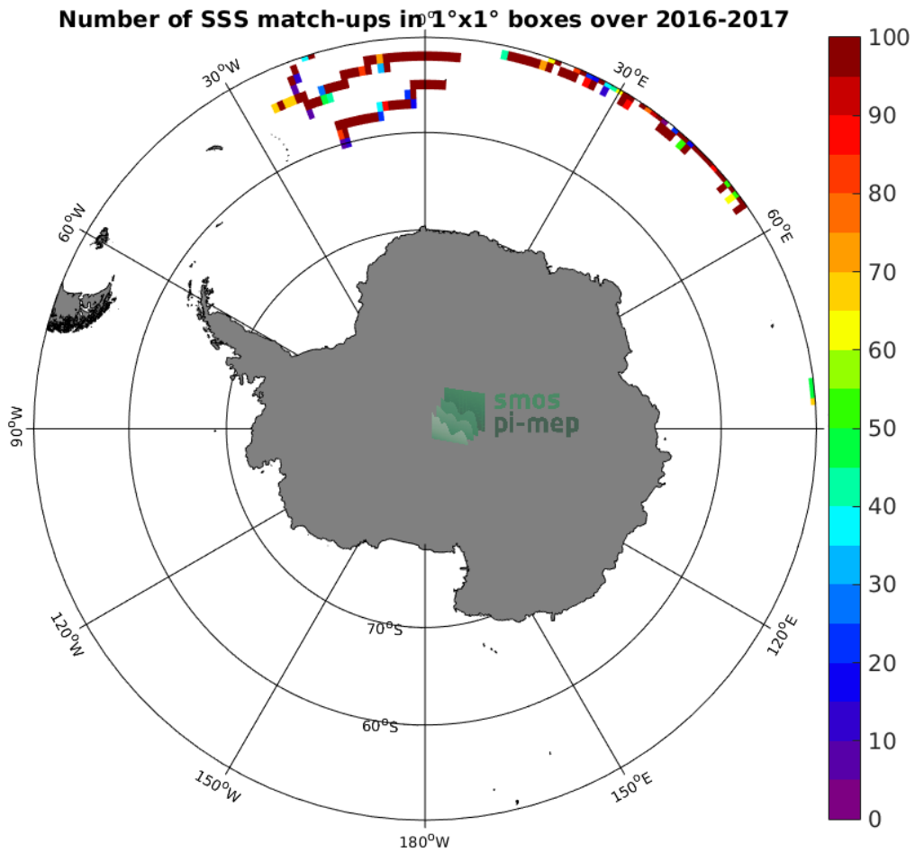
Figure 3: Number of SSS match-ups between Surface drifters SSS and the SMOS L3 v2 - Monthly - 0.25 Deg (CATDS-CECOS-IFREMER) SSS product for the Southern Ocean Pi-MEP region over 1°x1° boxes and for the full satellite product period.
