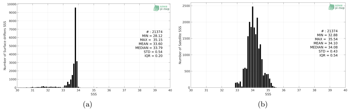
Figure 2: Histograms of SSS from Surface drifters (a) and SMOS L3 v2 - Monthly - 0.25 Deg (CATDS-CECOS-IFREMER) (b) considering all match-up pairs per bins of 0.1 over the Southern Ocean Pi-MEP region and for the full satellite product period.
