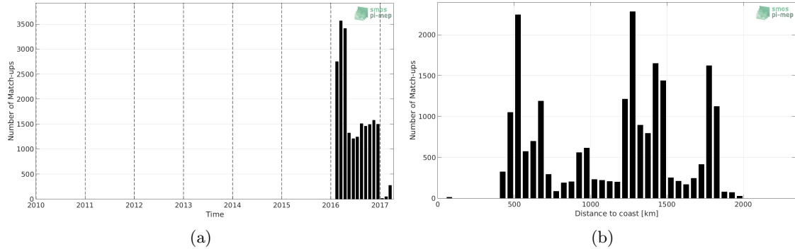
Figure 1: Number of match-ups between Surface drifters and SMOS-L3-CATDS-IFREMER-CECOS-V2-MONTHLY-0.25DEG SSS as a function of time (a) and as function of the distance to coast (b) over the Southern Ocean Pi-MEP region and for the full satellite product period.
