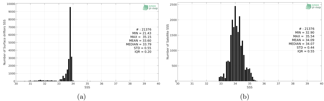
Figure 2: Histograms of SSS from Surface drifters (a) and SMOS-L3-CATDS-IFREMER-CECOS-V2-MONTHLY-0.25DEG (b) considering all match-up pairs per bins of 0.1 over the Southern Ocean Pi-MEP region and for the full satellite product period.
