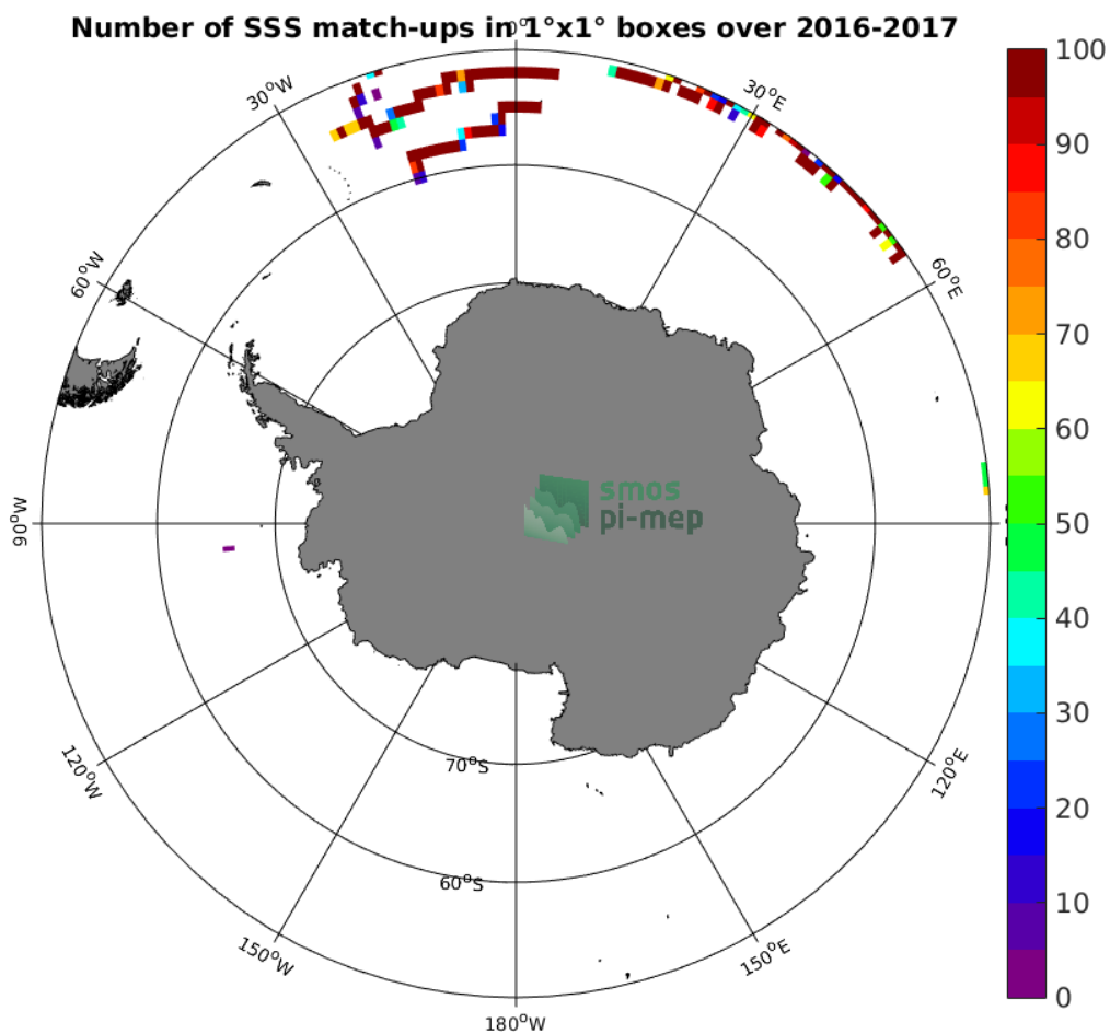
Figure 3: Number of SSS match-ups between Surface drifters SSS and the SMOS-L3-CATDS-IFREMER-CECOS-V2-MONTHLY-0.25DEG SSS product for the Southern Ocean Pi-MEP region over 1^\circ \times 1^\circ boxes and for the full satellite product period.
