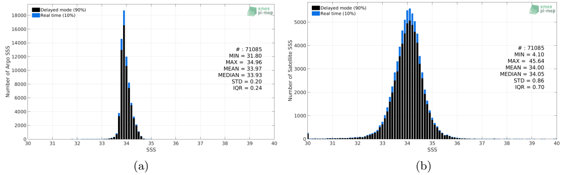
Figure 2: Histograms of SSS from Argo (a) and SMOS SSS L3 v2 - Monthly - 0.25 Deg (CATDS-CECOS-IFREMER) (b) considering all match-up pairs per bins of 0.1 over the Southern Ocean Pi-MEP region and for the full satellite product period.
