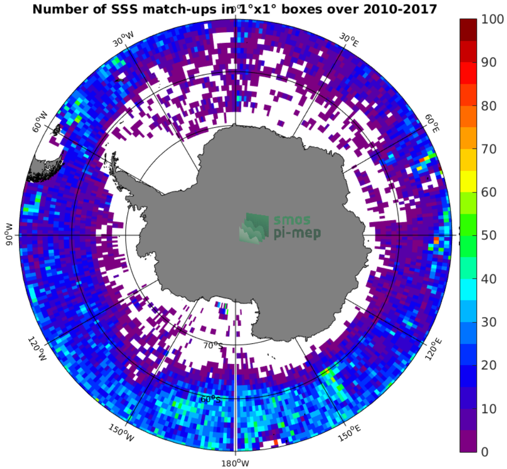
Figure 4: Number of SSS match-ups between Argo SSS and the SMOS SSS L3 v2 - Monthly - 0.25 Deg (CATDS-CECOS-IFREMER) SSS product for the Southern Ocean Pi-MEP region over 1^\circ \times 1^\circ boxes and for the full satellite product period.
