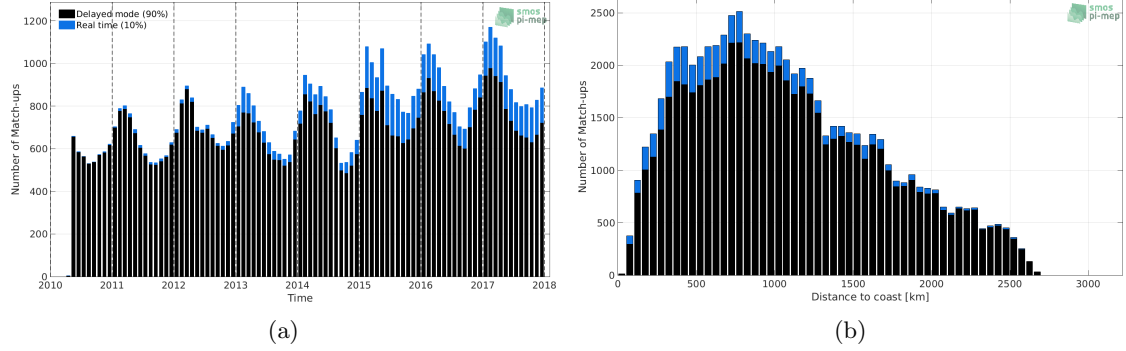
Figure 1: Number of match-ups between Argo and SMOS SSS L3 v2 - Monthly - 0.25 Deg (CATDS-CECOS-IFREMER) SSS as a function of time (a) and as function of the distance to coast (b) over the Southern Ocean Pi-MEP region and for the full satellite product period.
