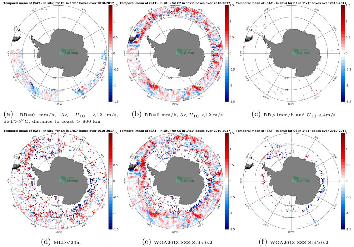
Figure 12: Temporal mean gridded over spatial boxes of size 1^{\circ}\times 1^{\circ} of \Delta\text{SSS} (SMOS SSS L3 v2 - Monthly - 0.25 Deg (CATDS-CECOS-IFREMER) - Argo) for 6 different subdatasets corresponding to: \text{RR}=0 mm/h, 3 < U_{10} < 12 m/s, \text{SST}>5^{\circ}\text{C} , distance to coast > 800 km (a), \text{RR}=0 mm/h, 3 < U_{10} < 12 m/s (b), \text{RR}>1\text{mm/h} and U_{10} < 4\text{m/s} (c), \text{MLD}<20\text{m} (d), \text{WOA2013 SSS Std}<0.2 (e), \text{WOA2013 SSS Std}>0.2 (f).
