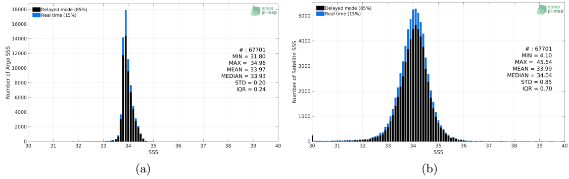
Figure 2: Histograms of SSS from Argo (a) and SMOS L3 v2 - Monthly - 0.25 Deg (CATDS-CECOS-IFREMER) (b) considering all match-up pairs per bins of 0.1 over the Southern Ocean Pi-MEP region and for the full satellite product period.
