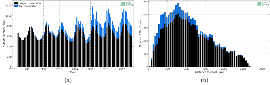
Figure 1: Number of match-ups between Argo and SMOS L3 v2 - Monthly - 0.25 Deg (CATDS-CECOS-IFREMER) SSS as a function of time (a) and as function of the distance to coast (b) over the Southern Ocean Pi-MEP region and for the full satellite product period.
