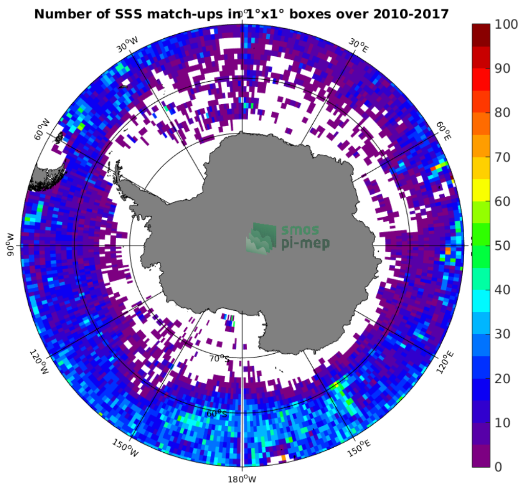
Figure 4: Number of SSS match-ups between Argo SSS and the SMOS L3 v2 - Monthly - 0.25 Deg (CATDS-CECOS-IFREMER) SSS product for the Southern Ocean Pi-MEP region over 1^\circ \times 1^\circ boxes and for the full satellite product period.
