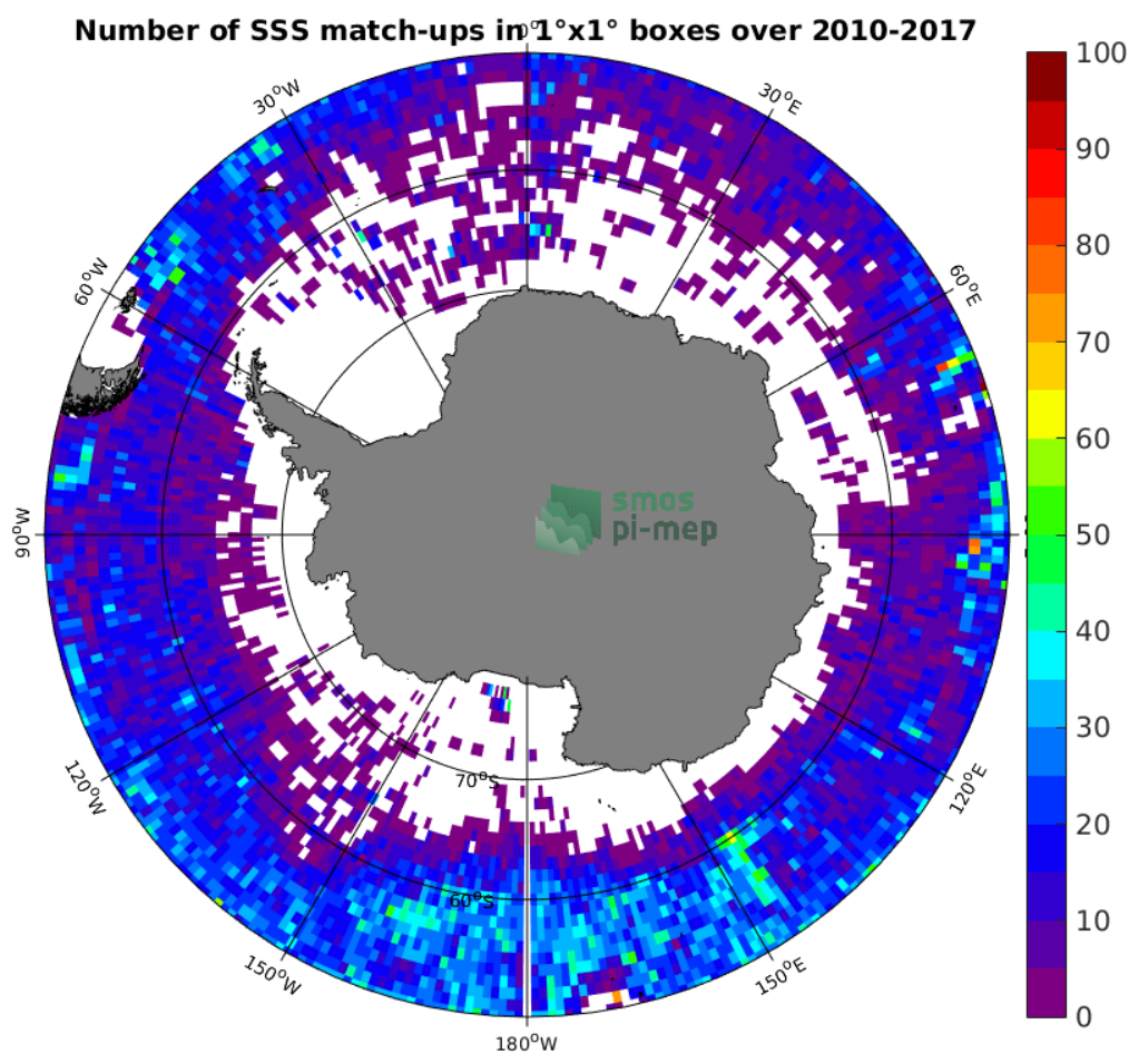
Figure 4: Number of SSS match-ups between Argo SSS and the SMOS-L3-CATDS-IFREMER-CECOS-V2-MONTHLY-0.25DEG SSS product for the Southern Ocean Pi-MEP region over 1^\circ \times 1^\circ boxes and for the full satellite product period.
