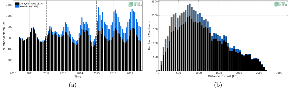
Figure 1: Number of match-ups between Argo and SMOS-L3-CATDS-IFREMER-CECOS-V2-MONTHLY-0.25DEG SSS as a function of time (a) and as function of the distance to coast (b) over the Southern Ocean Pi-MEP region and for the full satellite product period.
