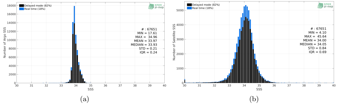
Figure 2: Histograms of SSS from Argo (a) and SMOS-L3-CATDS-IFREMER-CECOS-V2-MONTHLY-0.25DEG (b) considering all match-up pairs per bins of 0.1 over the Southern Ocean Pi-MEP region and for the full satellite product period.
