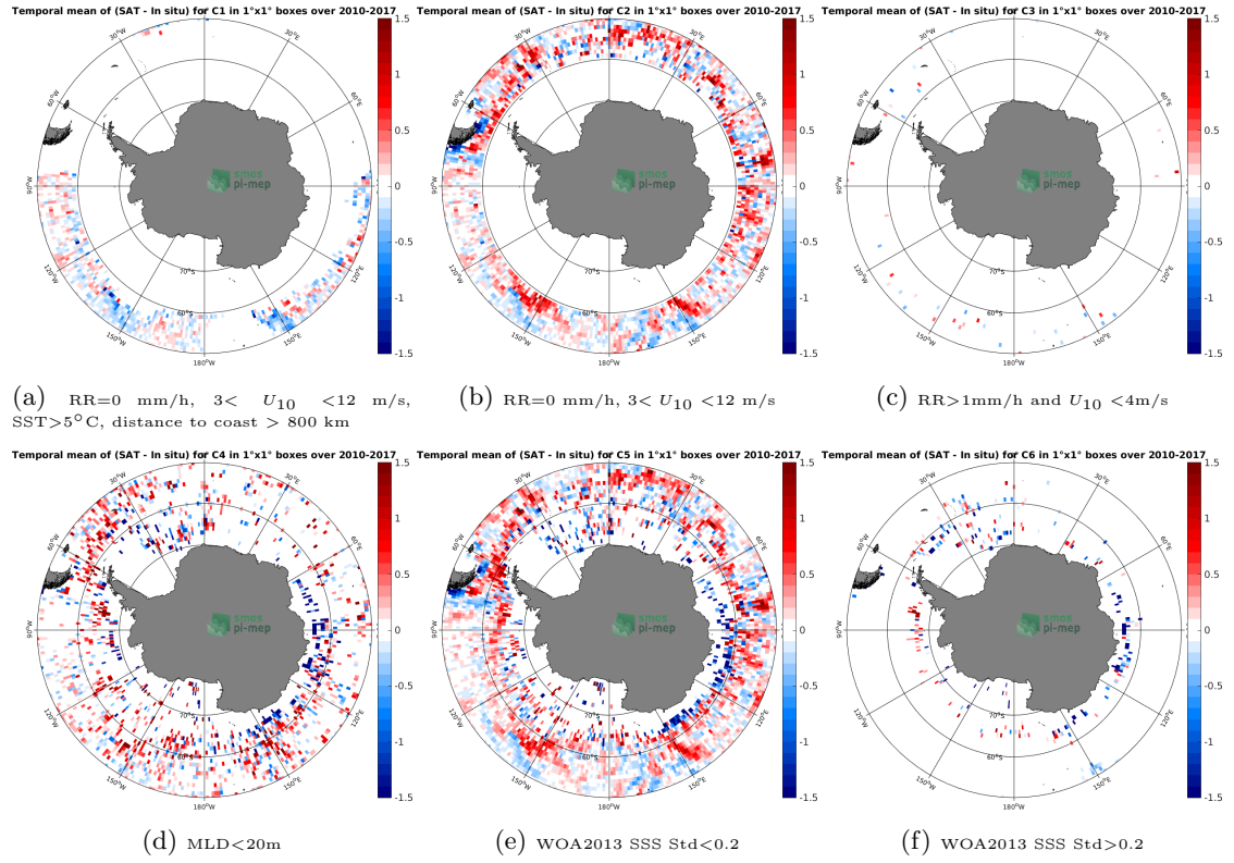
Figure 12: Temporal mean gridded over spatial boxes of size 1^\circ \times 1^\circ of \Delta SSS (SMOS-L3-CATDS-IFREMER-CECOS-V2-MONTHLY-0.25DEG - Argo) for 6 different subdatasets corresponding to: RR=0 mm/h, 3 < U_{10} < 12 m/s, SST >5^\circ C, distance to coast > 800 km (a), RR=0 mm/h, 3 < U_{10} < 12 m/s (b), RR >1 mm/h and U_{10} < 4 m/s (c), MLD <20 m (d), WOA2013 SSS Std <0.2 (e), WOA2013 SSS Std >0.2 (f).
