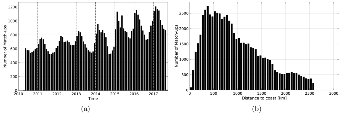
Figure 1: Number of match-ups between Argo and SMOS-L3-CATDS-IFREMER-CECOS-V2-MONTHLY-0.25DEG SSS as a function of time (a) and as function of the distance to coast (b) over the Southern Ocean Pi-MEP region and for the full satellite product period.
