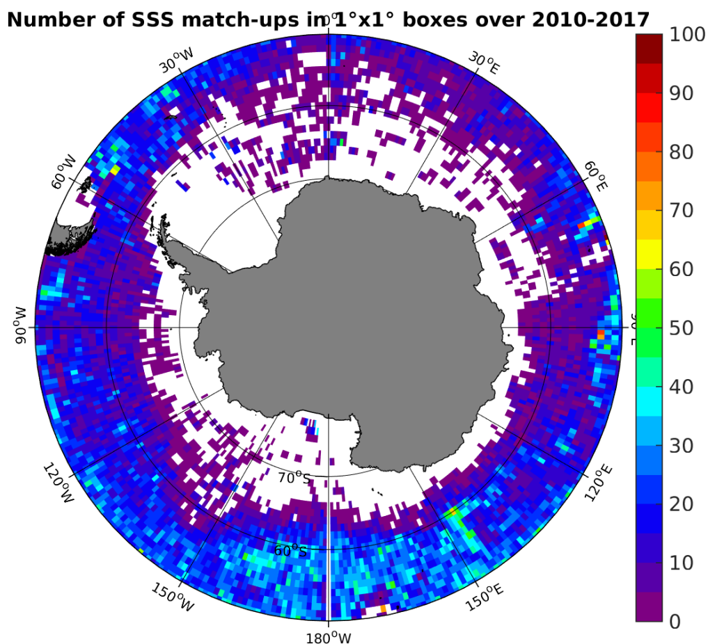
Figure 4: Number of SSS match-ups between Argo SSS and the SMOS-L3-CATDS-IFREMER-CECOS-V2-MONTHLY-0.25DEG SSS product for the Southern Ocean Pi-MEP region over 1^\circ \times 1^\circ boxes and for the full satellite product period.
