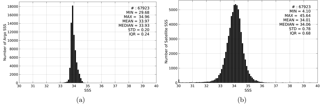
Figure 2: Histograms of SSS from Argo (a) and SMOS-L3-CATDS-IFREMER-CECOS-V2-MONTHLY-0.25DEG (b) considering all match-up pairs per bins of 0.1 over the Southern Ocean Pi-MEP region and for the full satellite product period.
