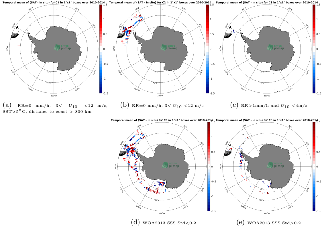
Figure 12: Temporal mean gridded over spatial boxes of size 1^{\circ}\times 1^{\circ} of \Delta\text{SSS} (SMOS SSS L3 v2 - Daily - 0.5 Deg (CATDS-CECOS-IFREMER) - TSG (SAMOS)) for 5 different subdatasets corresponding to: RR=0 mm/h, 3 < U_{10} < 12 m/s, SST > 5^{\circ}\text{C} , distance to coast > 800 km (a), RR=0 mm/h, 3 < U_{10} < 12 m/s (b), RR > 1 mm/h and U_{10} < 4 m/s (c), WOA2013 SSS Std < 0.2 (d), WOA2013 SSS Std > 0.2 (e).
