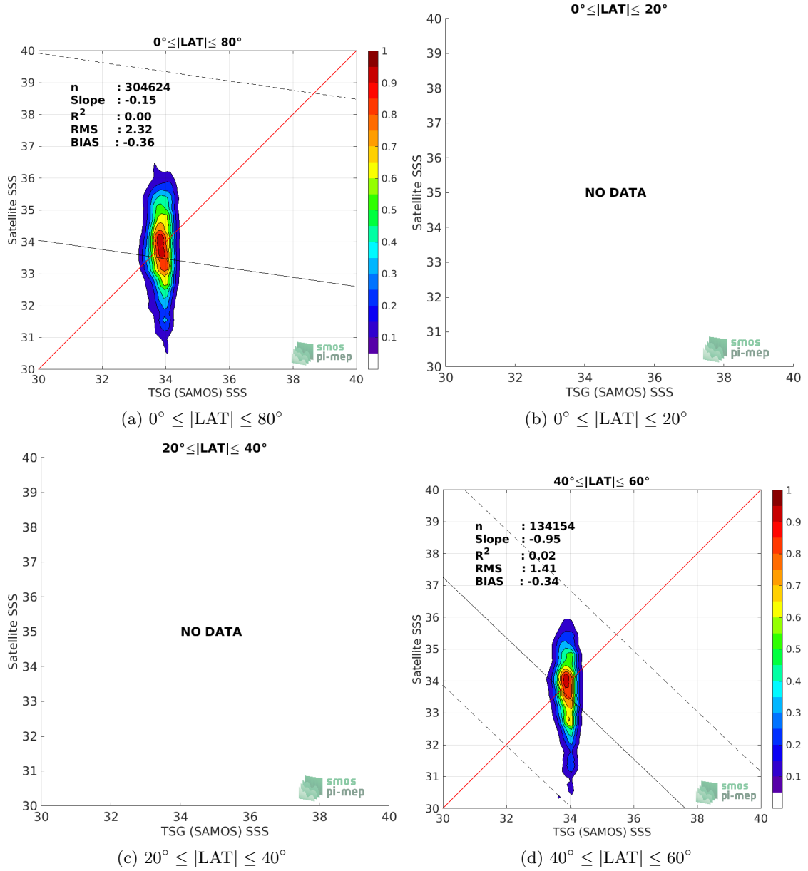
Figure 9: Contour maps of the concentration of SMOS SSS L3 v2 - Daily - 0.5 Deg (CATDS-CECOS-IFREMER) SSS (y-axis) versus TSG (SAMOS) SSS (x-axis) at match-up pairs for different latitude bands. For each plot, the red line shows x=y . The black thin and dashed lines indicate a linear fit through the data cloud and the \pm 95\% confidence levels, respectively. The number match-up pairs n , the slope and R^2 coefficient of the linear fit, the root mean square (RMS) and the mean bias between satellite and in situ data are indicated for each latitude band in each plots.
