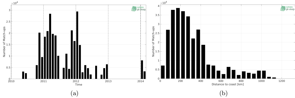
Figure 1: Number of match-ups between TSG (SAMOS) and SMOS SSS L3 v2 - Daily - 0.5 Deg (CATDS-CECOS-IFREMER) SSS as a function of time (a) and as function of the distance to coast (b) over the Southern Ocean Pi-MEP region and for the full satellite product period.
