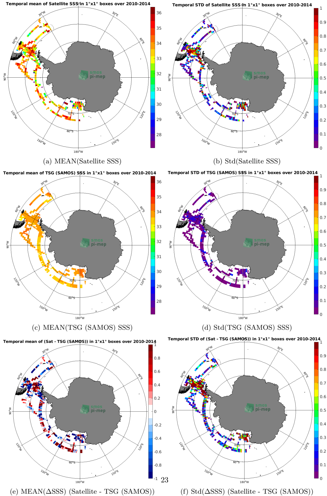
Figure 6: Temporal mean (left) and Std (right) of SSS from SMOS SSS L3 v2 - Daily - 0.5 Deg (CATDS-CECOS-IFREMER) (top), TSG (SAMOS) (middle), and of \Delta SSS (Satellite - TSG (SAMOS)). Only match-up pairs are used to generate these maps.
