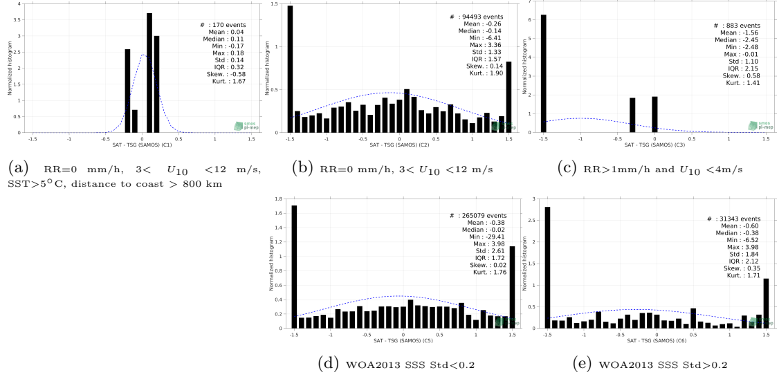
Figure 13: Normalized histogram of \Delta SSS (SMOS SSS L3 v2 - Daily - 0.5 Deg (CATDS-CECOS-IFREMER) - TSG (SAMOS)) for 5 different subdatasets corresponding to: RR=0 mm/h, 3 < U_{10} < 12 m/s, SST>5°C, distance to coast > 800 km (a), RR=0 mm/h, 3 < U_{10} < 12 m/s (b), RR>1mm/h and U_{10} < 4 m/s (c), WOA2013 SSS Std<0.2 (d), WOA2013 SSS Std>0.2 (e).
