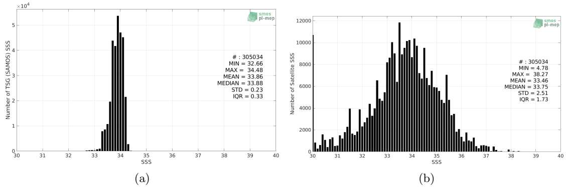
Figure 2: Histograms of SSS from TSG (SAMOS) (a) and SMOS SSS L3 v2 - Daily - 0.5 Deg (CATDS-CECOS-IFREMER) (b) considering all match-up pairs per bins of 0.1 over the Southern Ocean Pi-MEP region and for the full satellite product period.
