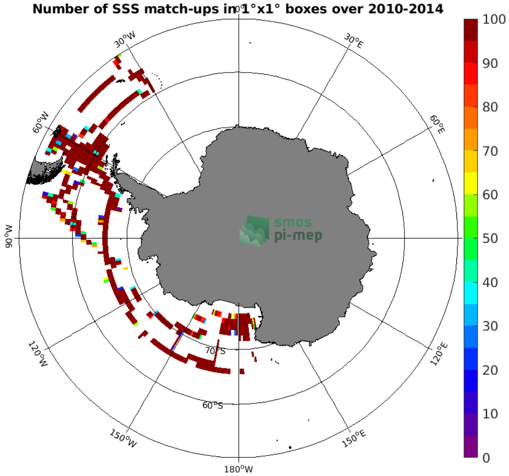
Figure 4: Number of SSS match-ups between TSG (SAMOS) SSS and the SMOS SSS L3 v2 - Daily - 0.5 Deg (CATDS-CECOS-IFREMER) SSS product for the Southern Ocean Pi-MEP region over 1^\circ \times 1^\circ boxes and for the full satellite product period.
