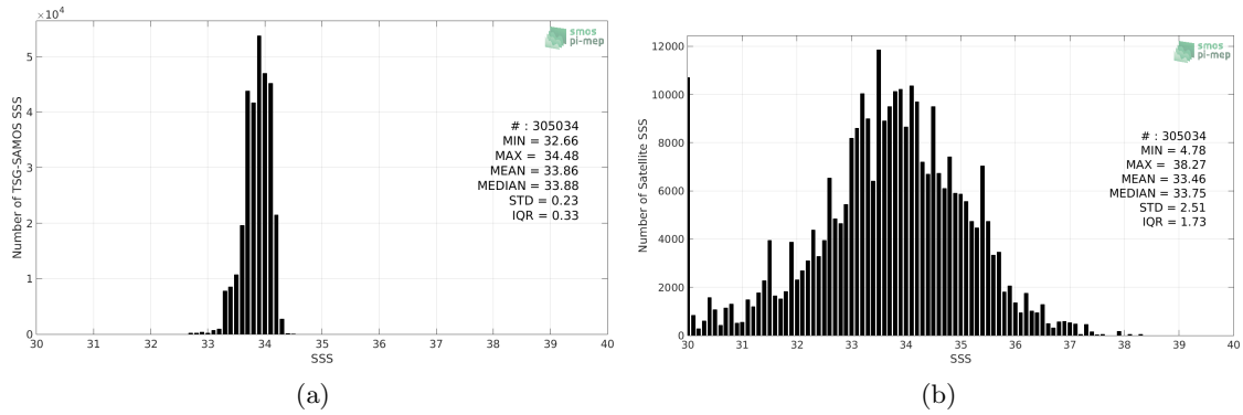
Figure 2: Histograms of SSS from TSG-SAMOS (a) and SMOS L3 v2 - Daily - 0.5 Deg (CATDS-CECOS-IFREMER) (b) considering all match-up pairs per bins of 0.1 over the Southern Ocean Pi-MEP region and for the full satellite product period.
