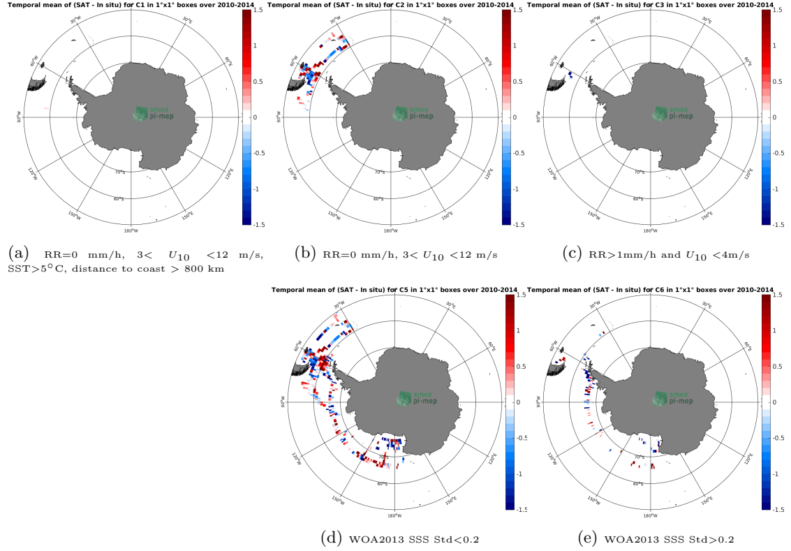
Figure 12: Temporal mean gridded over spatial boxes of size 1^{\circ}\times 1^{\circ} of \Delta\text{SSS} (SMOS L3 v2 - Daily - 0.5 Deg (CATDS-CECOS-IFREMER) - TSG-SAMOS) for 5 different subdatasets corresponding to: \text{RR}=0 mm/h, 3 < U_{10} < 12 m/s, \text{SST}>5^{\circ}\text{C} , distance to coast > 800 km (a), \text{RR}=0 mm/h, 3 < U_{10} < 12 m/s (b), \text{RR}>1 mm/h and U_{10} < 4 m/s (c), WOA2013 SSS Std <0.2 (d), WOA2013 SSS Std >0.2 (e).
