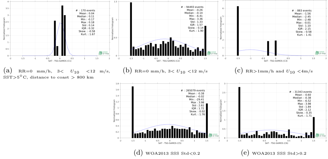
Figure 13: Normalized histogram of \Delta SSS (SMOS L3 v2 - Daily - 0.5 Deg (CATDS-CECOS-IFREMER) - TSG-SAMOS) for 5 different subdatasets corresponding to: RR=0 mm/h, 3 < U_{10} < 12 m/s, SST>5°C, distance to coast > 800 km (a), RR=0 mm/h, 3 < U_{10} < 12 m/s (b), RR>1 mm/h and U_{10} < 4 m/s (c), WOA2013 SSS Std<0.2 (d), WOA2013 SSS Std>0.2 (e).
