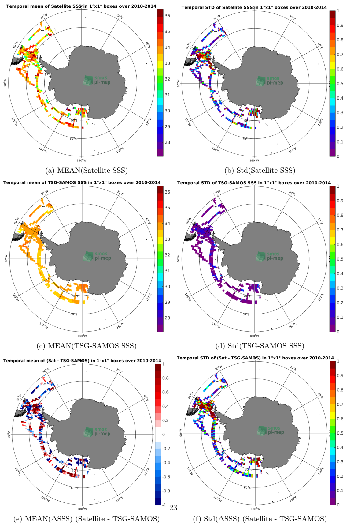
Figure 6: Temporal mean (left) and Std (right) of SSS from SMOS L3 v2 - Daily - 0.5 Deg (CATDS-CECOS-IFREMER) (top), TSG-SAMOS (middle), and of \Delta SSS (Satellite - TSG-SAMOS). Only match-up pairs are used to generate these maps.
