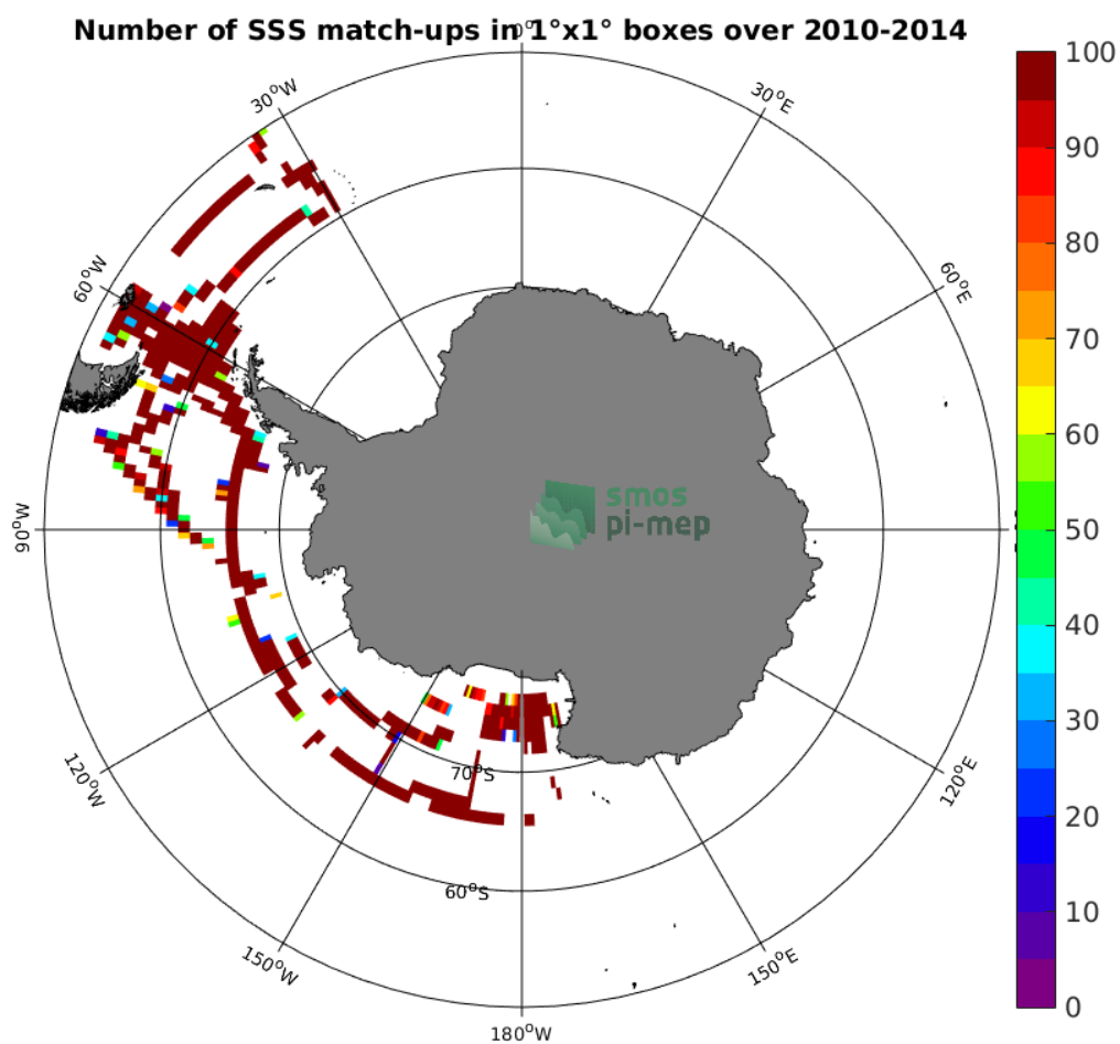
Figure 4: Number of SSS match-ups between TSG-SAMOS SSS and the SMOS L3 v2 - Daily - 0.5 Deg (CATDS-CECOS-IFREMER) SSS product for the Southern Ocean Pi-MEP region over 1^\circ \times 1^\circ boxes and for the full satellite product period.
