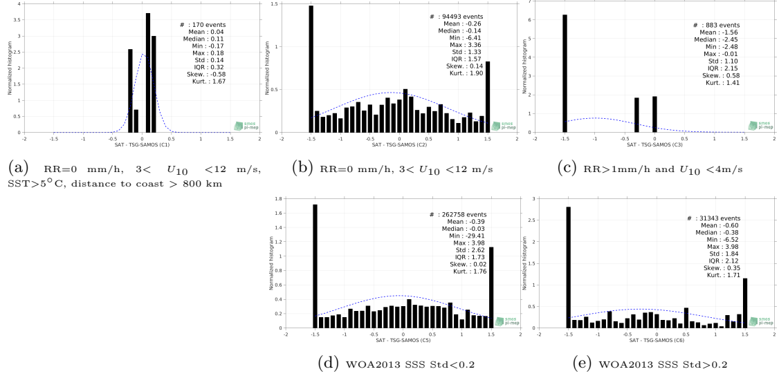
Figure 13: Normalized histogram of \Delta SSS (SMOS-L3-CATDS-CECOS-IFREMER-V2-1DAY-0.5DEG - TSG-SAMOS) for 5 different subdatasets corresponding to: RR=0 mm/h, 3 < U_{10} < 12 m/s, SST>5°C, distance to coast > 800 km (a), RR=0 mm/h, 3 < U_{10} < 12 m/s (b), RR>1mm/h and U_{10} < 4 m/s (c), WOA2013 SSS Std<0.2 (d), WOA2013 SSS Std>0.2 (e).
