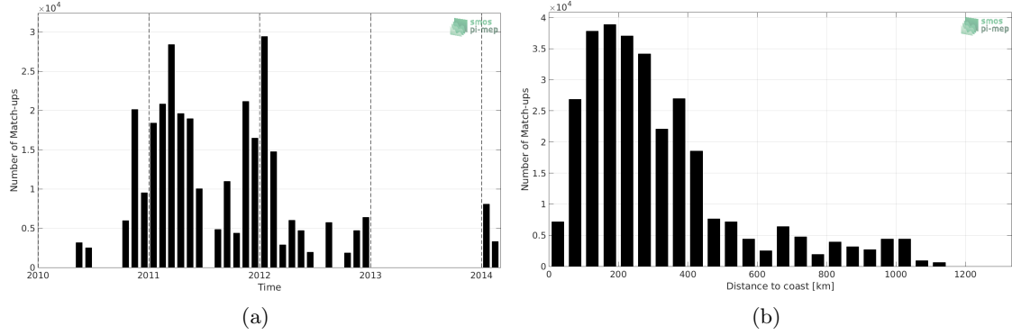
Figure 1: Number of match-ups between TSG-SAMOS and SMOS-L3-CATDS-CECOS-IFREMER-V2-1DAY-0.5DEG SSS as a function of time (a) and as function of the distance to coast (b) over the Southern Ocean Pi-MEP region and for the full satellite product period.
