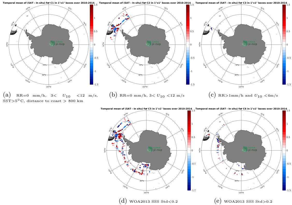
Figure 12: Temporal mean gridded over spatial boxes of size 1^\circ \times 1^\circ of \Delta SSS (SMOS-L3-CATDS-CECOS-IFREMER-V2-1DAY-0.5DEG - TSG-SAMOS) for 5 different subdatasets corresponding to: RR=0 mm/h, 3 < U_{10} < 12 m/s, SST > 5^\circ C , distance to coast > 800 km (a), RR=0 mm/h, 3 < U_{10} < 12 m/s (b), RR > 1 mm/h and U_{10} < 4 m/s (c), WOA2013 SSS Std < 0.2 (d), WOA2013 SSS Std > 0.2 (e).
