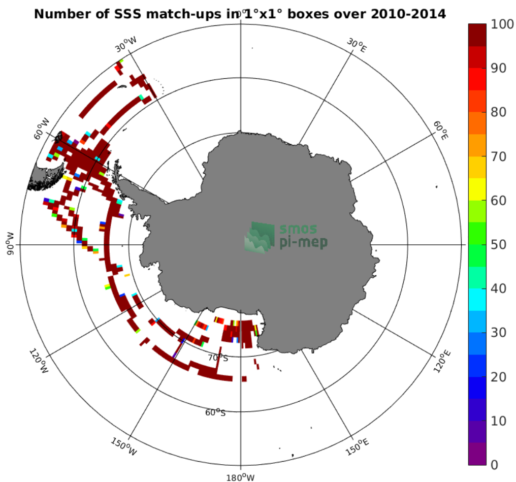
Figure 4: Number of SSS match-ups between TSG-SAMOS SSS and the SMOS-L3-CATDS-CECOS-IFREMER-V2-1DAY-0.5DEG SSS product for the Southern Ocean Pi-MEP region over 1^\circ \times 1^\circ boxes and for the full satellite product period.
