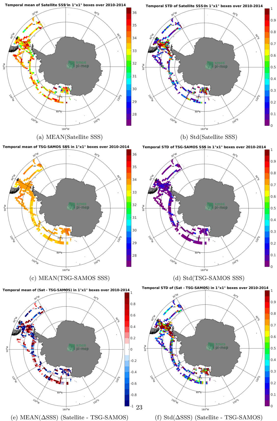
Figure 6: Temporal mean (left) and Std (right) of SSS from SMOS-L3-CATDS-CECOS-IFREMER-V2-1DAY-0.5DEG (top), TSG-SAMOS (middle), and of \Delta SSS (Satellite - TSG-SAMOS). Only match-up pairs are used to generate these maps.
