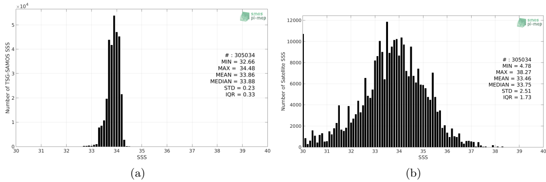
Figure 2: Histograms of SSS from TSG-SAMOS (a) and SMOS-L3-CATDS-CECOS-IFREMER-V2-1DAY-0.5DEG (b) considering all match-up pairs per bins of 0.1 over the Southern Ocean Pi-MEP region and for the full satellite product period.
