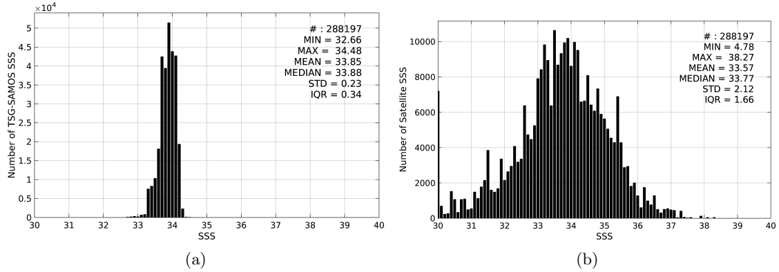
Figure 2: Histograms of SSS from TSG-SAMOS (a) and SMOS-L3-CATDS-CECOS-IFREMER-V2-1DAY-0.5deg (b) considering all match-up pairs per bins of 0.1 over the Southern Ocean Pi-MEP region and for the full satellite product period.
