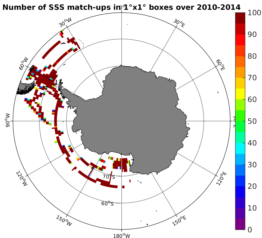
Figure 4: Number of SSS match-ups between TSG-SAMOS SSS and the SMOS-L3-CATDS-CECOS-IFREMER-V2-1DAY-0.5deg SSS product for the Southern Ocean Pi-MEP region over 1^\circ \times 1^\circ boxes and for the full satellite product period.
