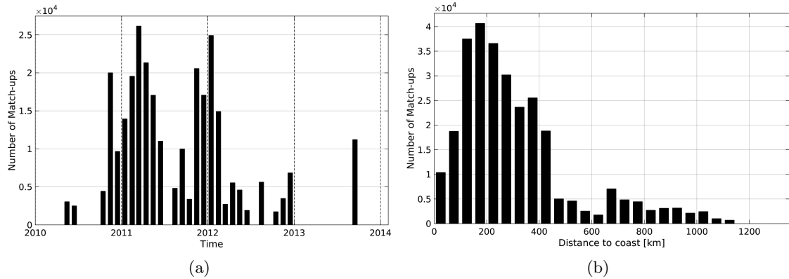
Figure 1: Number of match-ups between TSG-SAMOS and SMOS-L3-CATDS-CECOS-IFREMER-V2-1DAY-0.5deg SSS as a function of time (a) and as function of the distance to coast (b) over the Southern Ocean Pi-MEP region and for the full satellite product period.
