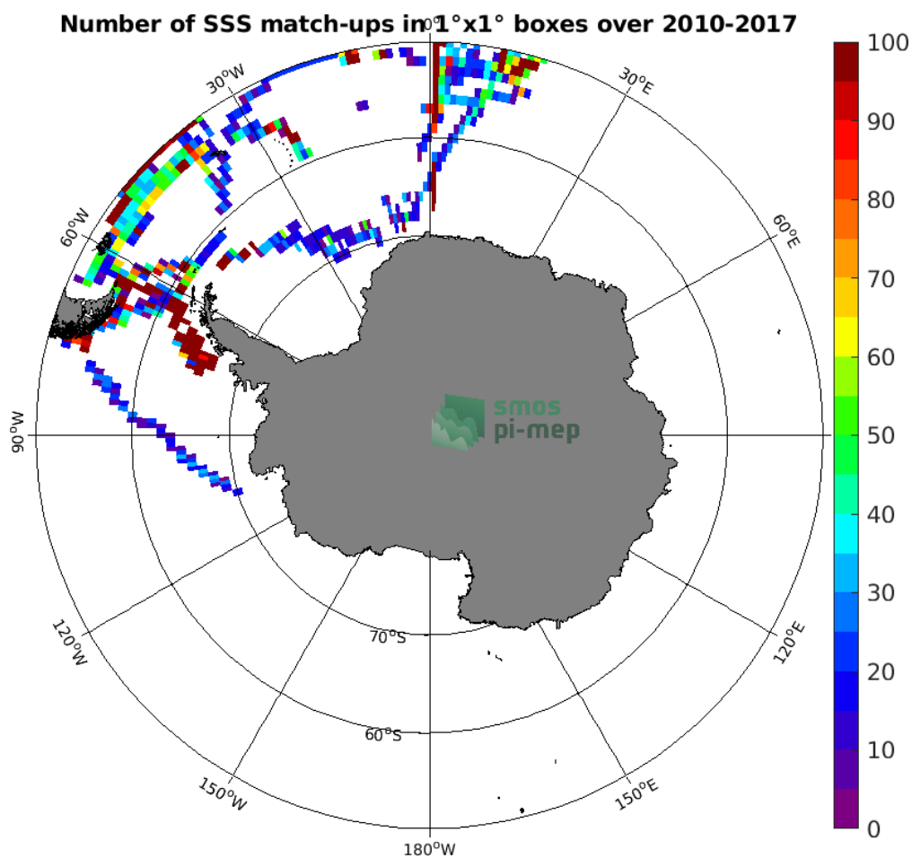
Figure 4: Number of SSS match-ups between TSG (Polarstern) SSS and the SMOS SSS L3 v2 - Daily - 0.5 Deg (CATDS-CECOS-IFREMER) SSS product for the Southern Ocean Pi-MEP region over 1^\circ \times 1^\circ boxes and for the full satellite product period.
