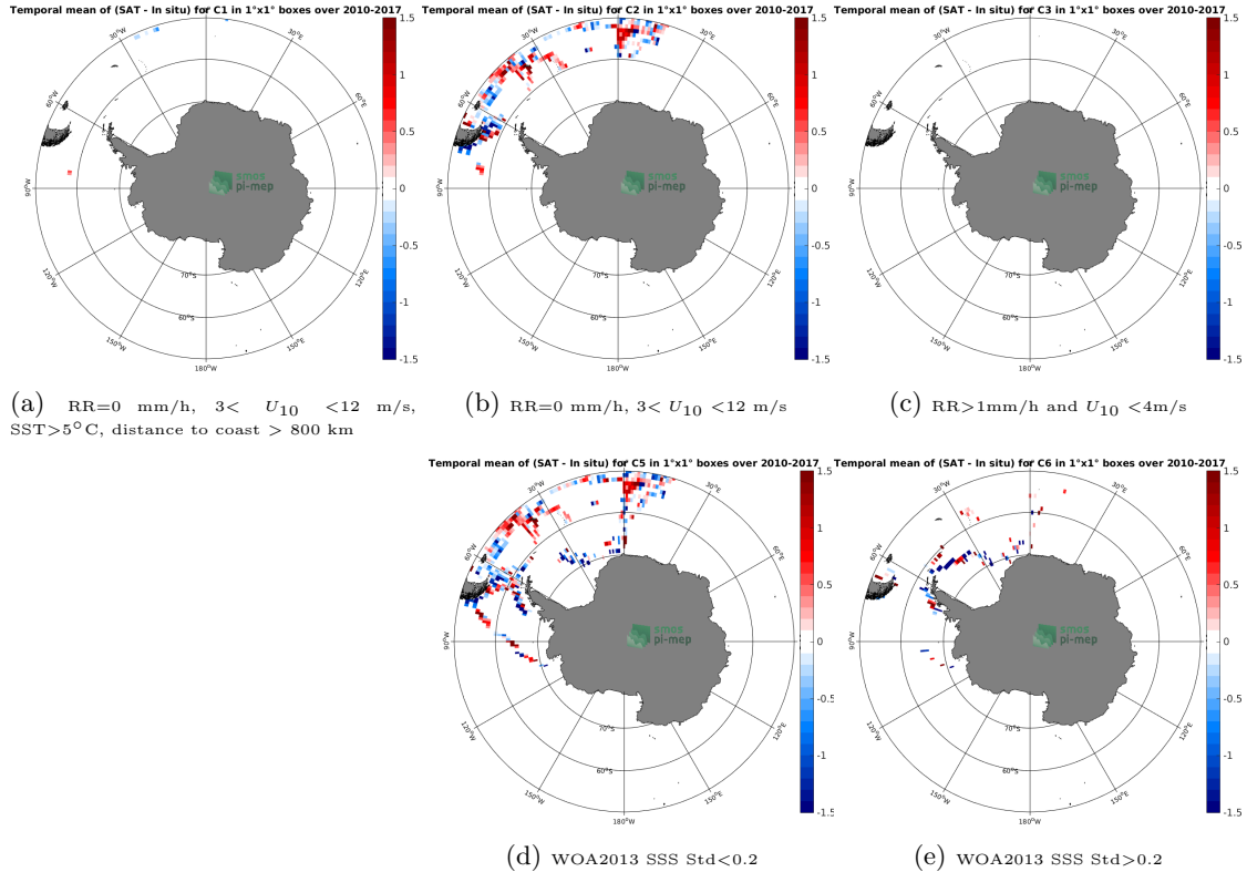
Figure 12: Temporal mean gridded over spatial boxes of size 1^{\circ}\times 1^{\circ} of \Delta\text{SSS} (SMOS SSS L3 v2 - Daily - 0.5 Deg (CATDS-CECOS-IFREMER) - TSG (Polarstern)) for 5 different subdatasets corresponding to:RR=0 mm/h, 3 < U_{10} < 12 m/s, SST >5^{\circ}\text{C} , distance to coast > 800 km (a), RR=0 mm/h, 3 < U_{10} < 12 m/s (b), RR >1 mm/h and U_{10} < 4 m/s (c), WOA2013 SSS Std <0.2 (d), WOA2013 SSS Std >0.2 (e).
