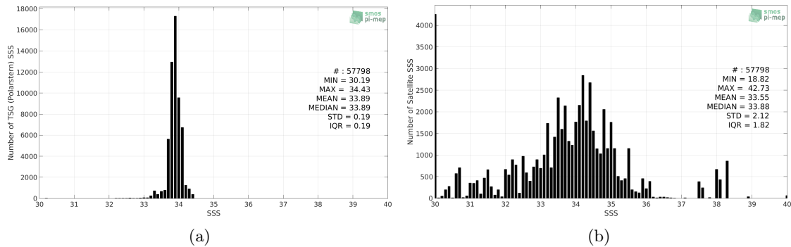
Figure 2: Histograms of SSS from TSG (Polarstern) (a) and SMOS SSS L3 v2 - Daily - 0.5 Deg (CATDS-CECOS-IFREMER) (b) considering all match-up pairs per bins of 0.1 over the Southern Ocean Pi-MEP region and for the full satellite product period.
