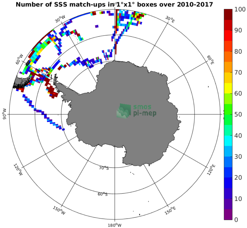
Figure 4: Number of SSS match-ups between TSG (Polarstern) SSS and the SMOS SSS L3 v2 - Daily - 0.5 Deg (CATDS-CECOS-IFREMER) SSS product for the Southern Ocean Pi-MEP region over 1°x1° boxes and for the full satellite product period.
