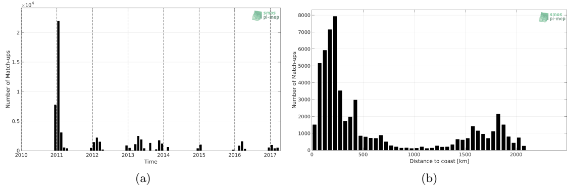
Figure 1: Number of match-ups between TSG (Polarstern) and SMOS SSS L3 v2 - Daily - 0.5 Deg (CATDS-CECOS-IFREMER) SSS as a function of time (a) and as function of the distance to coast (b) over the Southern Ocean Pi-MEP region and for the full satellite product period.
